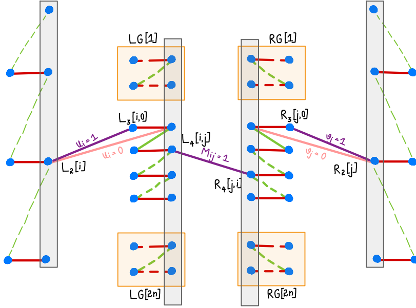
Figure 6.3: Reduction graph for the expander matching lower bound. It is similar to Figure 6.2, except for the changes due to increasing the dimension, the pink edges when the input is 0, and the grey region which denote the expander edges.
