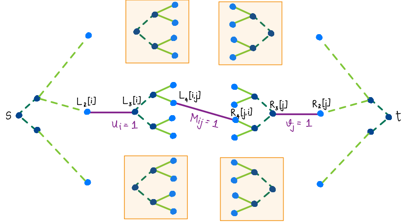
Figure 6.4.: Reduction graph for the (s, t) -shortest path lower bound. The dark green edges denote the internal forest edges, the light green edges denote the leaf edges, and the purple edges denote the input-dependent edges.
