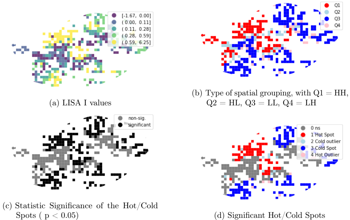
Figure 4.8: LISA Maps
