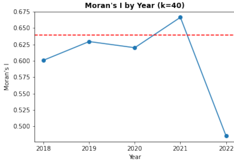
Figure 4.7: Moran's I 2018 - 2022
