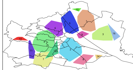
Figure 7.1: MDSTC-DBSCAN results
