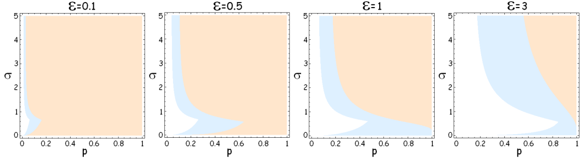
FIG. 3: (Colour online) Detection quality of the inequality (*) for the family of the tripartite states (8) with \Delta = 1, \delta = 1 and x_0 = \{0, 1.5\} (where x_0 = 0 detects better if \sigma < 1 , even for very small p , but ceases to detect for large \epsilon ; and x_0 = 1.5 detects better for \sigma > 1 and still detects a considerable amount of entanglement for large \epsilon ). The red area is detected to be genuinely multipartite entangled (2-inseparable) and the blue and red areas are detected to be entangled (3-inseparable).
