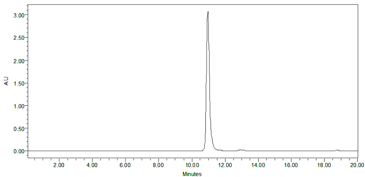
Fig. 24 CP20 100 \mu M in buffer from uptake assay, 50 \mu l injection volume, retention time: 10.962 minutes
