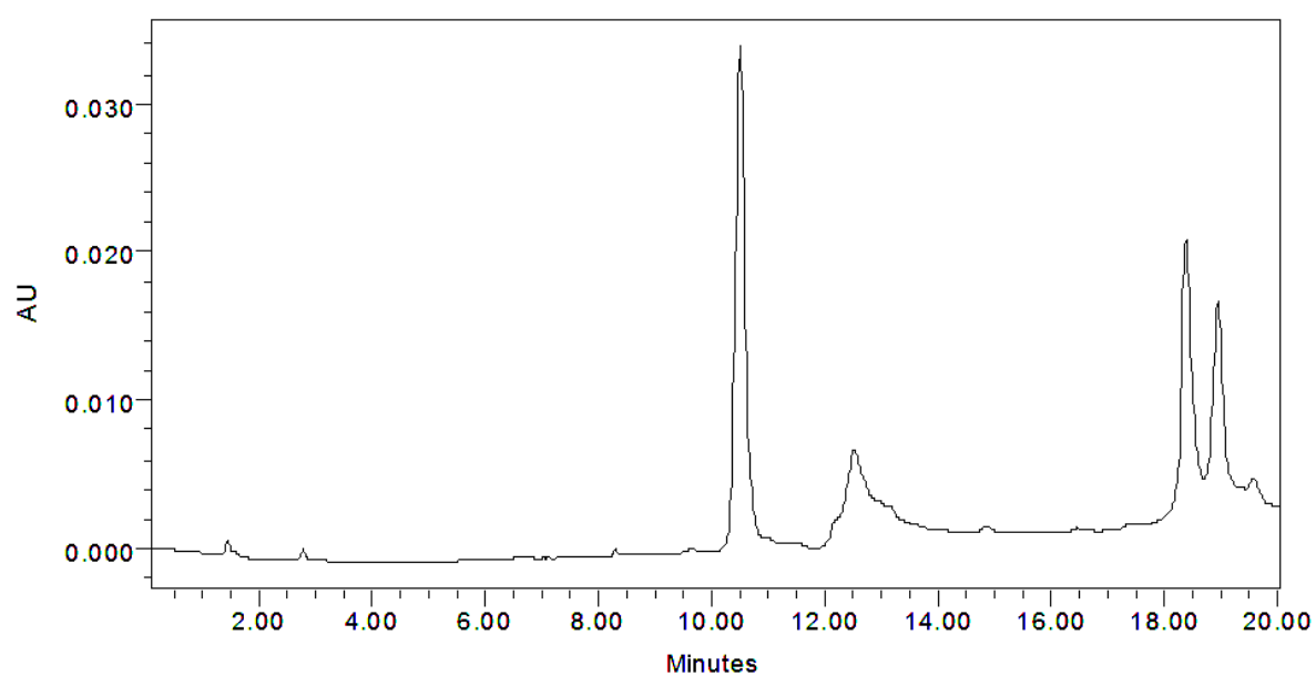
Fig. 48 CP20 20 μM in water, 50 μl injection volume
