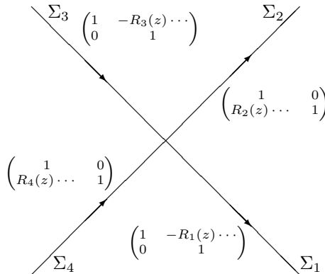
Figure A.1: Contours of a cross
