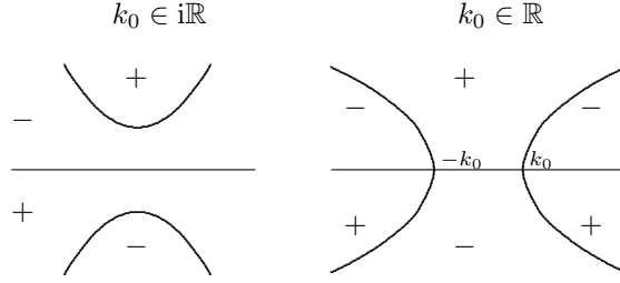
Figure 3.1: Sign of \text{Re}(\Phi(k)) for different values of k_0
