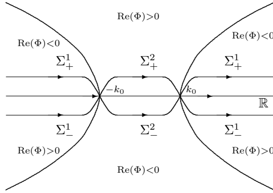
Figure 3.3: Deformed contour for k_0 \in \mathbb{R}^+
