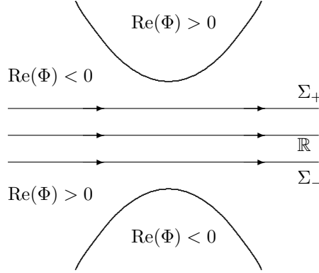
Figure 3.2: Deformed contour for k_0 \in i\mathbb{R}^+
