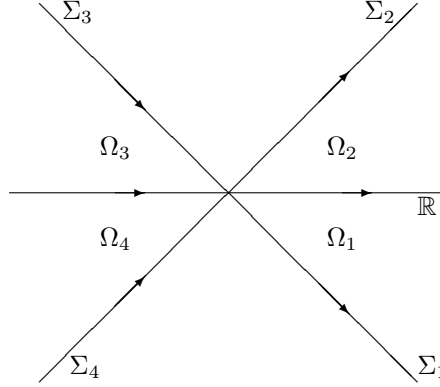
Figure A.2: Deforming back the cross
