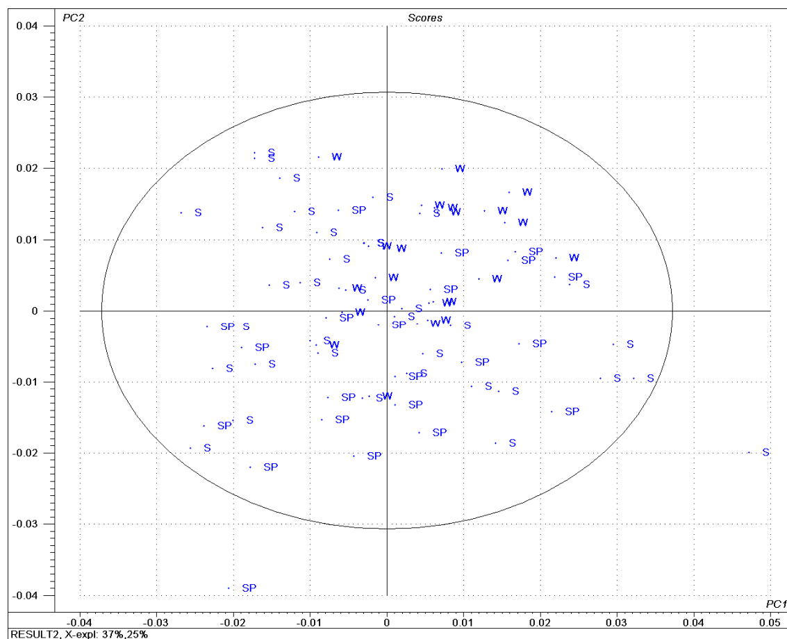
Fig. 27: Scores plot (PC1 (37%) vs. PC2 (25%)) of R. repens chloroform extracts. Spring (SP), summer (S), winter (W).
