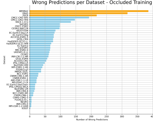
Figure 15: Example for one of the conducted experiments. Prediction of CNN classifier trained on 20% fraction occluded data. Wrong predictions are biased towards the OBS.
