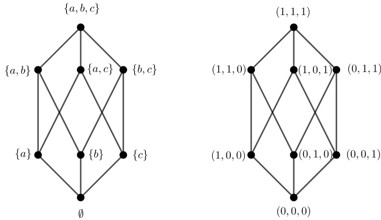
Figure 2.1: \mathcal{P}(\{a, b, c\}) is isomorphic to the boolean poset B_3 .
