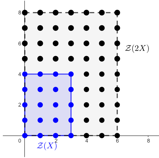
Figure 3.2: Integer points of a simple zonotope and its dilation by 2.
