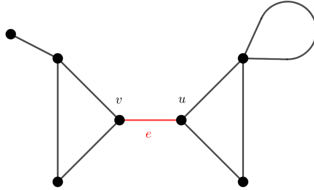
Figure 1.5: A graph with an distinct edge e = (u, v) .
