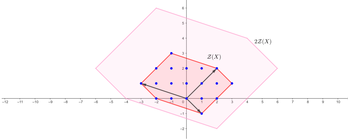
Figure 3.1: Integer points and the dilation of a zonotope.
