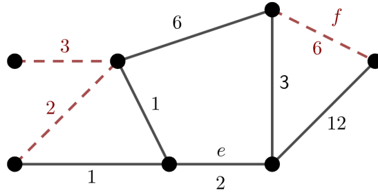
Figure 2.3: A labelled graph with regular edges (black) and dotted edges (brown).
