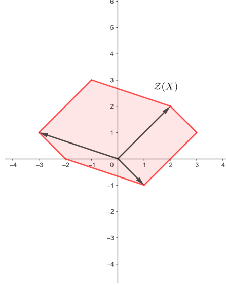
Figure 2.2: The zonotope \mathcal{Z}(X) .
