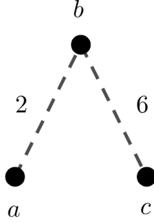
Figure 3.4: The simple counterexample.
