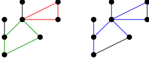
Figure 1.2: Circuits in red and green on the left and a basis marked in blue on the right.
