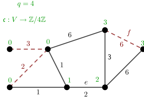
Figure 3.3: A proper arithmetic 4-colouring marked in green.
