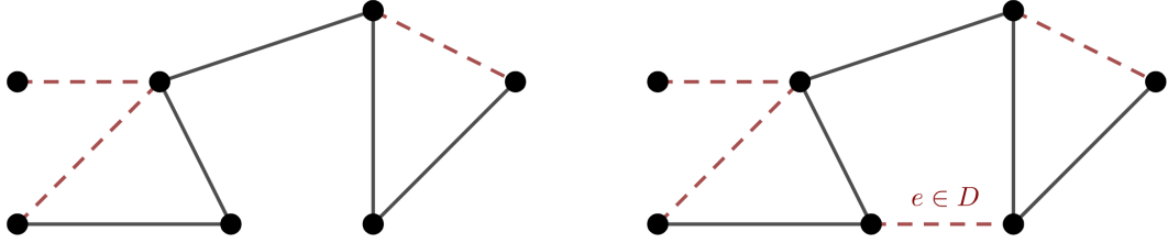
Figure 2.4: labelled deletion and contraction of the former regular edge e .
