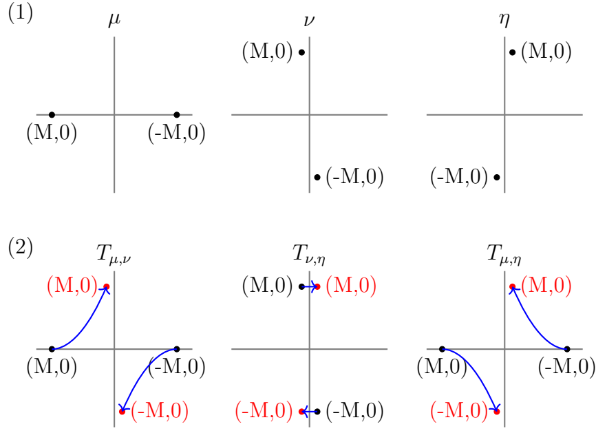
FIGURE 1. Example that the triangle inequality does not hold for the Knothe-Rosenblatt distance, see the proof of Lemma 4.1.
