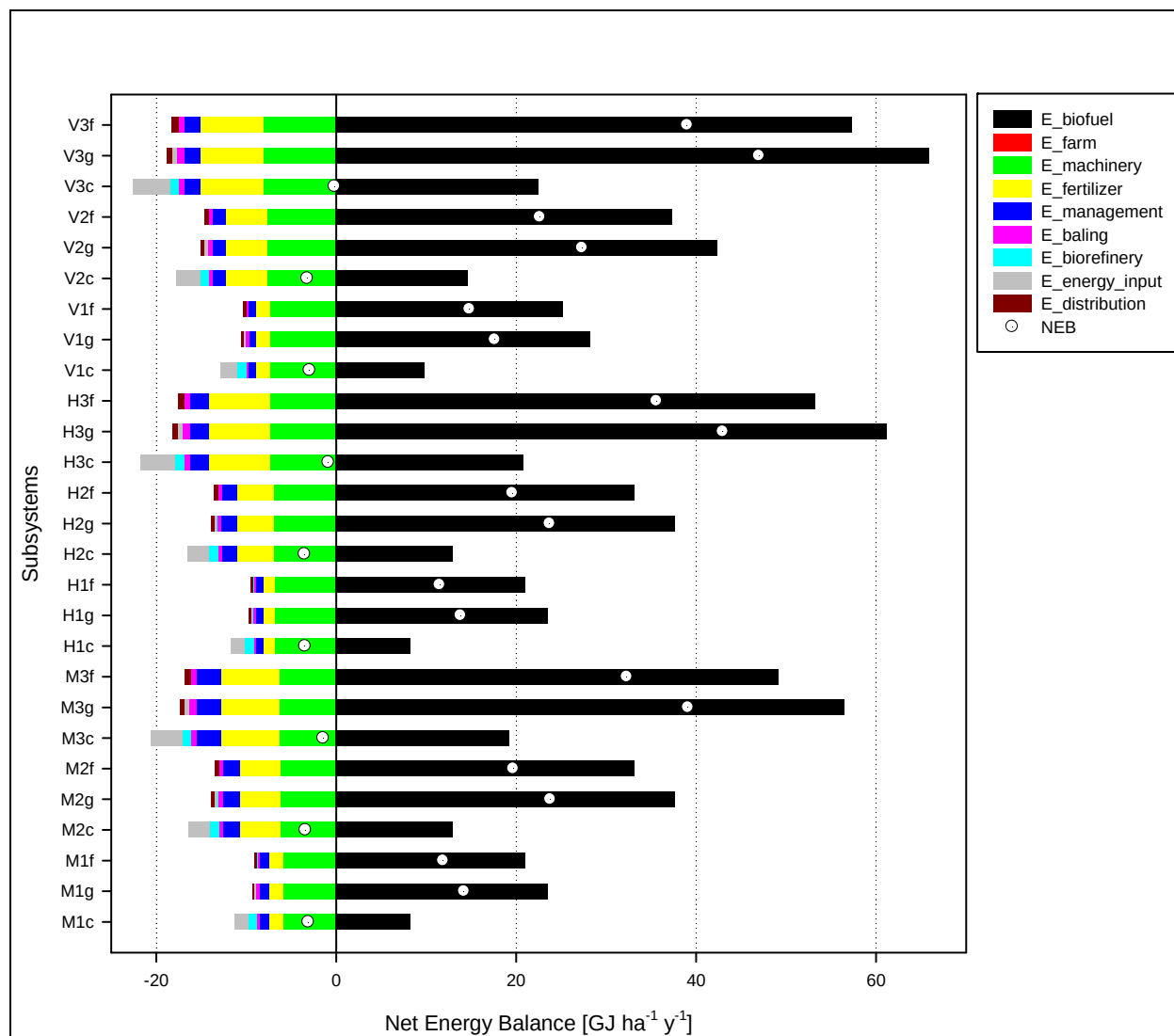
Figure 28: Net energy balance with constituent energy fluxes. Dots show values of NEB, calculated as sum of energy inputs and energy content of the biofuel. Subsystems are coded according to mean elevation above sea level (M = mountain, H = hillside, V = valley), management intensity (1 = one-cut, 2 = two-cut, 3 = three-cut) and conversion processes (c = combustion (CHP), g = gasification (bio-SNG), f = fermentation (LC-etOH)).
