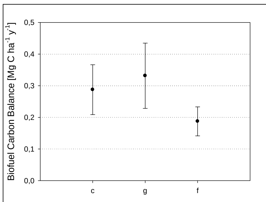
Figure 15: Biofuel carbon balances grouped for the factor conversion process. Letters indicate conversion processes (c = combustion (CHP), G = gasification (bio-SNG), and, f = fermentation (LC-etOH)). Fermentation subsystems emitted less carbon than combustion and gasification subsystems. Gasification subsystems returned the highest values for BCB. Whiskers show 99 % confidence intervals.
