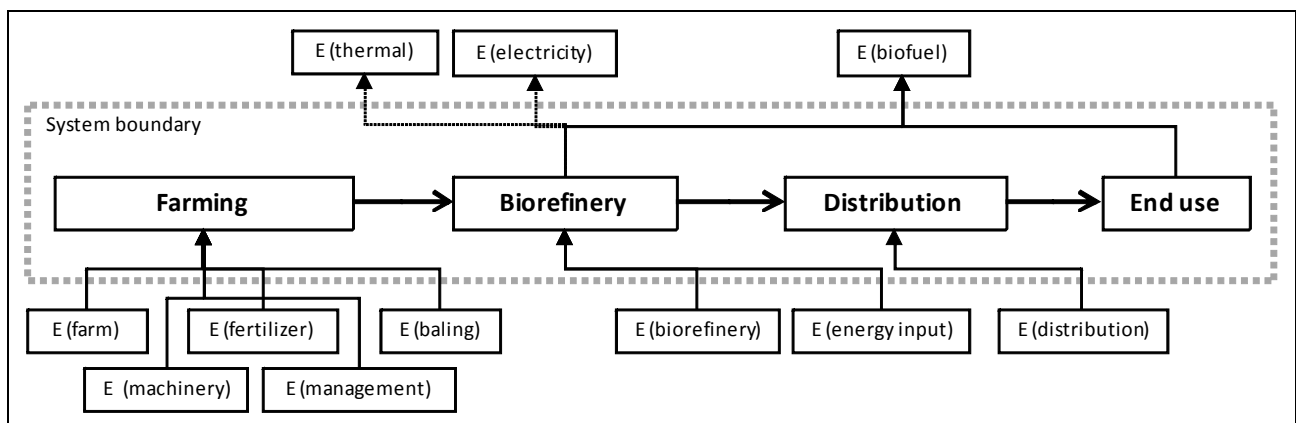
Figure 8: Schematic representation of the modelled net energy balance including co-products. The energy flow of biomass to biofuel is shown in thick continuous lines. Energy inputs and outputs are distinguished by direction of arrows. Co-products are distinguished by dotted lines.
