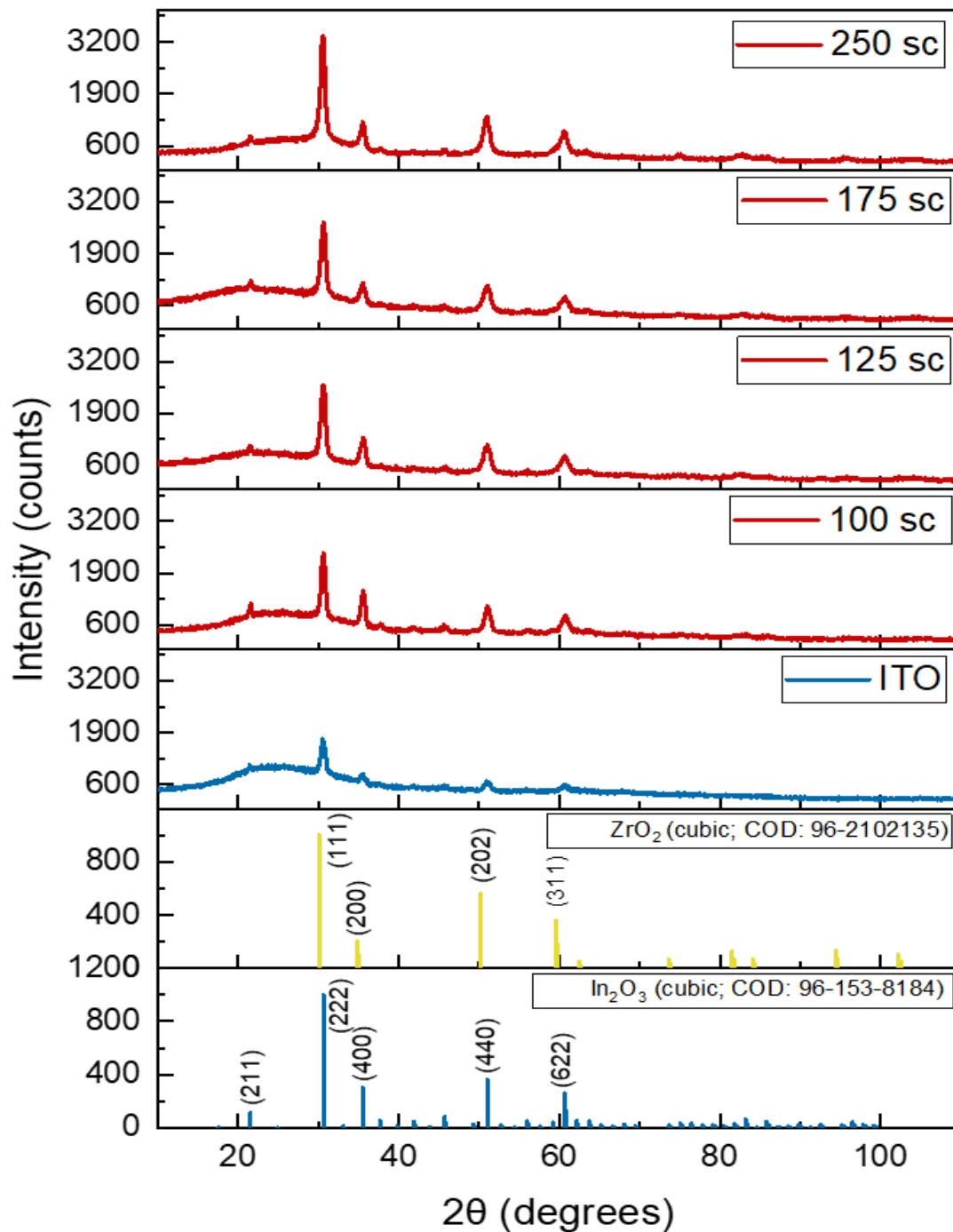
Figure 28: X-ray diffraction patterns of the cubic \text{ZrO}_2 films, sprayed at T=410^\circ\text{C} and c=100 mM with scanning numbers varying between 250 and 100 on ITO-coated glass. Also shown is the glass/ITO substrate diffractogram and the JCPDS standards for the cubic \text{ZrO}_2 and cubic \text{In}_2\text{O}_3 .
