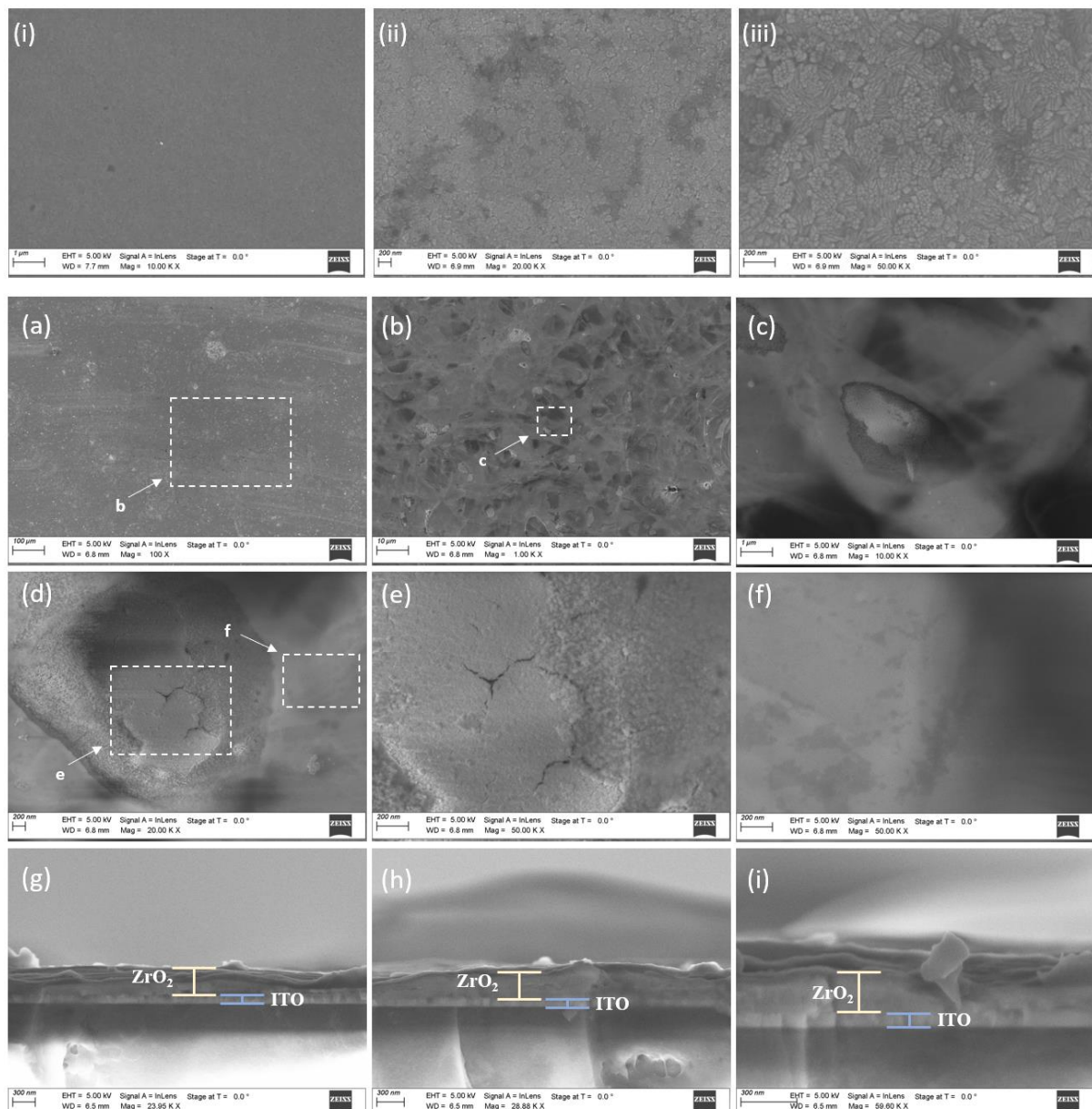
Figure 25: i)-iii) SEM micrographs of the glass/ITO substrate. a)-f) Plane-view and g)-i) cross-section SEM micrographs of the ITO/ \text{ZrO}_2 layer deposited from the 25 mM concentration solution.
