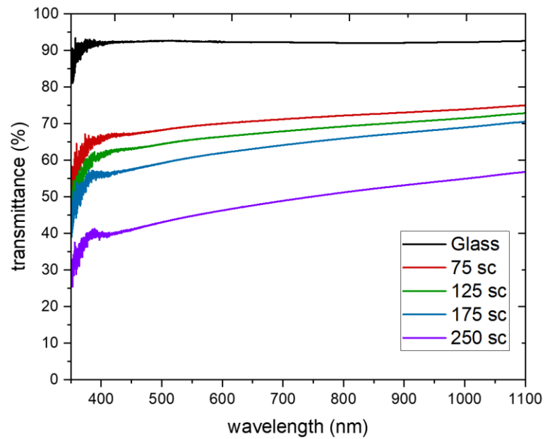
Figure 11: Optical transmission spectra of the cubic \text{ZrO}_2 films sprayed at T=410^\circ\text{C} and c=100\text{ mM} on borosilicate glass with scanning number ranging from 75 to 250 scans (sc.).
