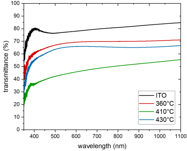
Figure 31: Optical transmission spectra of the cubic \text{ZrO}_2 , sprayed at temperatures between 360^\circ\text{C} and 430^\circ\text{C} on ITO-coated glass.
