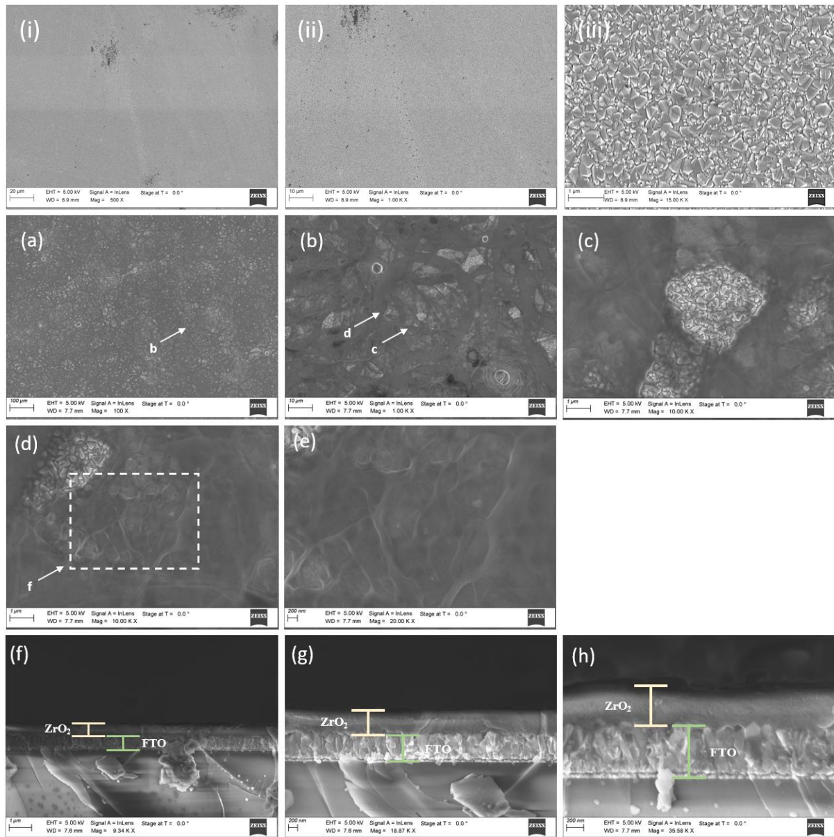
Figure 16: i)-iii) SEM micrographs of the glass/FTO substrate. a)-e) Plane-view and f)-h) cross-section SEM micrographs of the FTO/ \text{ZrO}_2 layer deposited from the 25 mM concentration solution.
