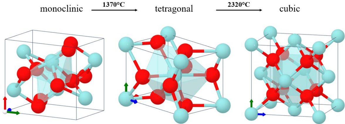
Figure 1: Polymorphic transformation for \text{ZrO}_2 and the corresponding space groups: (a) monoclinic ( P2_1/c ), (b) tetragonal ( P4_2/nmc ) and (c) cubic ( Fm\bar{3}m ) 23
