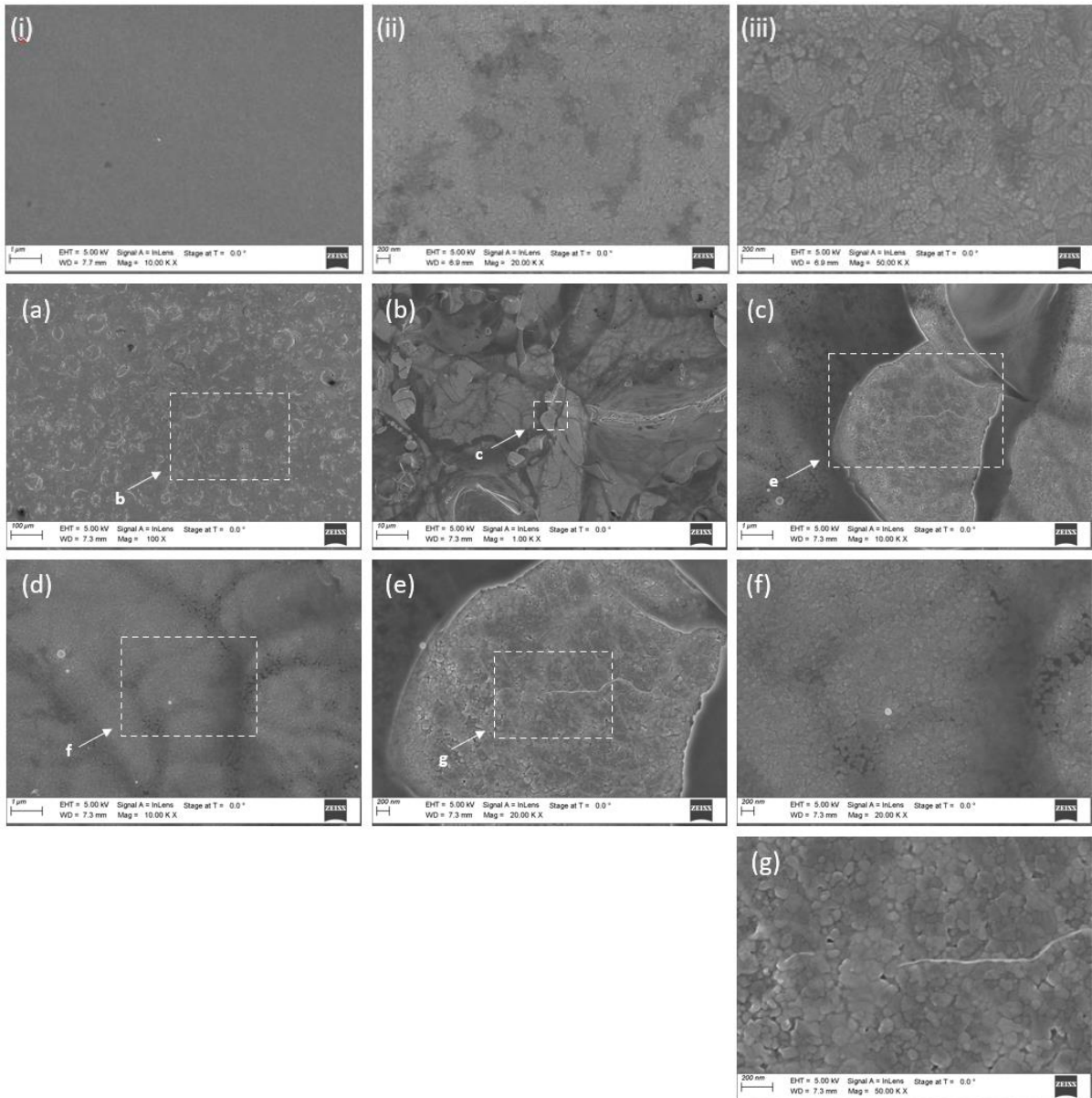
Figure 34: i)-iii) SEM micrographs of the glass/FTO substrate. a)-g) Plane-view SEM micrographs of FTO/ \text{ZrO}_2 film deposited \text{ZrO}_2 at 430°C.
