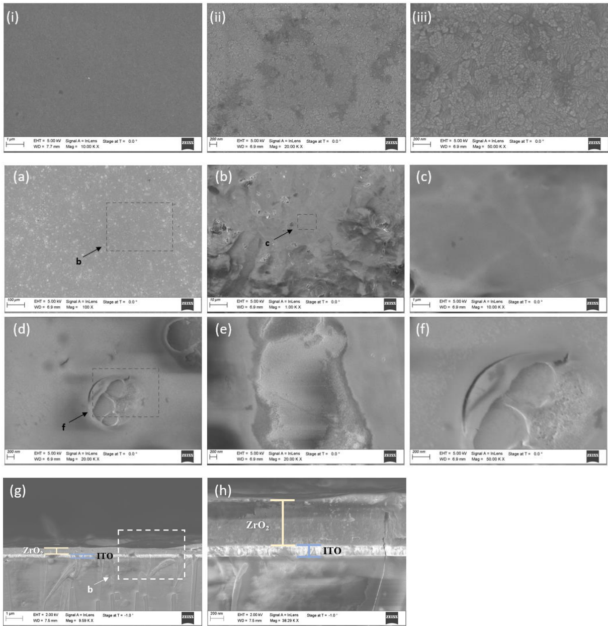
Figure 33: i)-iii) SEM micrographs of the glass/ITO substrate. a)-f) Plane-view and g)-h) cross-section SEM micrographs of ITO/ZrO 2 film deposited ZrO 2 at 410°C.
