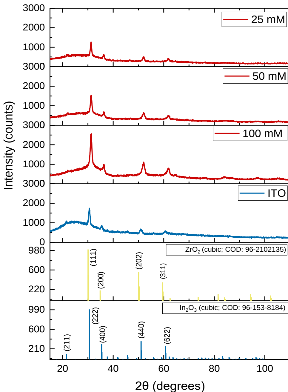
Figure 23: X-ray diffraction patterns of the cubic \text{ZrO}_2 films, sprayed onto a substrate with a T=380^\circ\text{C} at 200 scans, with varying concentrations of 25, 50 and 100 mM, on ITO-coated glass. Also shown is the glass/ITO substrate diffractogram and the JCPDS standards for the cubic \text{ZrO}_2 and cubic \text{In}_2\text{O}_3 .
