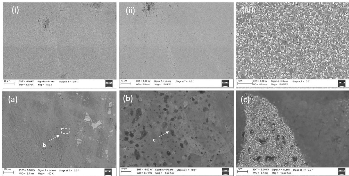
Figure 20: i)-iii) SEM micrographs of the glass/FTO substrate. a)-c) Plane-view SEM micrographs of FTO/ \text{ZrO}_2 film deposited at 360°C.
