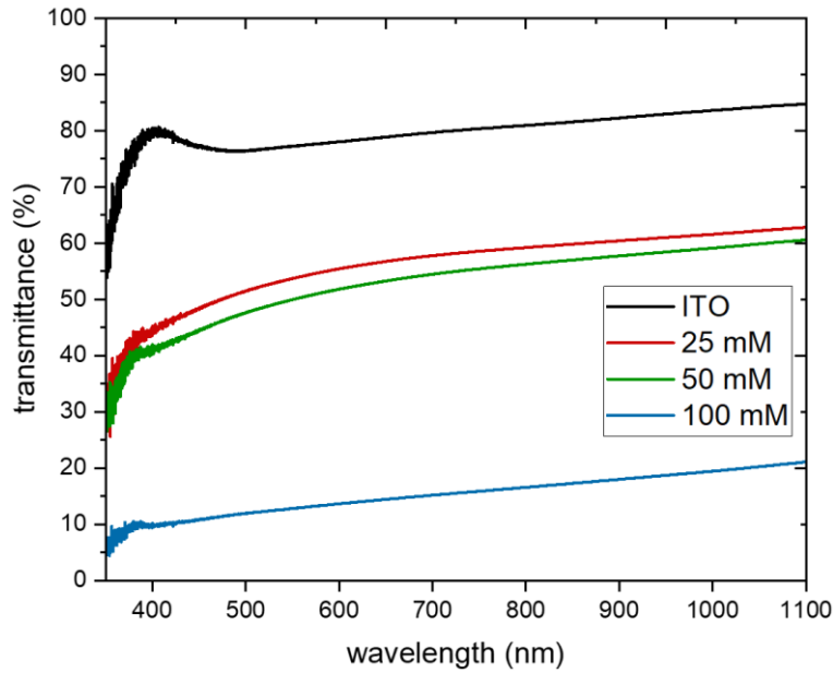
Figure 24: Optical transmission spectra of the cubic \text{ZrO}_2 films, sprayed at T=380^\circ\text{C} and 200 scanning repetitions with varying solution concentration of 25, 50 and 100 mM on ITO-coated glass.
