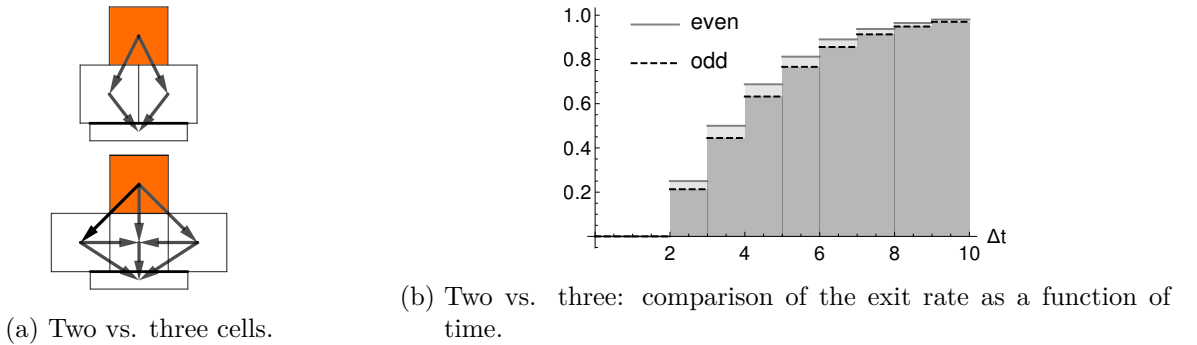
Figure 2.3: Discretization of the exit. In the case of an even number of cells, a central positioned agent will leave the corridor faster than in the case of three cells.
