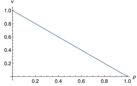
(b) Fundamental diagram for Burgers equation.
