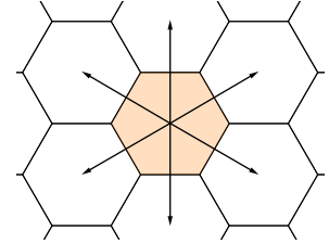
(c) A hexagon neighborhood.
