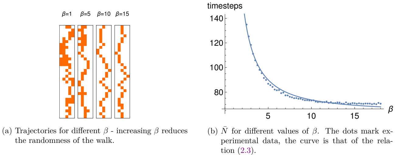
Figure 2.5: Influence of the scaling parameter \beta on individual dynamics.
