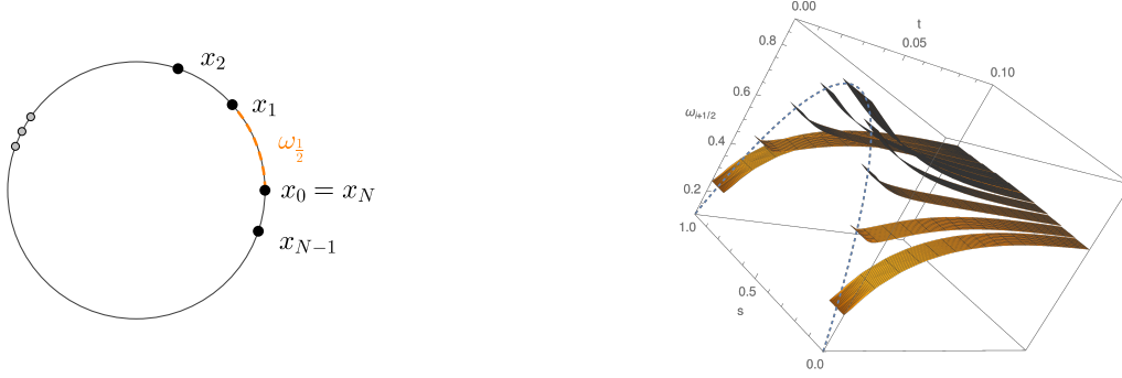
(a) We work with periodic boundary conditions in model (1.26), this can be seen as N agents x_i repelling each other on a circle.
