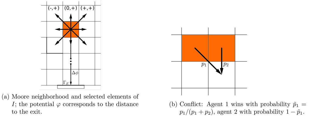
Figure 2.2: Cellular automaton: transition rules.
