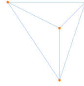
(b) Corresponding Delaunay-diagram, it is the dual graph.
