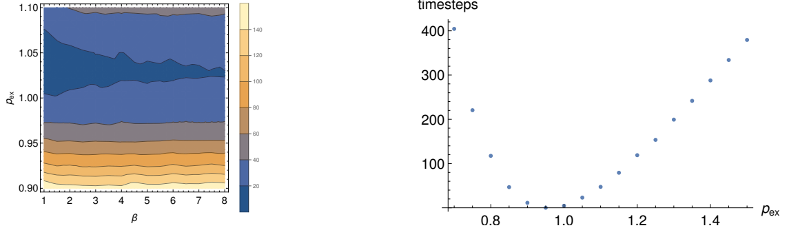
(a) The average exit time for a discrete set of \beta/p_{ex} -combinations.
