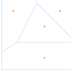
(a) Voronoi-diagram of random initial data in 2D.
