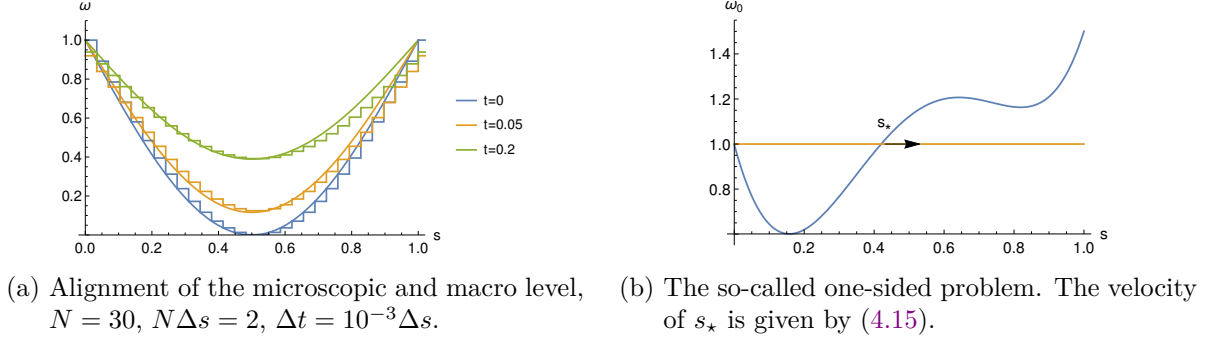
Figure 4.4: On the left we see alignment between the two scales for equation (4.11) in Lagrange-coordinates. On the right we see initial datum for the one-sided problem which will be the focus of our main investigation in Subsection 4.3.2.
