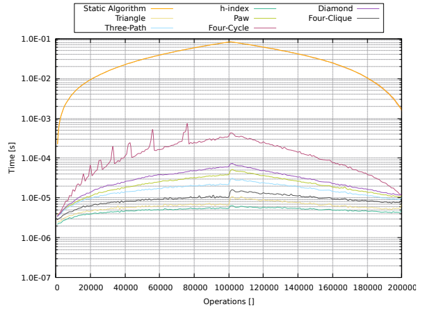
(d) Computing total subgraphs counts using the algorithm by Eppstein et al.
