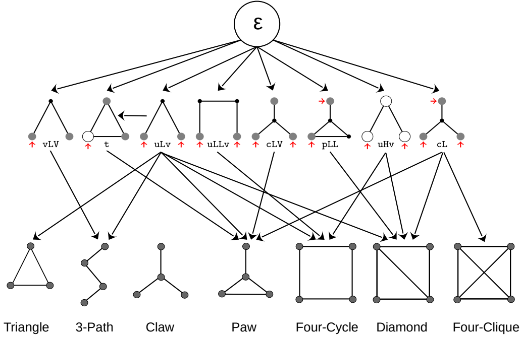
Figure 1: Overview of the dependencies between the different counts maintained by the algorithm by Hanauer et al.. The first row represents the epsilon partition. The second row shows the different substructures, where small dots represent low degree vertices, large and empty dots represent high degree vertices, and large filled dots represent any vertex. The anchor vertices are marked with a red arrow. (Pictograms taken from [12]) The last row depicts the subgraphs whose counts are the final results. Dependencies between elements are drawn as arrows.
