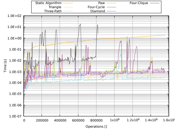
(b) Computing the total subgraph counts using the algorithm by Hanauer et al.
