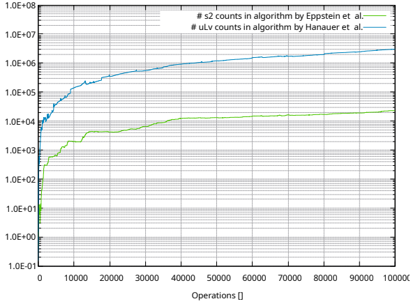
(c) Comparison between uLv and s2
