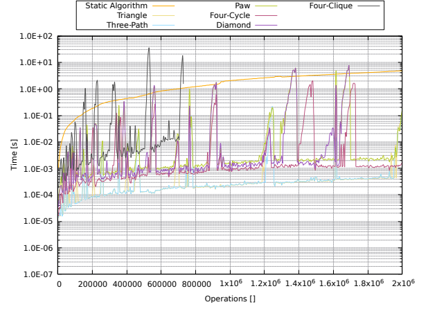
(b) Computing the total subgraph counts using the algorithm by Hanauer et al.
