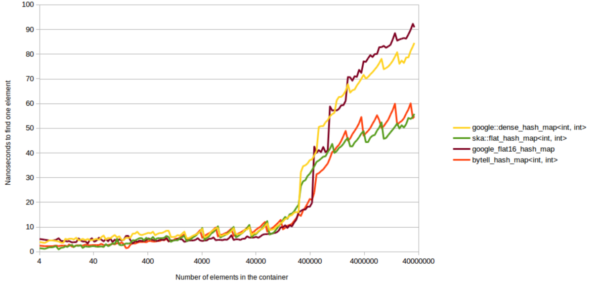
Figure 11: Speed of successful lookups for various hash maps using integer-keys. The hash map used for the implementation of both algorithms corresponds to the red line [24].
