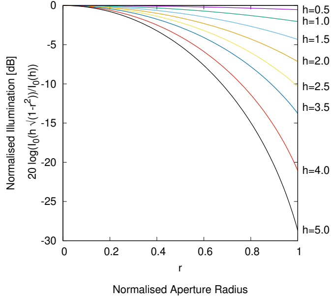
Figure 1.7: The efficiency of dish illumination is dependent on the choice of edge taper. While low tapers offer good consistency in signal power towards the edge of the aperture, it is also clear that a significant amount is lost past the boundaries of the dish.
