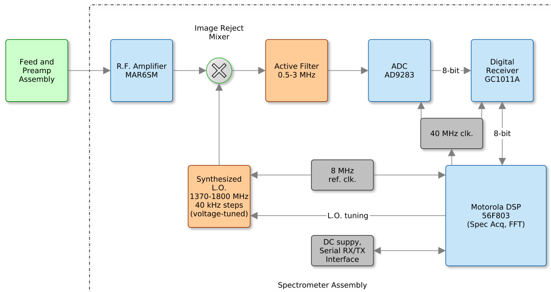
Figure 2.17: Block diagram of the spectrometer assembly
