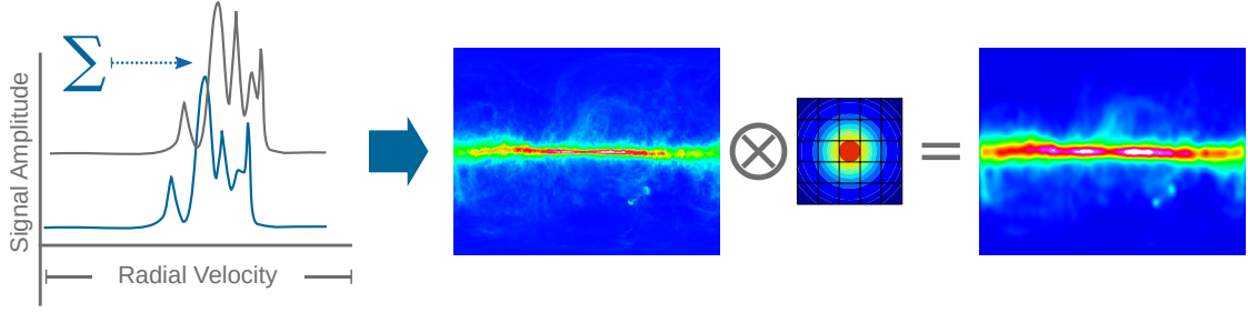
Figure 2.26: In the Fourier convolution approach, a map of the sky is first computed by integrating the spectra along their velocity axis for each position. Convolution with the beam is then performed on the flattened map.
