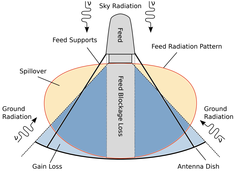
Figure 1.5: Signal losses in dish antenna configurations stem from the area shaded by the feed horn (or reflector in Cassegrain-type arrangements) and the loss of sensitivity due to the feed's radiation pattern, which results in imperfect illumination of the dish. A major ingress of unwanted thermal noise also comes from the feed radiation pattern, which partially looks at the ground behind the dish itself ( spillover ). The first sidelobe of the dish's radiation pattern also contributes spillover, when at low elevations (not illustrated).
