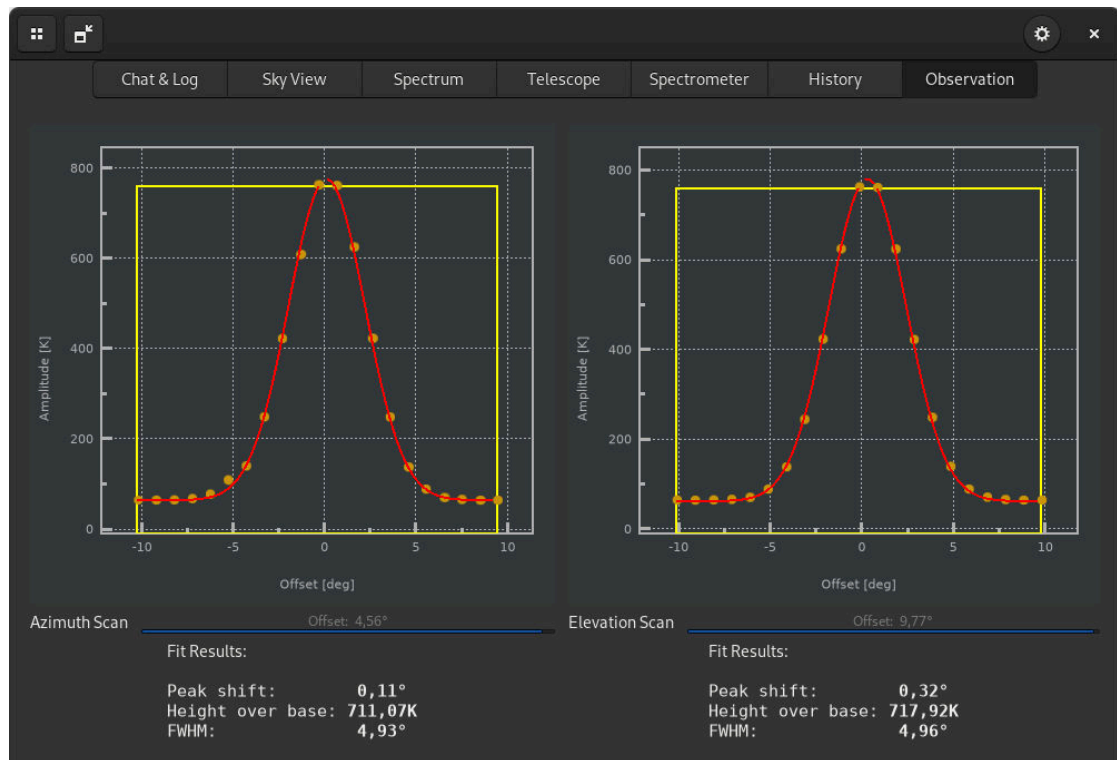
Figure 3.2: An example cross scan observation performed on the simulated Sun for a dish of D = 3 m. When completed, a Gaussian is fitted to the recorded data for both scan planes. The fitting results are shown below the graphs.
