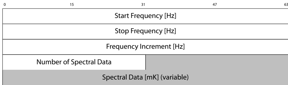
Figure 2.9: The structure of the Spectral Data payload packet. Frequencies are in units of Hz and treated as unsigned integers, spectral data are transported as equivalent temperature in mK as 32 bit integers.
