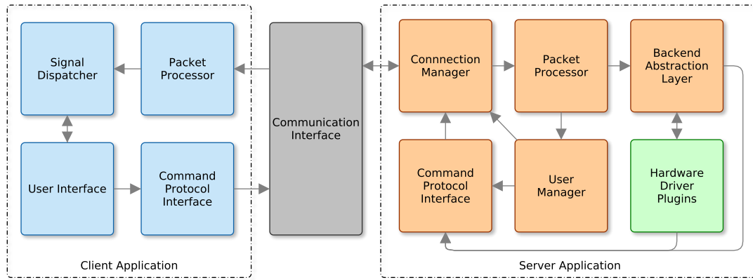
Figure 2.1: The top-level architecture of the software. It consists of a client and a server component which communicate via a network interface. Data is exchanged via command packets, which trigger functions in other parts of the software.
