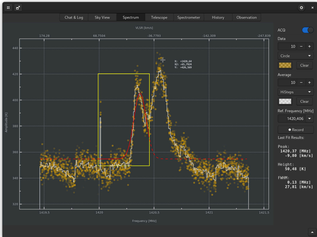
Figure 2.29: The Spectrum display shows individual spectra as a point cloud, while their moving average is drawn as a line. The depth of the stored data buffer, as well as the length of the moving average is user-configurable. Users may zoom and move the graph. Basic fitting of spectral lines is built-in. Other functions can be reached via a pop-up menu and keyboard commands.
