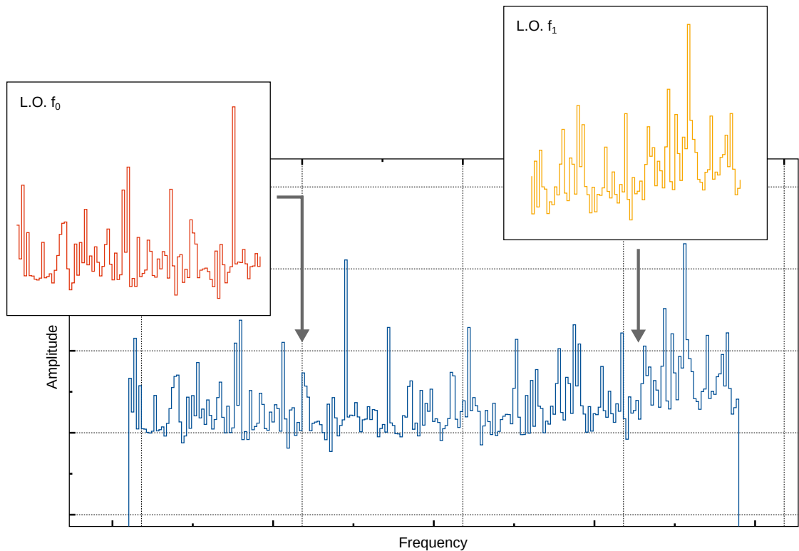
Figure 2.14: Spectra delivered to clients can be cut out of a fixed-width passband, if a smaller section is selected. Should the selected frequency range be larger than the passband, the delivered spectrum can be constructed from sequentially recorded and concatenated spectra, if the local oscillator frequency can be adjusted.
