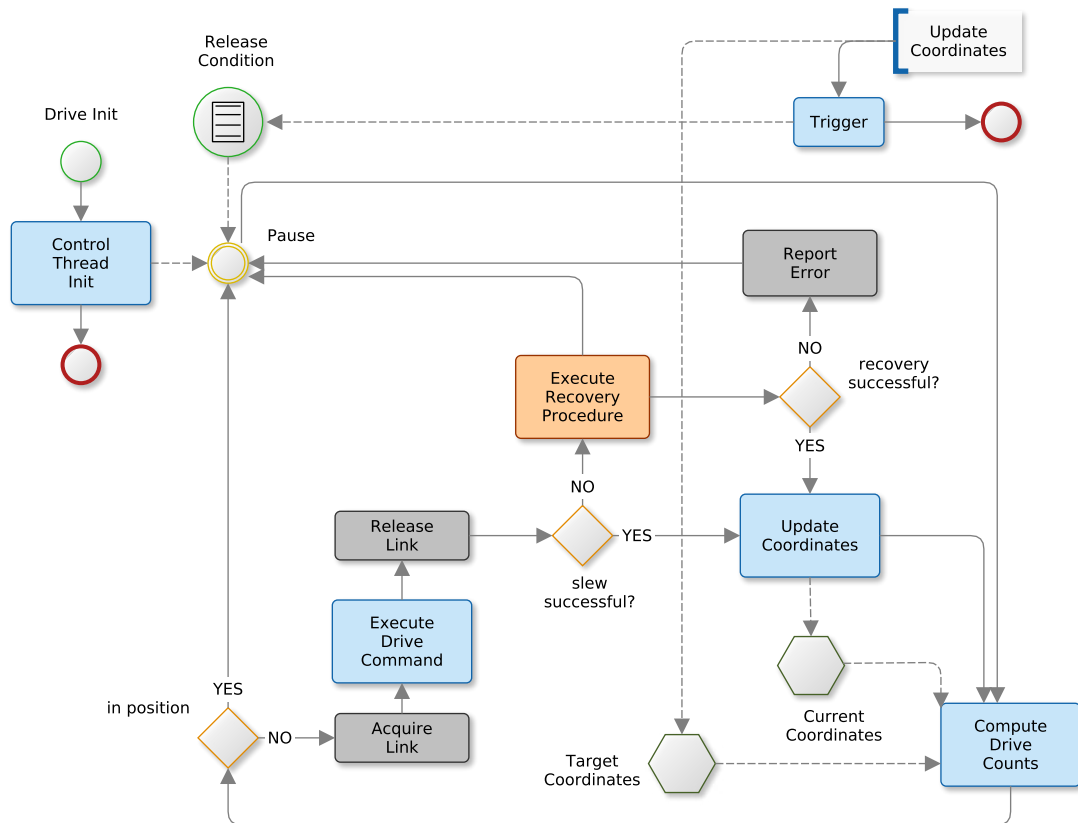
Figure 2.20: The operating principle of the drive plugin. On initialisation, a thread is created which waits until triggered, then executes the move to the new pointing. If an error (timeout) of the drive occurs, a recovery procedure is attempted. Note that this diagram only shows the primary control logic of the plugin.
