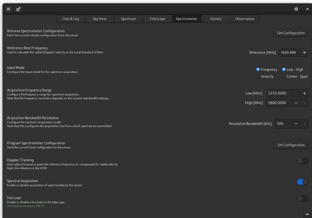
Figure 2.31: The Spectrometer settings follow a top-to-bottom workflow. The user sets up the configuration items step by step, before issuing a command to the server.
