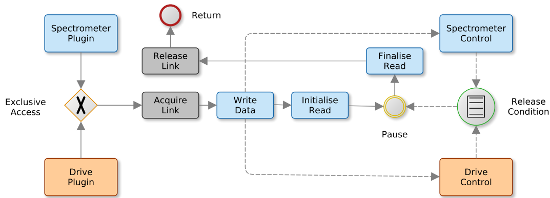
Figure 2.19: The SRT spectrometer and drive hardware cannot be controlled concurrently, as both components electrically share the same link interface. To ensure serialised access to the individual controllers, an intermediate software layer provides a unified interface to the spectrometer and drive control components and ensures mutually exclusive access.
