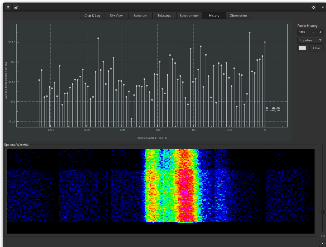
Figure 2.32: The History tab shows the continuum values of recorded spectra, with the most recent value marked in red and older data displayed towards the left. Below is a waterfall diagram of the spectra, with their amplitudes encoded in colour.
