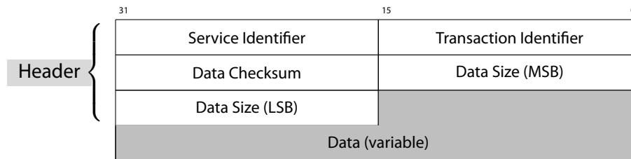
Figure 2.4: The structure of a protocol exchange packet. All fields with the exception of the Data field are mandatory. If a packet does not have an associated data payload, the data size field is set to 0 and the CRC16 is set to 0xFFFF , as demanded by the verification code generator used (see [15]).
