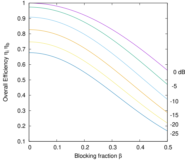
Figure 1.8: Overall efficiency is generally good for medium edge tapers and low feed blockages, which should not be larger than about 10 % of the main dish, otherwise performance degrades quickly. Note: edge taper curves are listed in terms of normalised illumination instead of h (see fig. 1.7).
