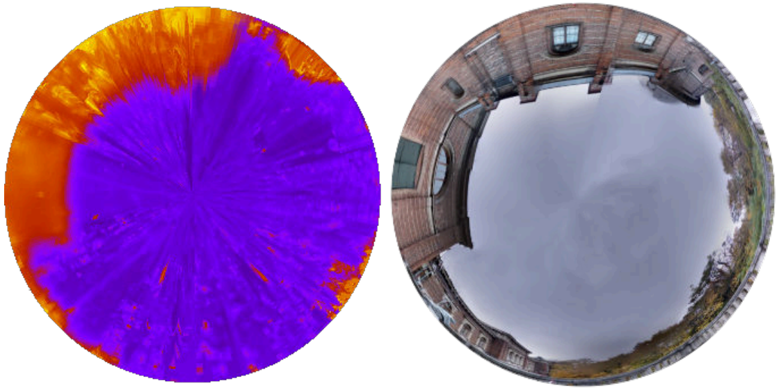
Figure 3.17: A map of the local environment of the SRT in radio is displayed on the left. For comparison, a fisheye-projected image of the optical view is shown on the right. The outlines of the building are clearly visible, even the shape of the telescope dome is recognisable, as are the emissions of a tall tree in the bottom right corner.
