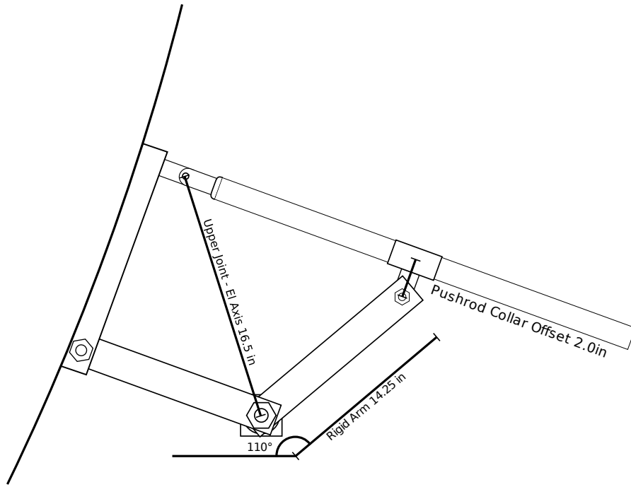
Figure 2.18: Schematic diagram of the CASSI elevation mount. All length values are given in U.S. customary units as per the original specification.
