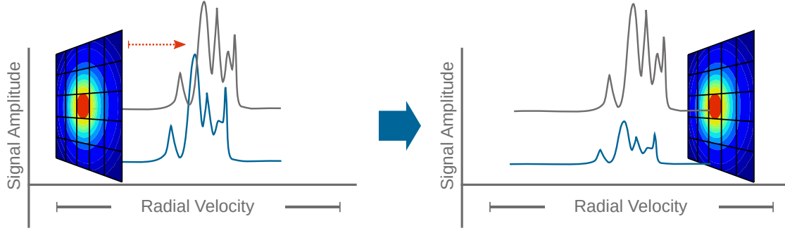
Figure 2.25: In the discrete convolution approach, the spectra within range of the target coordinate (given the beam size) are convolved by multiplication along the radial velocity axis, so their amplitude is scaled to appropriately reflect their contribution to the total signal contained in the beam. The processed spectra are then co-added, resulting in the final spectrum (not shown).
