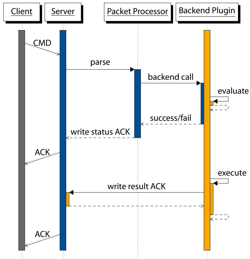
Figure 2.3: The execution profile of an asynchronous command. A service command packet sent by a client application is handed over to the packet processor, which parses the request and initiates the requested action on the backend plugin. The packet processor then immediately responds to the client with the outcome of the request, while the backend starts the process of executing the requested procedure. Once the procedure has completed, the backend independently transmits a second response packet to the client.
