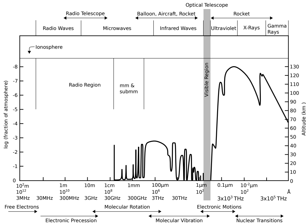
Figure 1.1: The transmission of the Earth's atmosphere for electromagnetic radiation. The diagram gives the height above sea level at which the radiation is attenuated by half. The absorption bands below 1 cm come mostly from \text{H}_2\text{O} and \text{O}_2 . Absorption above 300 GHz is caused by other abundant atmospheric gasses such as \text{N}_2 and \text{CO}_2 (fig. recreated from [1]).
