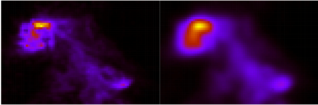
Figure 3.14: The Magellanic Clouds observed with simulated beams of 0.5^\circ (left) and 2^\circ (right) with a grid step size for both scans of 0.5^\circ , recorded between galactic latitudes -50^\circ to -25^\circ and longitudes 270^\circ to 310^\circ .
