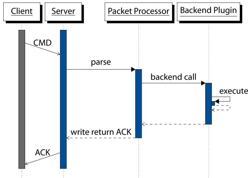
Figure 2.2: The execution profile of synchronous command processing. A service command packet sent by a client application is handed over to the packet processor, which parses the request and immediately executes the requested action on the backend plugin which has implemented and registered that action. A response packet is immediately returned to the client.
