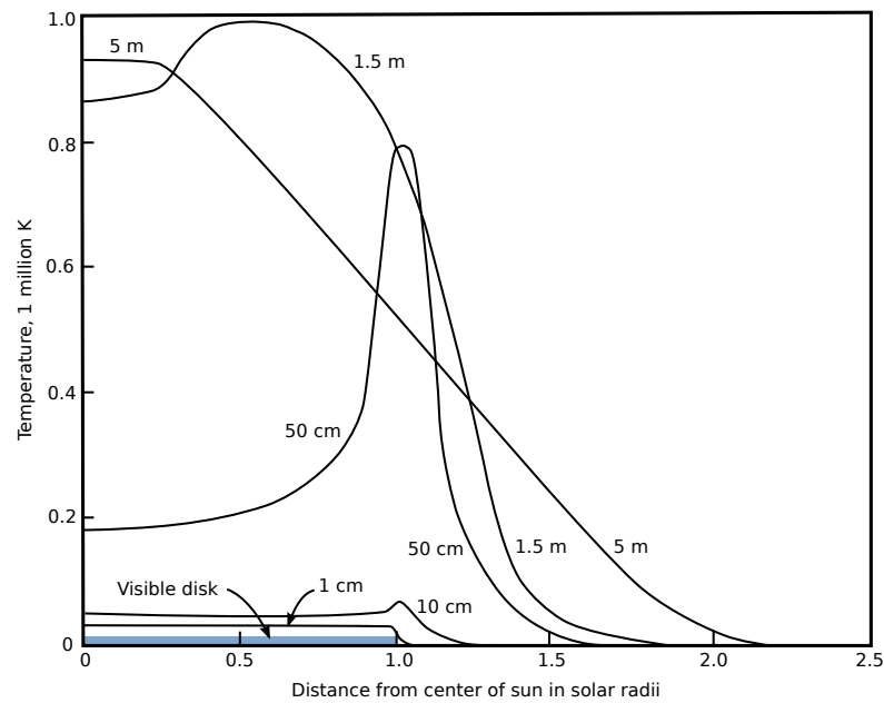
Figure 3.7: The predicted variation of the effective temperature with distance from the centre of the visual solar disk (blue) at different radio frequencies. Note that these curves are derived by ray-tracing a model of the solar corona for a given wavelength via the refractive index determined by the plasma oscillation frequency (1.1.1) for the given local electron densities ( fig. recreated from [32] ).
