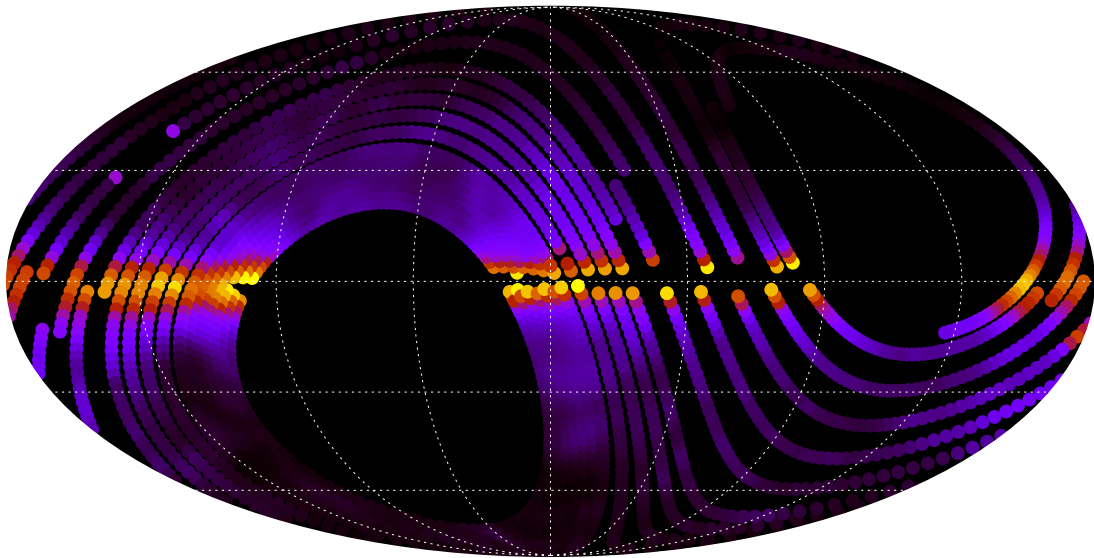
Figure 3.15: An example of (partial) drift scan lines for a simulated beam of 5^\circ in Mollweide projection.
