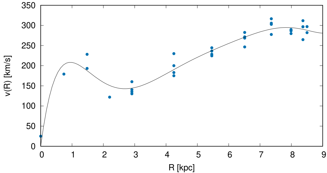
Figure 3.12: A galactic rotation curve measured for a simulated dish of D = 3 m. The data are fitted via a high-order polynomial.
