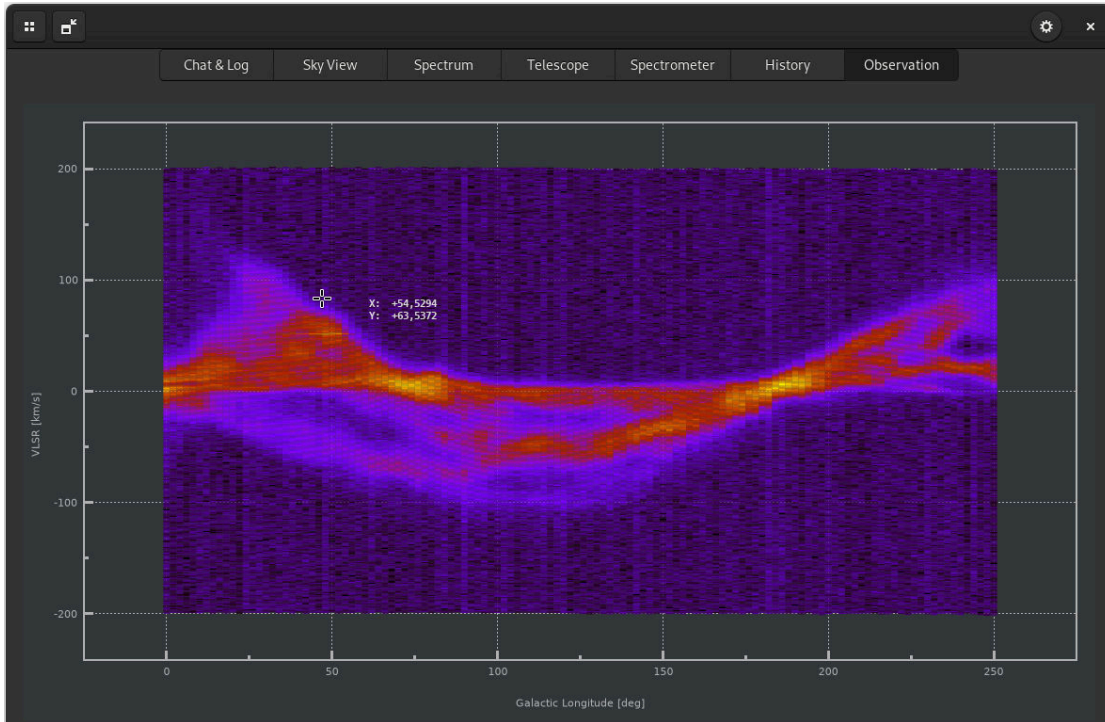
Figure 3.10: A position-velocity diagram recorded between galactic longitudes 0^\circ to 250^\circ for a simulated dish of D = 3 m using a step size of 2^\circ . Note that the mouse cursor position shows the velocity and longitude for immediate basic analysis.
