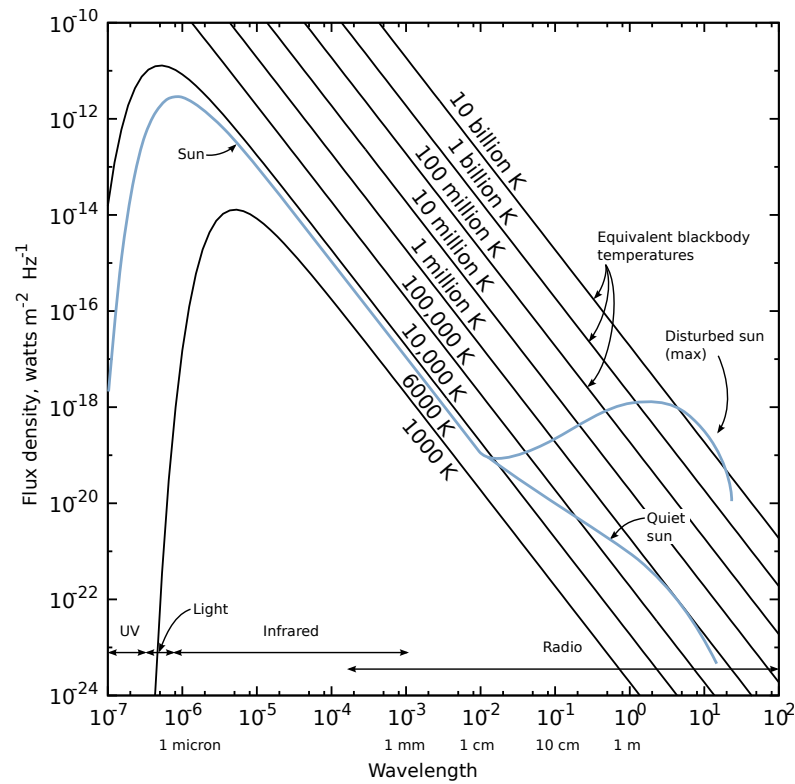
Figure 3.6: The solar spectral profile (blue curve) from the ultraviolet to radio wavelengths. The flux density is equal to that of a blackbody radiator at 6000K for wavelengths less than 1 cm, but deviates at longer wavelengths. In the radio, the observed flux varies with solar activity ( fig. recreated from [38] ).
