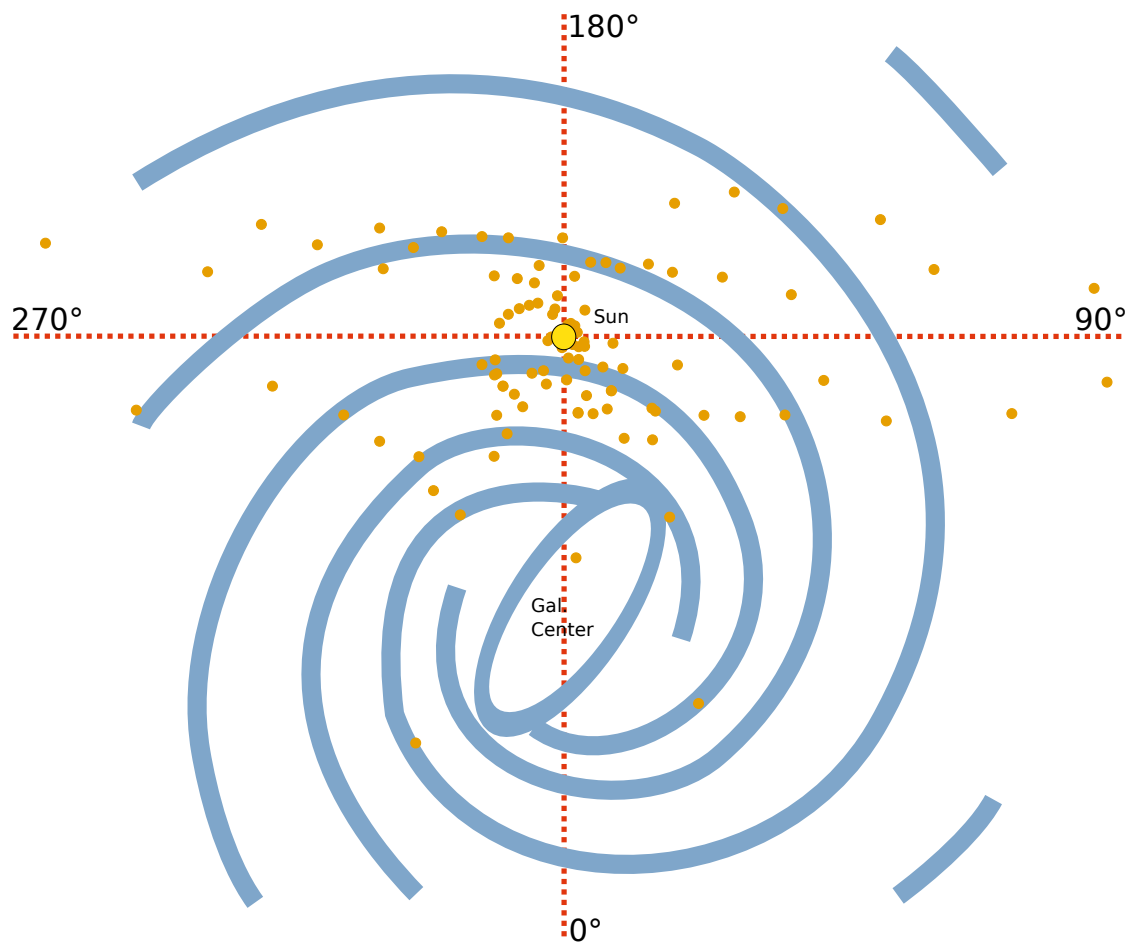
Figure 3.13: The measured distribution of spiral arms (dots) as measured with a simulated dish of D = 3 m. Proposed locations of spiral arms (solid lines) were taken from [41].
