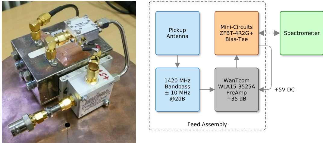
Figure 2.16: The signal from the feed's pickup antenna is filtered by a two-cavity bandpass and amplified in the WanTcom WLA15-3525A. Power is supplied by a Mini-Circuits ZFBT-4R2G+ bias-tee. The block diagram of the setup is on the right, the upgraded frontend assembly is on the left. (Photo courtesy of H. Chmela)
