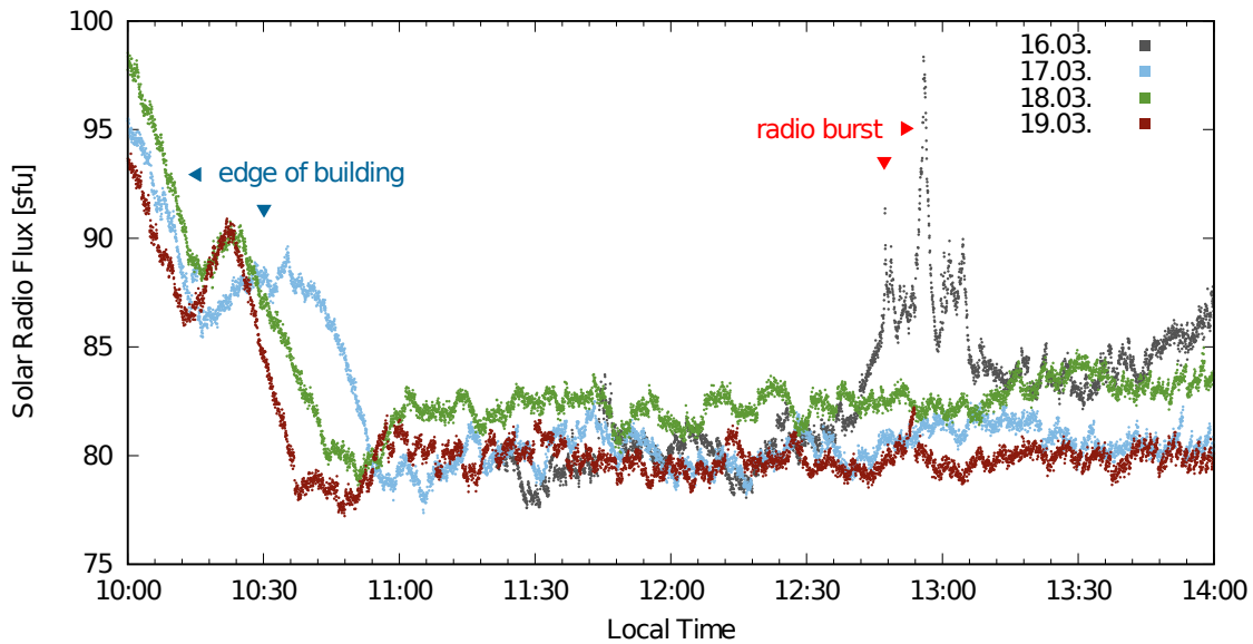
Figure 3.16: Solar activity was monitored for several days around local noon. A single radio burst event was recorded and is prominently visible. Note that the high levels of signal before about 10h30 come from the roof edge of the building next to the instrument. The distinct shape of the curves in this region are likely a case of Fresnel diffraction of the solar radio signal.
