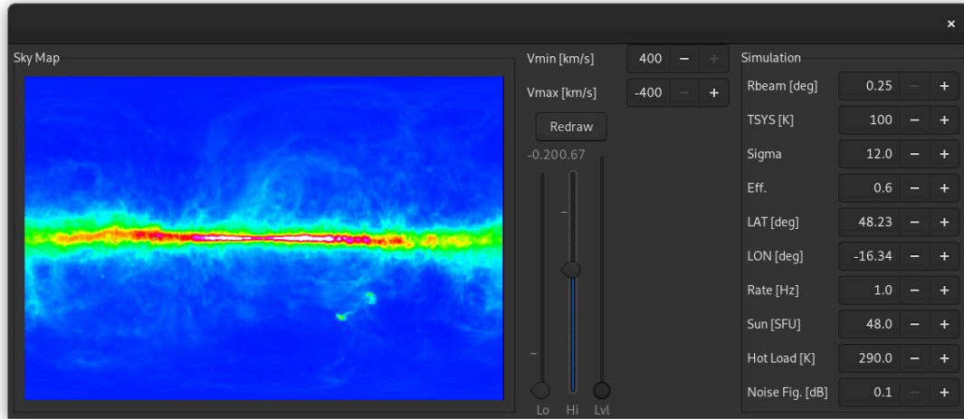
Figure 2.22: The user interface of the simulator plugin allows the user to configure various instrument parameters, such as beam size, geographical location and acquisition data rates. A rendered preview of the sky for the given beam size is also shown.
