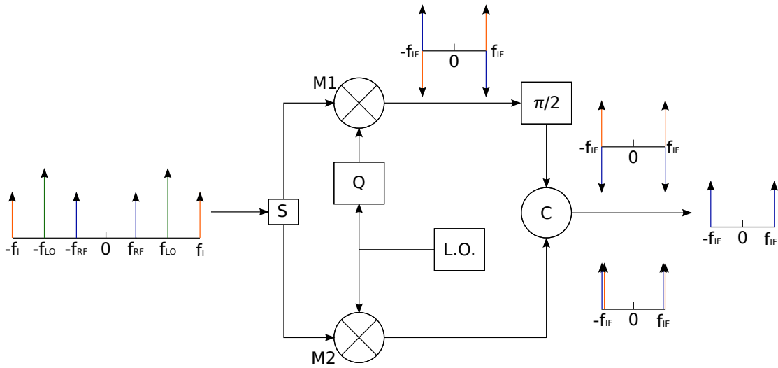
Figure 1.4: Working principle of an image reject mixer. The input signal (left) is divided in half by a splitter (S) and fed to the mixer inputs (M1, M2). The inputs are mixed with the signals from the local oscillator (L.O.), of which one is in in quadrature (Q) (i.e. an orthogonal sinusoid). The 90° phase-shifted signals are then recombined (C), resulting in the suppression of the unwanted sideband.
