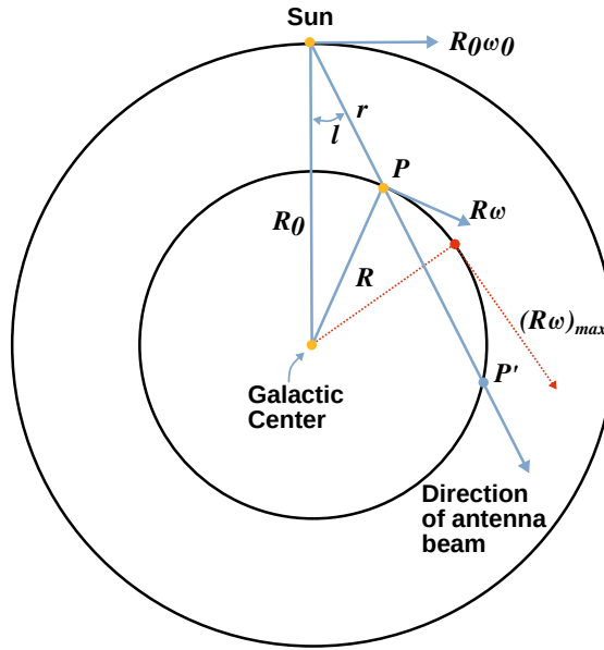
Figure 3.11: A simple model of galactic rotation as circular motion with decreasing angular rate for increasing distance from the centre. The maximum velocity of an orbit is tangential to the line of sight ( fig. recreated and adapted from [39] ).
