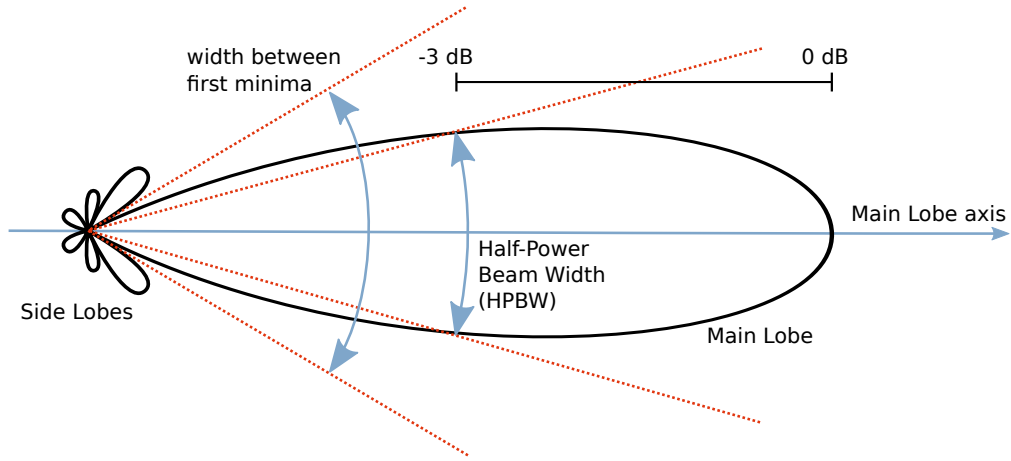
Figure 1.6: The idealised antenna beam consists of the main lobe, which contains the wanted signal components and the side lobes that contribute unwanted signals from other directions. The antenna resolution is considered to be the angular diameter at half the peak sensitivity (-3 dB) of the main lobe.
