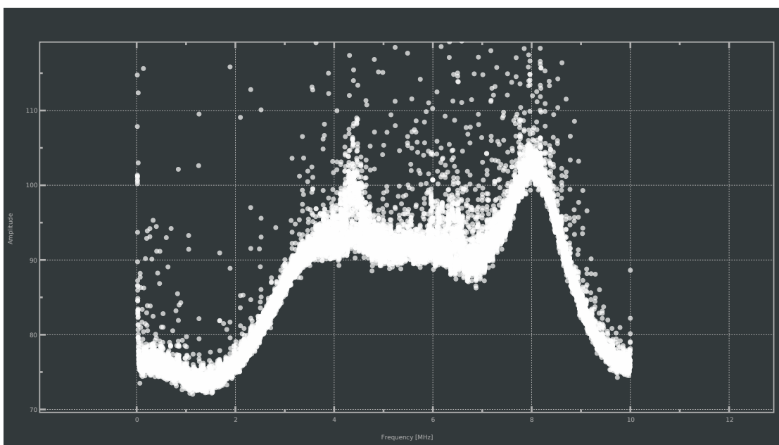
Figure 3.19: The characteristic spectral response of an instrument in the intermediate frequency band. Note that the amplitude is in arbitrary units. To obtain the curve, the pickup antenna input of the pre-amplifier was terminated with a 50 Ohm resistor.
