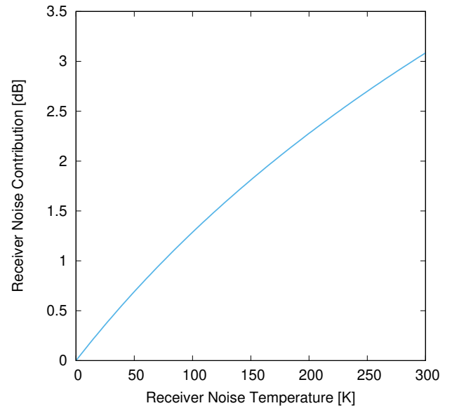
Figure 1.3: Noise figure for T_0 = 290\text{K} . It corresponds to the signal-to-noise ratio of a receiver, so an improvement of 1 dB will improve the SNR by about 1 dB.
