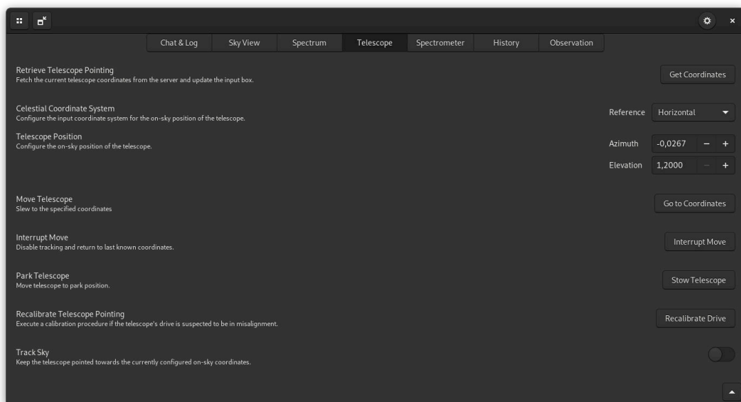
Figure 2.30: The Telescope pointing controls are arranged in top-to-bottom order, which allow the user to fetch, set and command the telescope drive unit parameters.
