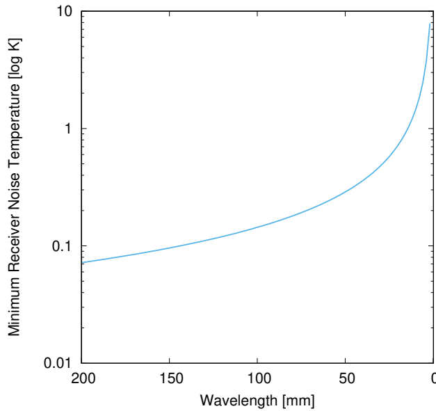
Figure 1.2: Minimum noise for a coherent receiver. The noise contribution is small for longer wavelengths, but quickly increases in the sub-millimetre range.
