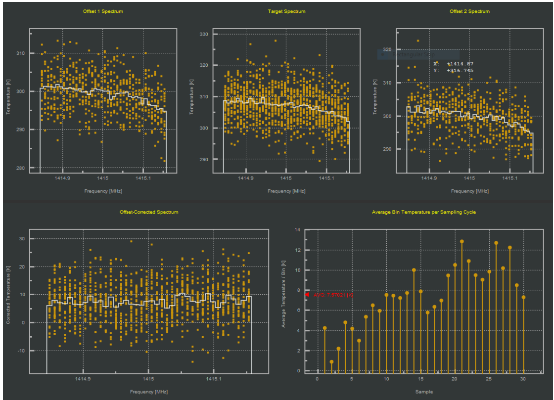
Figure 3.5: Beam switching performed on the Cygnus X star forming region with the SRT ( D = 2.3 m) shows the source signal to be about 7.6 K above background. For a flux density of 8000 Jansky, the resulting aperture efficiency is \eta_{\text{ap}} = 0.63 .
