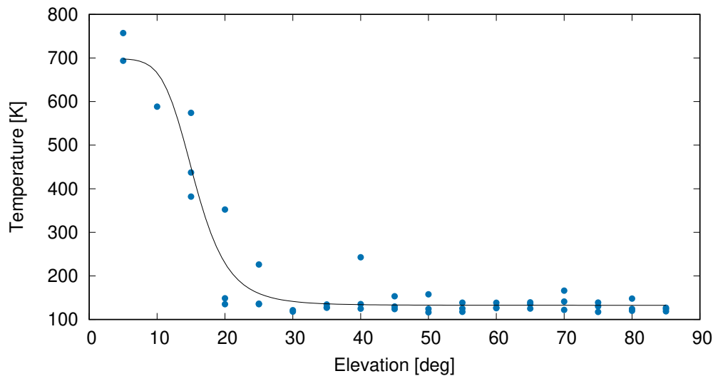
Figure 3.8: The spillover curve shown indicates significant contributions of signal coming from the ground up to elevations of 20°. This indicates partial illumination of the surroundings by the main beam, in addition to the radiation picked up by the side lobes.
