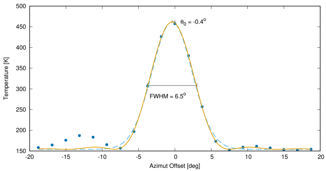
Figure 3.3: An example beam measurement of a real instrument. When compared to the radial cross-section of the Airy pattern (solid curve), it is apparent that a Gaussian (dashed curve) is a sufficient approximation of the main beam. Note that the increased signal at the negative offset is most likely not coming through a side lobe, but from a nearby object in the scan line, which is partially covered by the main beam. The slight increase at the positive offset is more likely to be a side lobe component.
