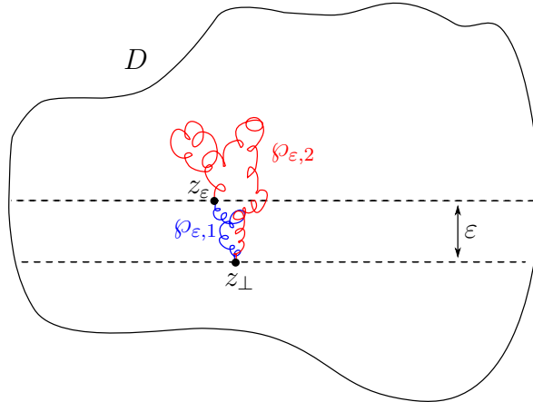
Figure 4.1: Rooting a loop at the point with minimal imaginary part.
