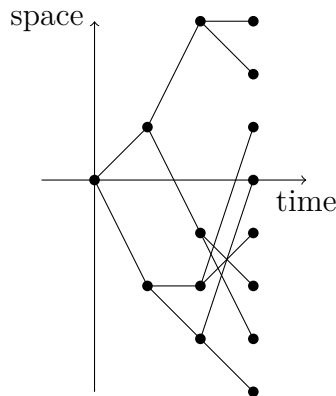
Figure 1.1: First three generations of a binary branching random walk.
