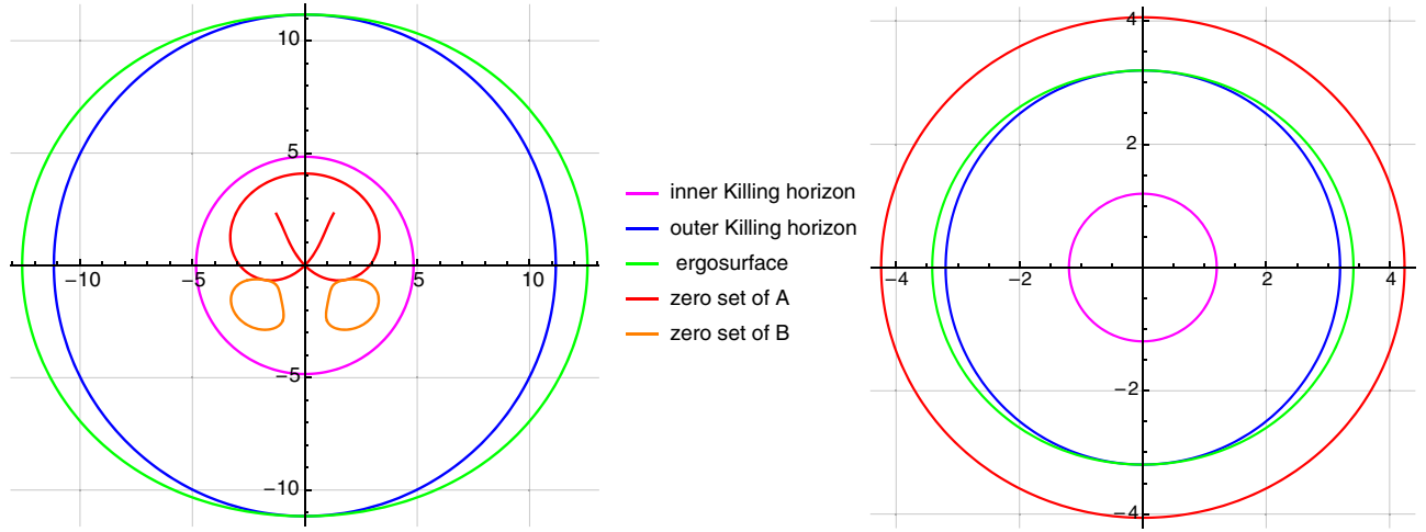
FIG. 1. Two sample plots for the location of the ergosurface (zeros of G ), the outer and inner Killing horizons (zeros of \Delta ), and the zeros of A , B . Left plot: M = 8 , a = \frac{33}{10} , Q = \frac{8}{5} , \Sigma = -\frac{23}{5} , P = -\frac{1}{5} \sqrt{\frac{2(4105960\sqrt{3}+2770943)}{12813}} \approx -7.86 , with zeros of A and B under both horizons, consistently with Eq. (A20) and (A22). Right plot: M = 1 , a = 1 , Q = 0 , \Sigma = \sqrt{6} , P = \sqrt{4 - 2\sqrt{2}} \approx 1.08 ; here, Eq. (A20) is violated, while the zeros of B occur at negative r .
