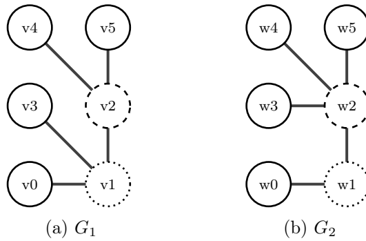
Figure 3.1: Two input graphs for the McSplit example. Vertex labels are encoded as the style of the outlines of vertices. McSplit produces the following mapping: v0 \rightarrow w0 , v1 \rightarrow w1 , v2 \rightarrow w2 , v4 \rightarrow w3 and v5 \rightarrow w4 .
