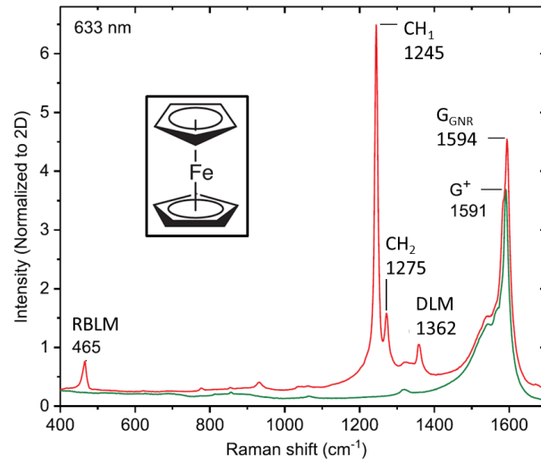
Figure 5.7: Raman modes of transformed ferrocene (molecular sketch in inset) encapsulated in SWCNT: RBLM at 465\text{ cm}^{-1} , CH 1 at \sim 1245\text{ cm}^{-1} , CH 2 mode at \sim 1275\text{ cm}^{-1} , D-like mode (DLM) at \sim 1362\text{ cm}^{-1} and G-band at 1594\text{ cm}^{-1} . Adapted from [125].
