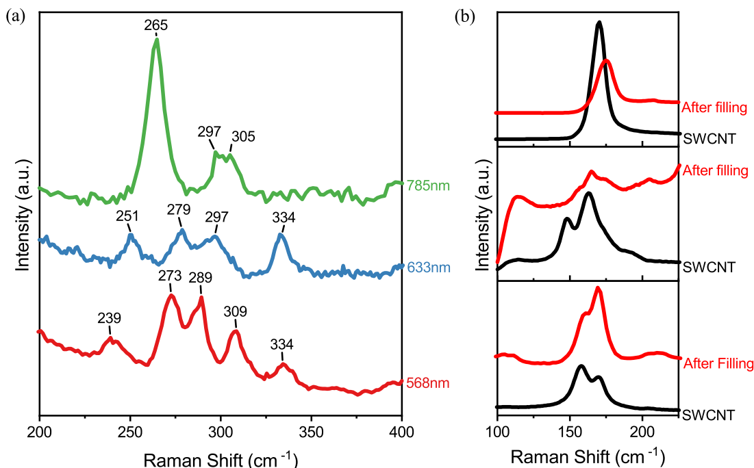
Figure 8.3: (a) RBMs of DWCNTs synthesized after heating at 1550 °C, recorded at 568nm, 633 nm and 785 nm. (b) Comparison between RBMs of encapsulating SWCNT before and after filling. The modes up-shift and change shape due to a changed force constant. Recorded at at 568 nm (top) 633 nm (middle) and 785 nm (bottom).
