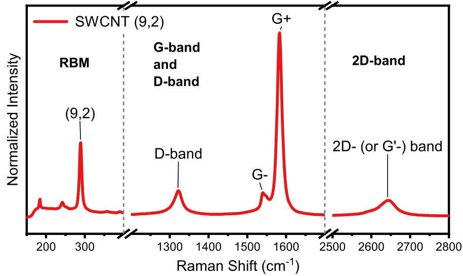
Figure 5.2: Raman spectrum recorded at 568 nm of a high-purity (9,2) SWCNT sample. Typical high intensity SWCNT modes are visible: RBM, D-band, G-band split into G+ and G-, and 2D- (or G'-) mode. Additional peaks in the RBM region are due to slight contamination by other chiralities. Data adapted from [142].
