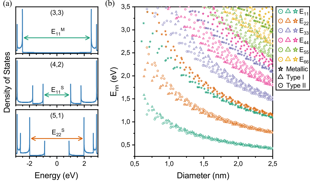
Figure 3.7: (a) Examples of DoS for the smallest allowed SWCNTs: metallic (3,3), type I (4,2), type II (5,1). Adapted from [68]. (b) Theoretical excitonic Kataura plot showing the relation between diameter and allowed optical transitions in SWCNTs.[66, 67]
