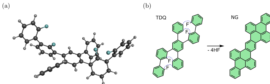
Figure 6.1: (a) Ball-and-stick sketch of tetrafluoro-diphenyl-quinguephenyl (TDQ). (b) TDQ precursor and expected cyclodehydrofluorination into heptacene dipyrene (NG) under ideal conditions [110].
