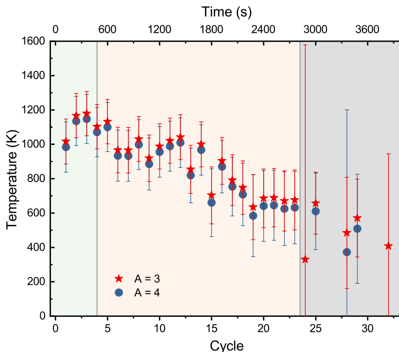
Figure 7.6: Temperature evolution during laser annealing calculated with equation 5.9. The standard deviation was calculated with equation 7.3. The temperature increases sharply from room temperature to about 1100K at the beginning of the process (green shading) and then gradually decreases (orange shading). The values after cycle 23 (grey shading) are unreliable due to lower signal-to-noise ratios.
