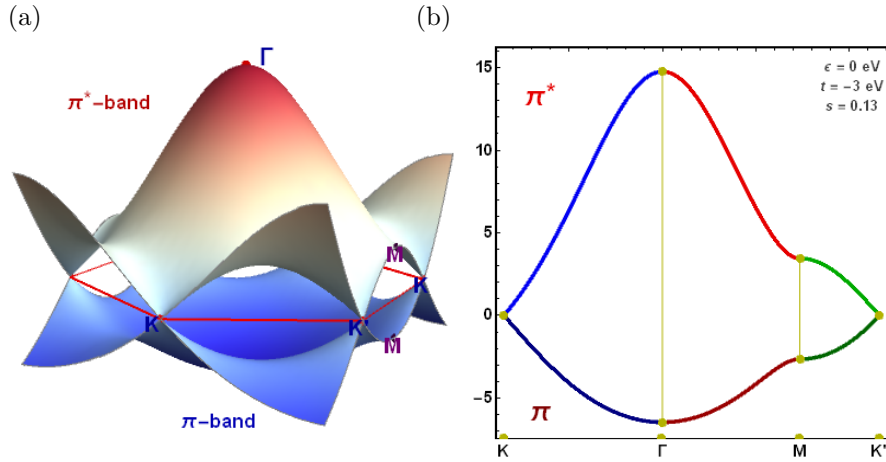
Figure 3.2: (a) Electronic energy dispersion of graphene in the first Brilluoin zone (b) and along high symmetry directions, generated from [62].
