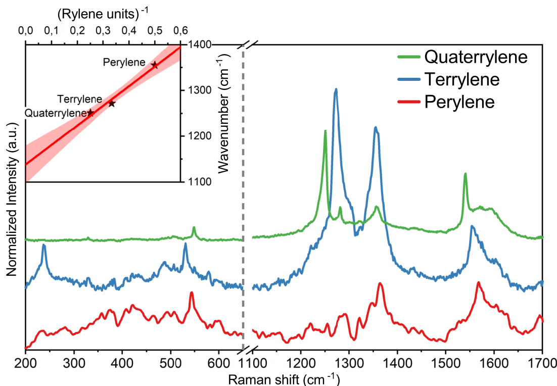
Figure 8.2: Comparison of Raman fingerprints of perylene, terryene and quaterrylene recorded at 568nm, after background subtraction and normalization to the G-line. Inset: position of the highest CH-mode as function of inverse number of rylene groups in the molecule, overlapped with linear fit and one standard deviation confidence band.
