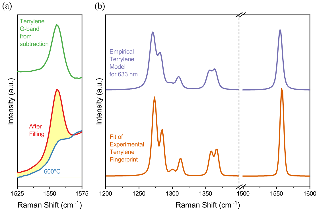
Figure 8.11: Creation of the empirical terrylene model for the 633nm wavelength. (a) The difference between spectra after filling (red spectrum) and after annealing at 600 °C (blue spectrum) is computed. The resulting peak is the extrapolated G-band of terrylene, which is then fitted to a Voigt profile to find the width broadening factor b_l and possible calibration shifts. (b) The data found in (a) is used to adapt the fitted model for the experimental terrylene fingerprint found in section 8.1.1 to the wavelength under examination.
