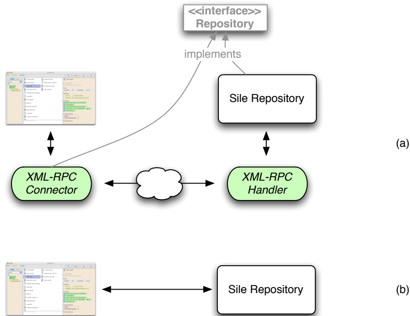
Figure 6.4: Distributed connector/handler architecture
