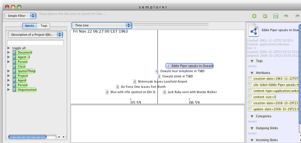
Figure 8.4: Semplorer timeline view [Tod08]
