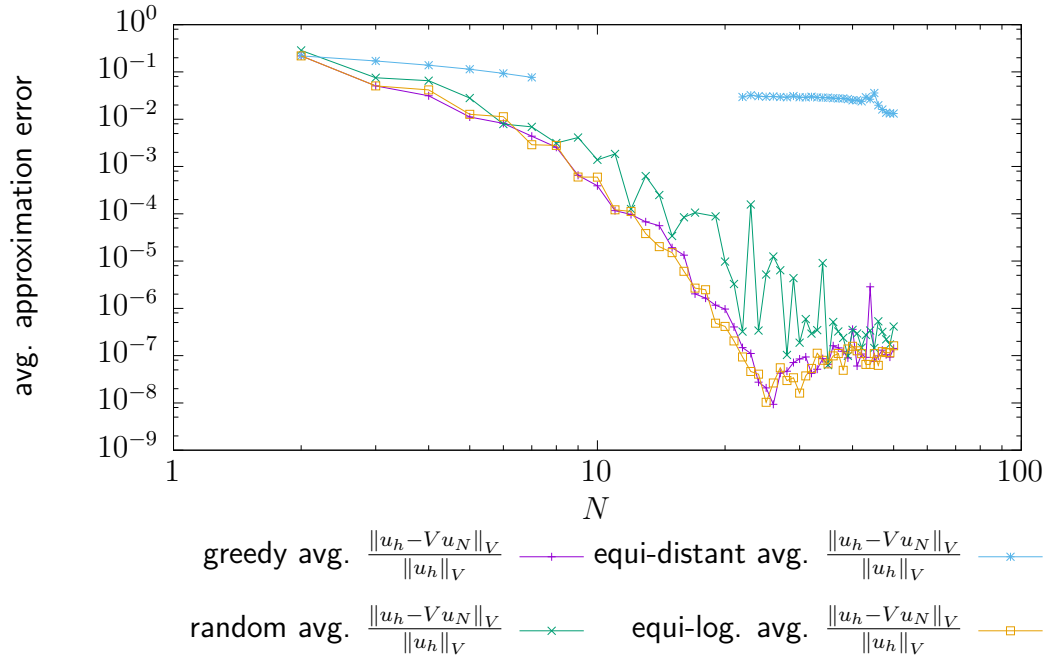
Figure 3.5: Average approximation error for different RB spaces for problem (3.9).
