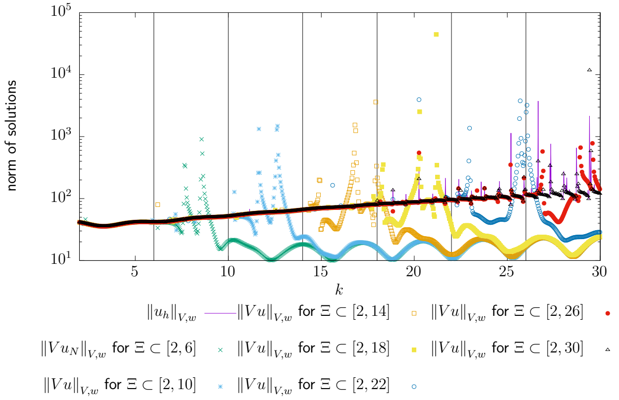
Figure 4.11: Comparison of different RB spaces for the transmission/reflection problem (4.9). The RB are constructed using training sets \Xi taken from different intervals.
