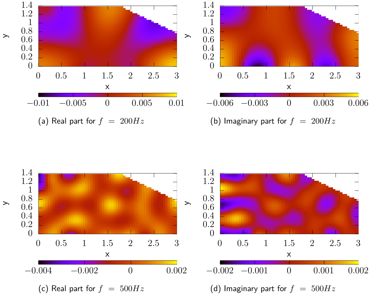
Figure 5.2: Exact solutions to problem (5.7).
