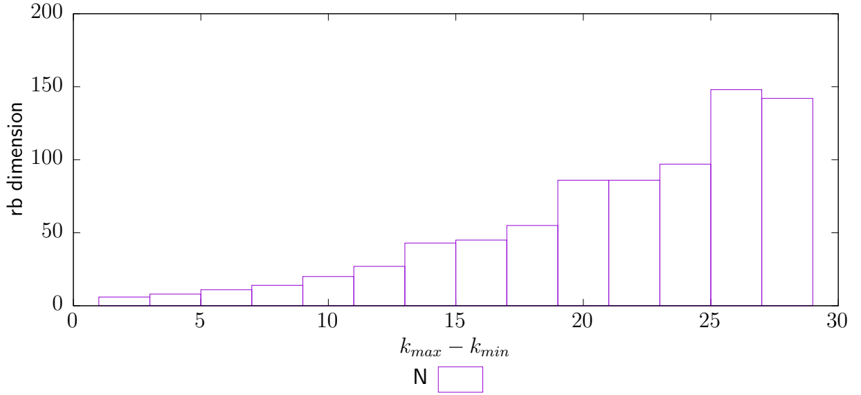
Figure 4.15: Dimensions of RB spaces depending on the interval length k_{max} - k_{min} for the transmission/reflection problem (4.9).
