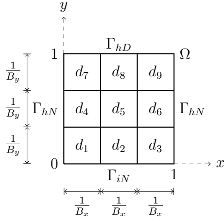
Figure 3.2: Thermal block domain \Omega for B_x = 3 and B_y = 3 .
