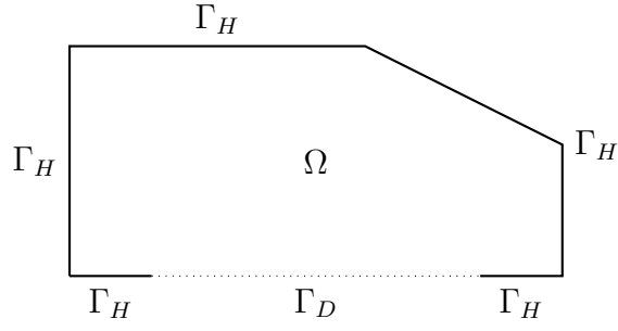
Figure 5.1: The domain and boundaries for problem (5.7).
