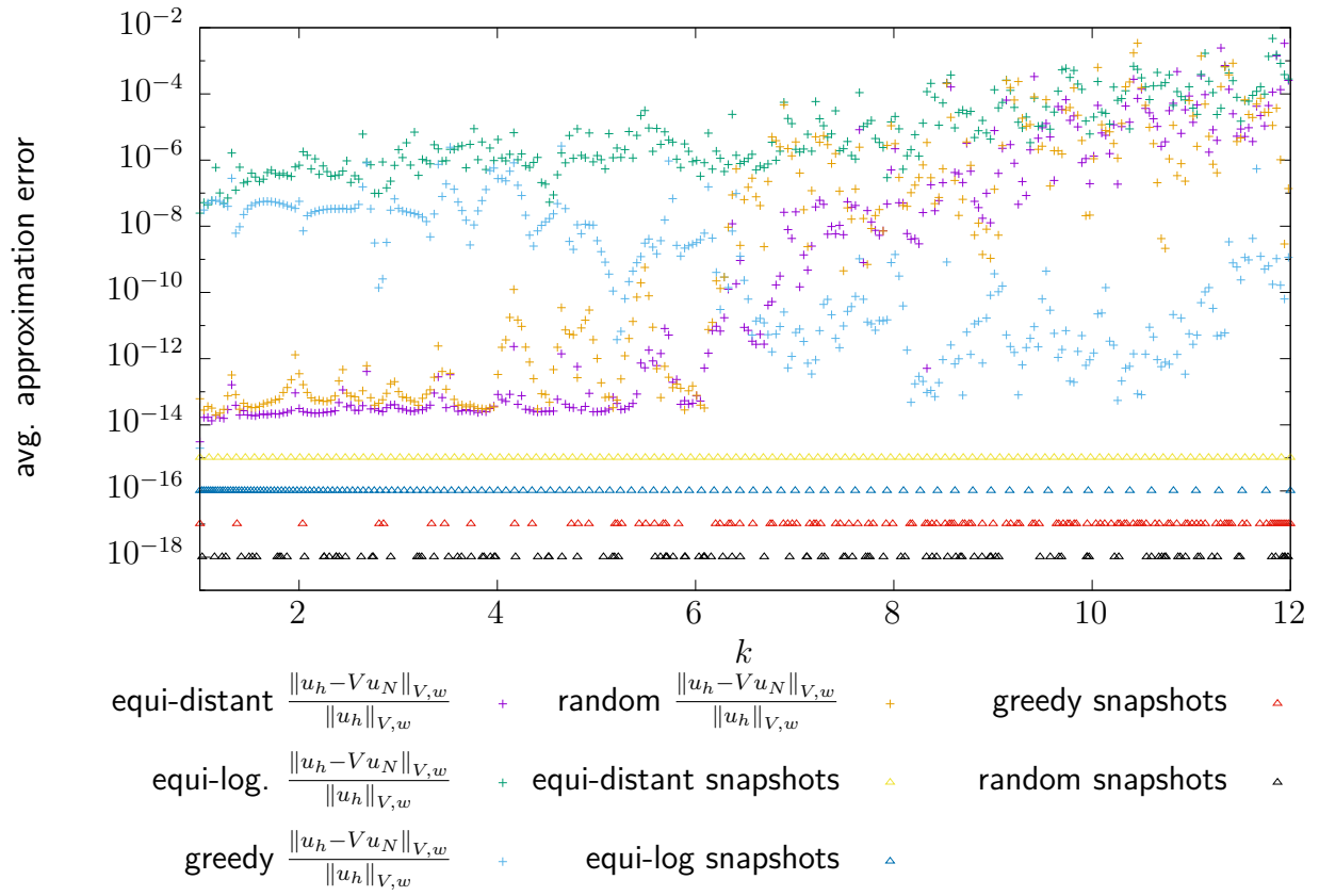
Figure 4.7: Comparison of the different construction strategies for RB spaces for the transmission/reflection problem (4.9). The approximation errors are marked by crosses. The snapshots are marked using triangles.
