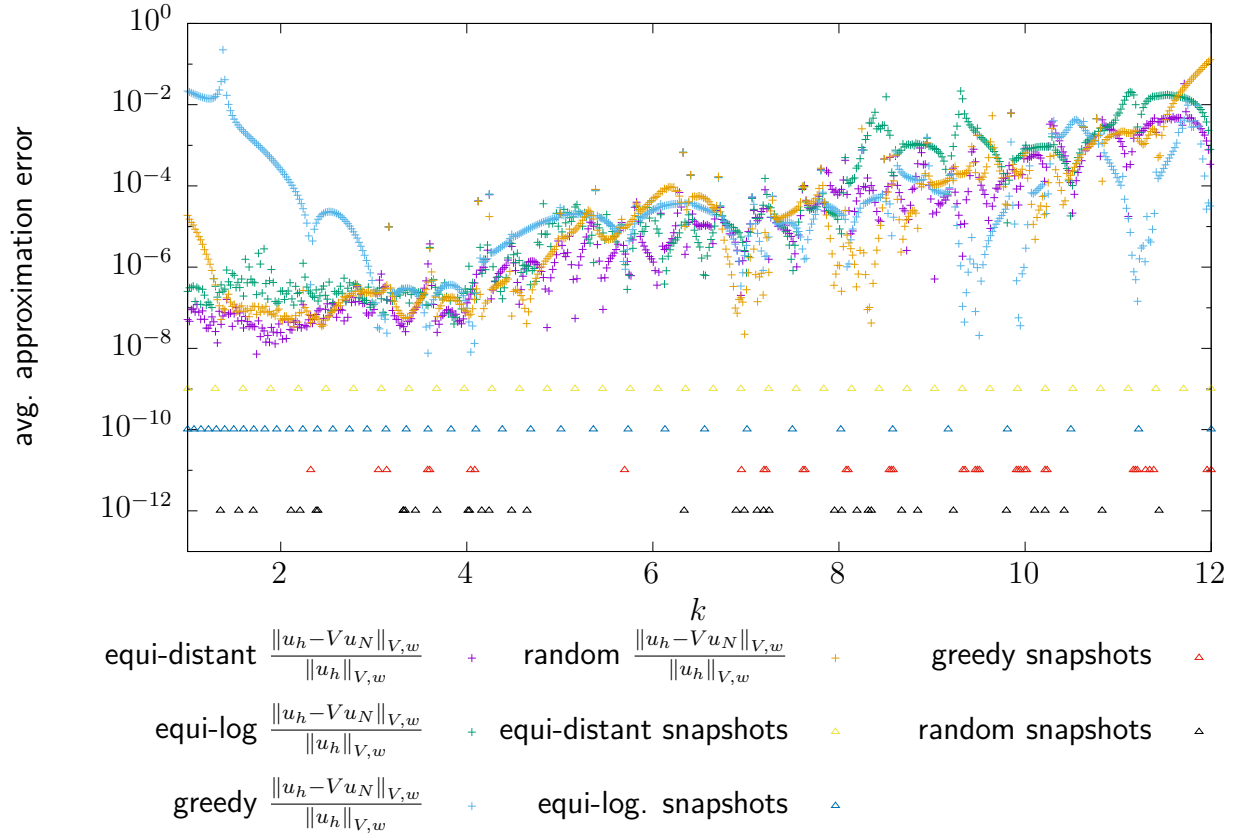
Figure 4.6: Comparison of the different construction strategies for RB spaces for the plane wave problem from Section 4.1. The approximation errors are marked by crosses. The snapshots are marked using triangles.
