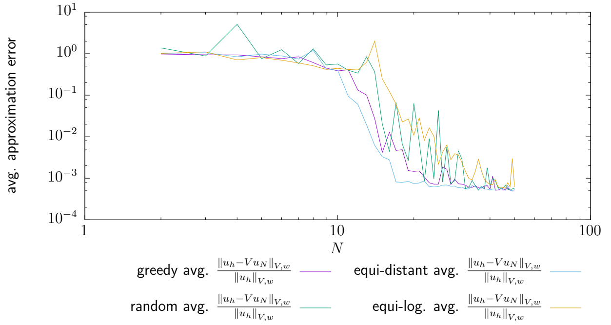
Figure 4.9: Convergence of RB spaces using different construction strategies using for the transmission/reflection problem (4.9).
