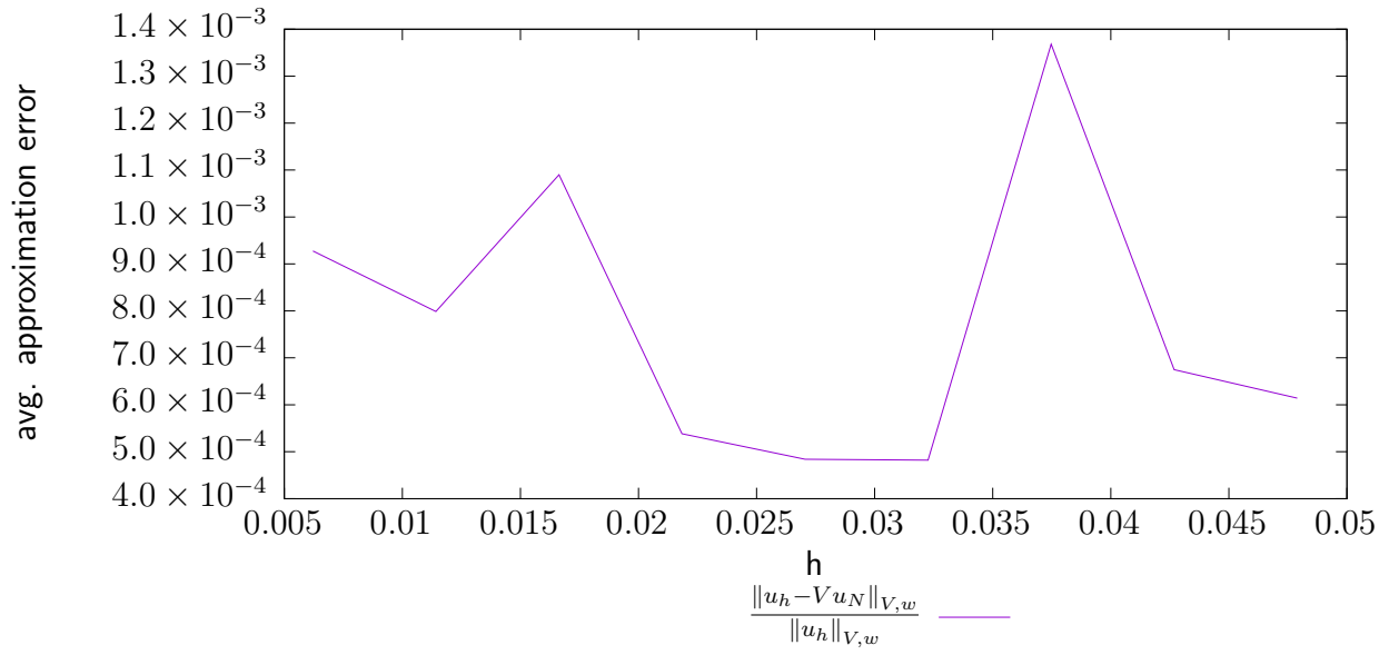
Figure 4.19: Average error for different RB spaces for the transmission/reflection problem (4.9). The RB spaces are constructed using training sets that are discretisations of the interval [1, 12] with step sizes h .
