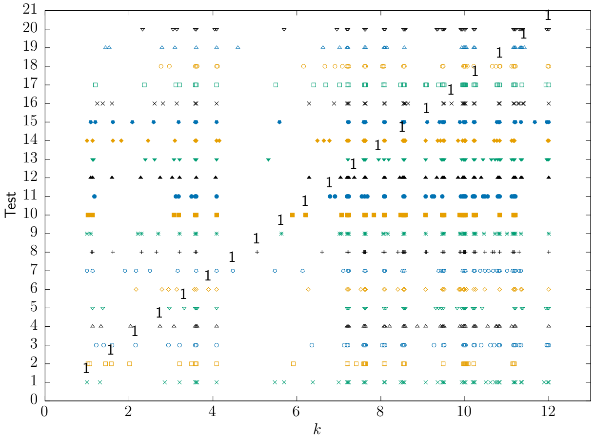
Figure 4.16: Snapshots selected by the greedy algorithm using different starting points for the plane wave problem from Section 4.1. The initial snapshot is marked by 1.
