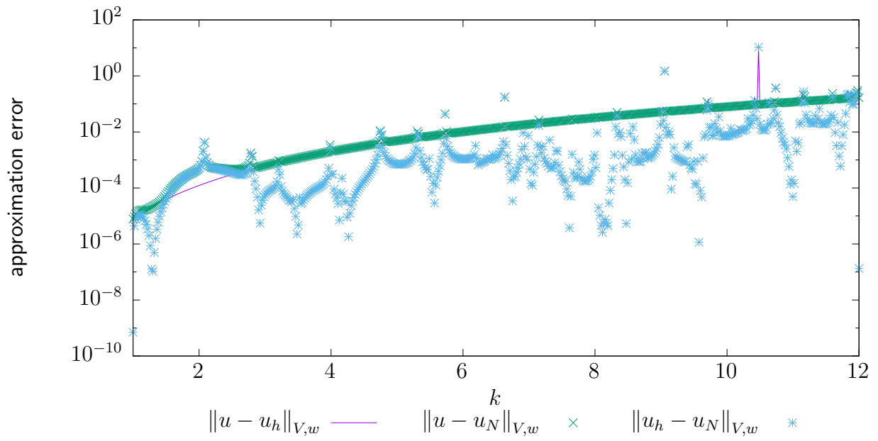
Figure 4.5: Error of solutions to problem (4.9).
