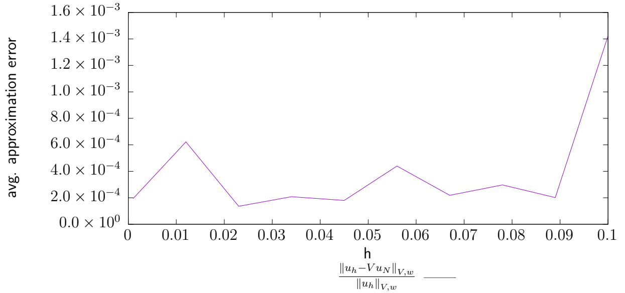
Figure 4.18: Average error for different RB spaces for the plane wave problem from Section 4.1. The RB spaces are constructed using training sets that are discretisations of the interval [1, 12] with differing step sizes h .
