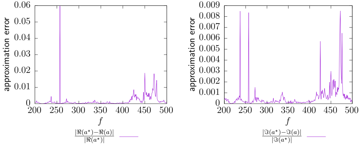
Figure 5.7: Error of the predicted admittance a for the admittance identification problem (5.7) at different frequencies. The exact solution is denoted by a^* .
