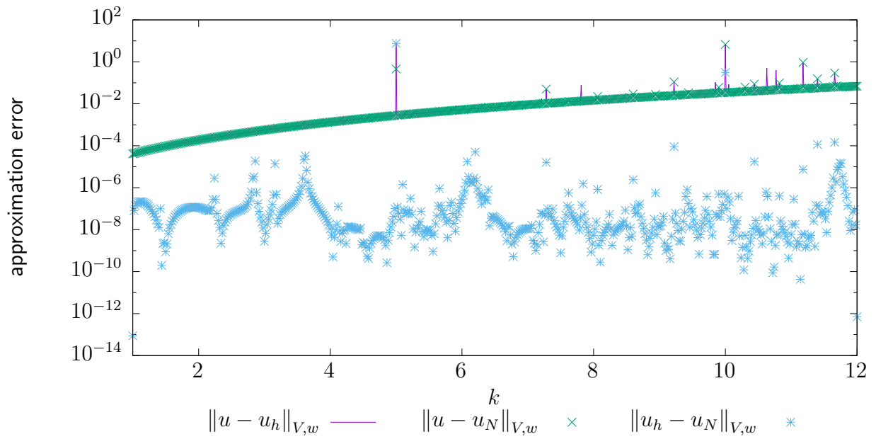
Figure 4.4: Error of solutions to the plane wave problem from Section 4.1.
