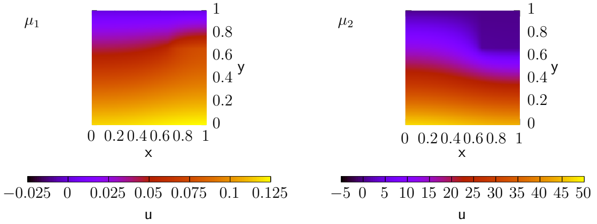
Figure 3.3: Two solutions to the thermal block problem for the parameter points \mu_1 and \mu_2 . \mu_1 = (0.633, 0.003, 0.919, 12.789, 1.368, 6.832, 712.252, 10.077) and \mu_2 = (0.049, 0.008, 35.889, 0.195, 4.427, 621.291, 252.26, 0.017)
