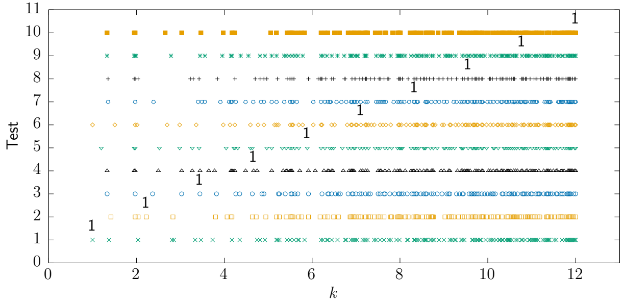
Figure 4.17: Snapshots computed by the greedy algorithm using different starting points for the transmission/reflection problem (4.9). The initial snapshot is marked by 1.
