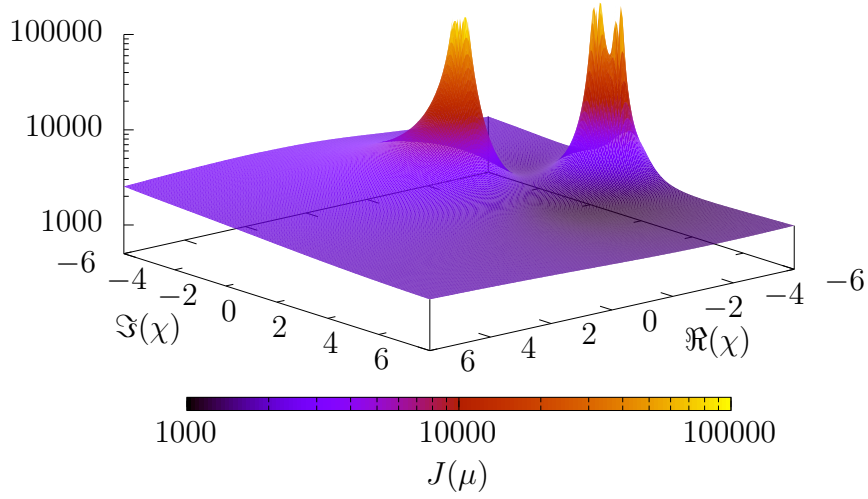
Figure 5.5: Value of the cost function J(\mu) defined in (5.24) for \mu = (2\pi, \chi) .
