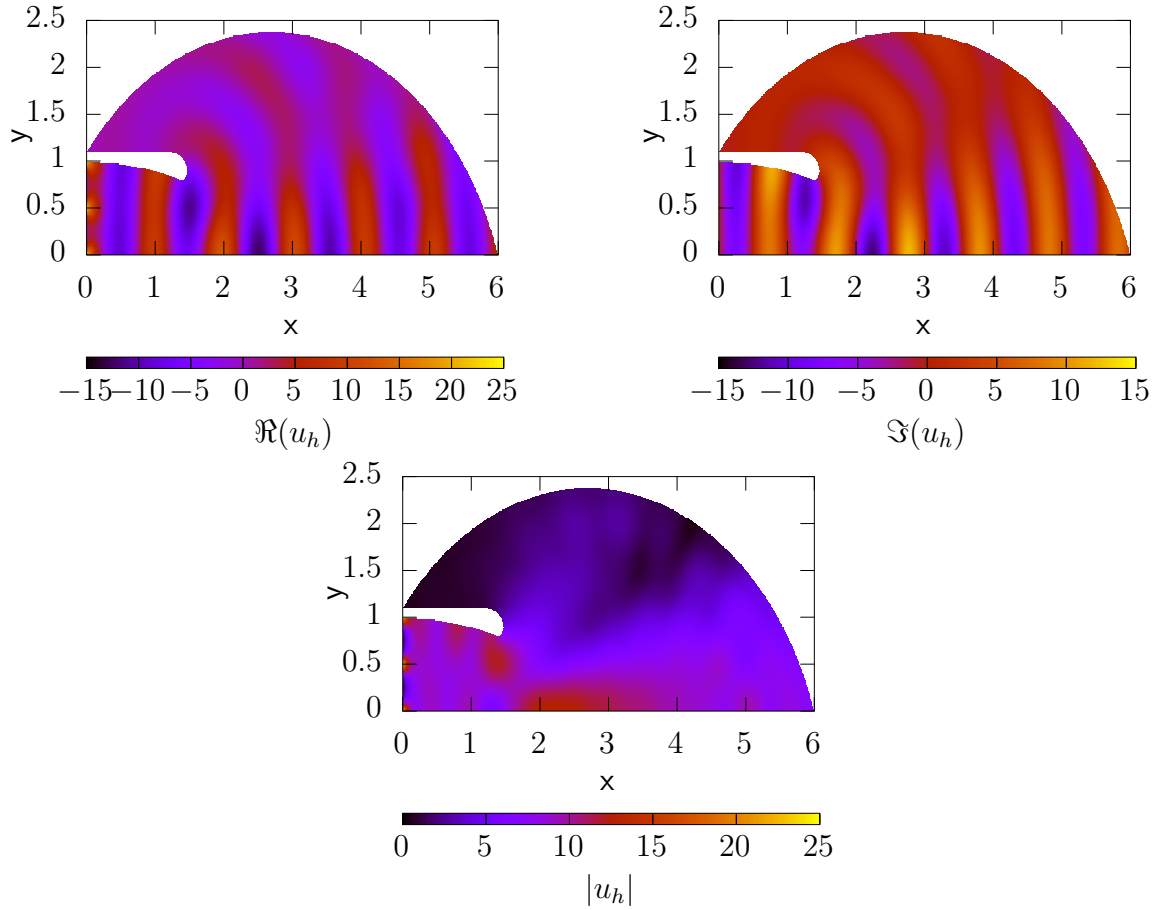
Figure 5.4: FE solution u_h to (5.21) for \chi = 0 and k = 2\pi .
