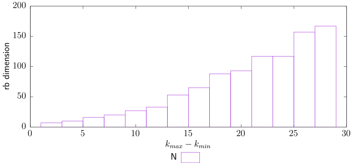
Figure 4.14: Dimensions of RB spaces depending on the interval length k_{max} - k_{min} for the plane wave problem from Section 4.1.
