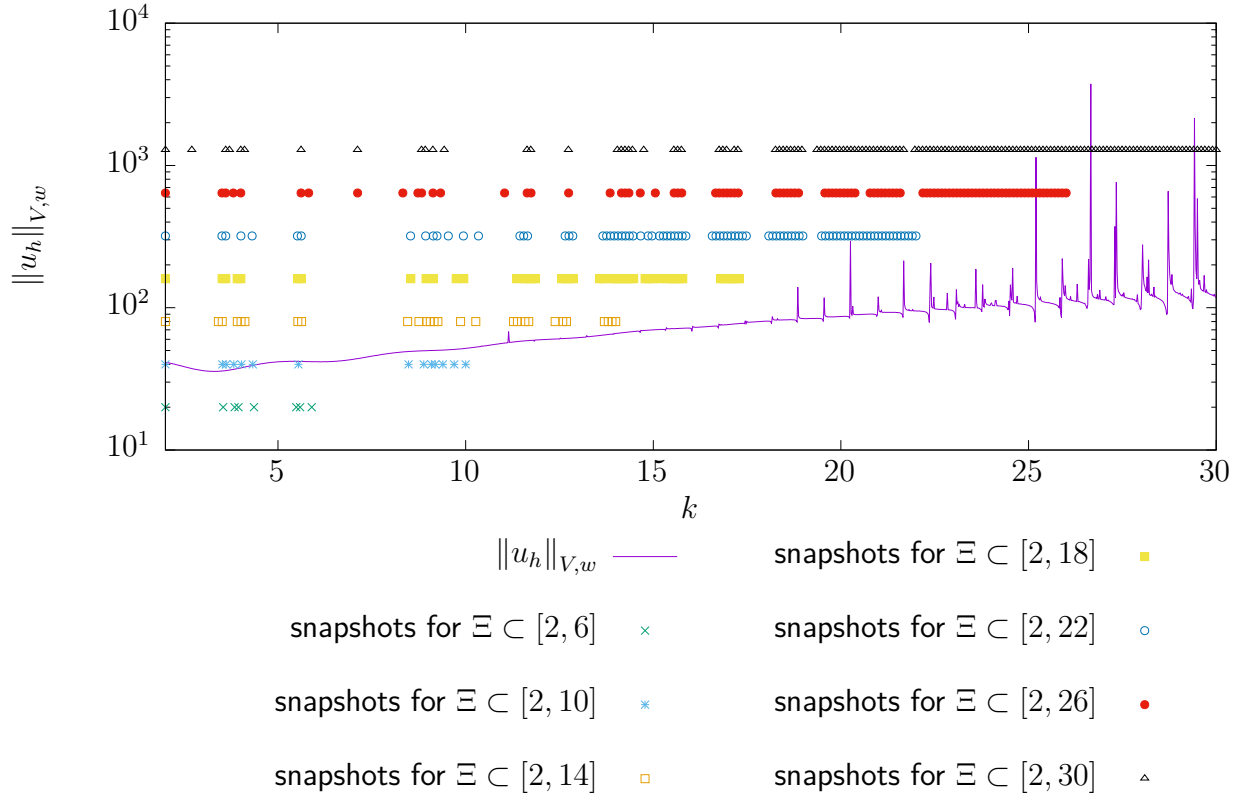
Figure 4.13: Selected snapshots to construct RB spaces for the transmission/reflection problem (4.9). The spaces are constructed using training sets \Xi taken from different intervals.
