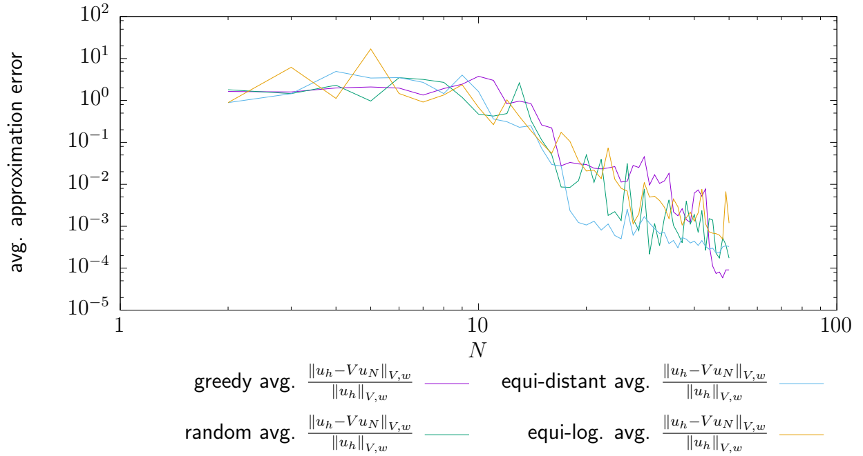
Figure 4.8: Convergence of RB spaces using different construction strategies for the plane wave problem from Section 4.1.
