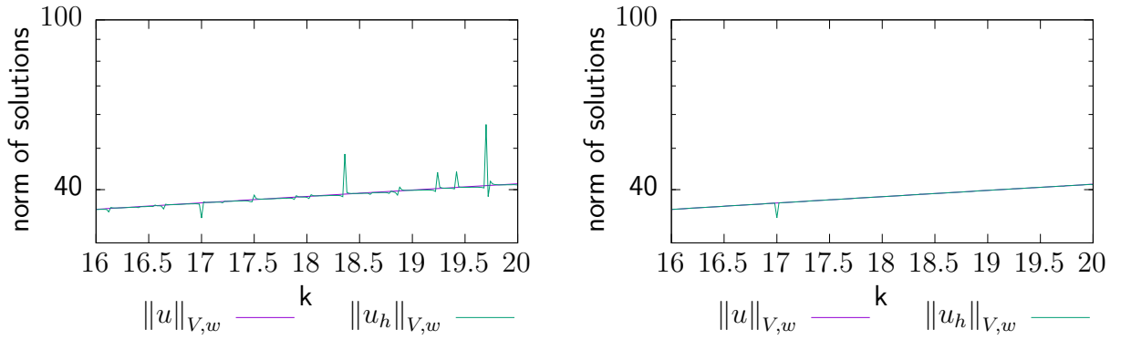
(a) Norm of solutions for a FE space with grid size h = 0.1 . (b) Norm of solutions for a FE space with grid size h = 0.05 .
