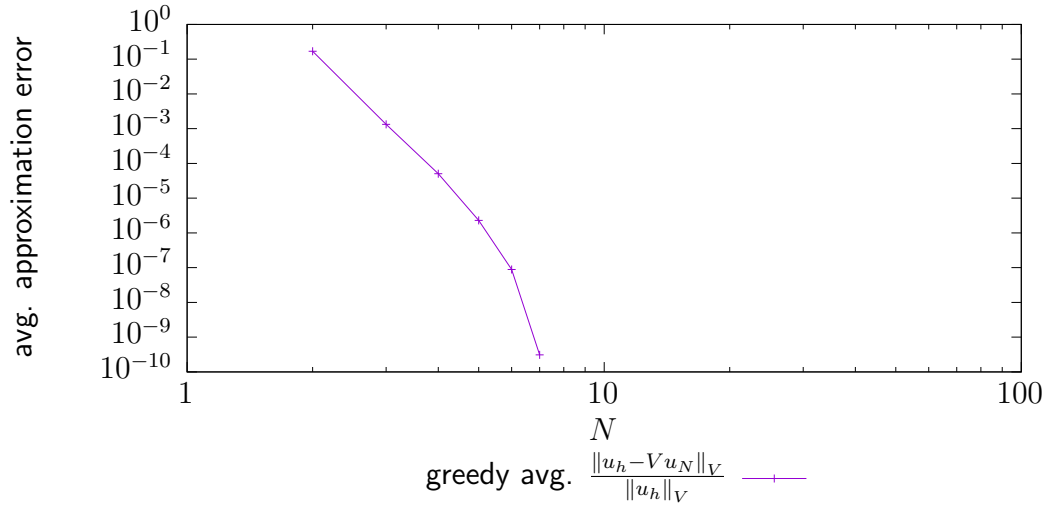
Figure 3.6: Average approximation error for the RBM using the greedy algorithm for problem (3.14).
