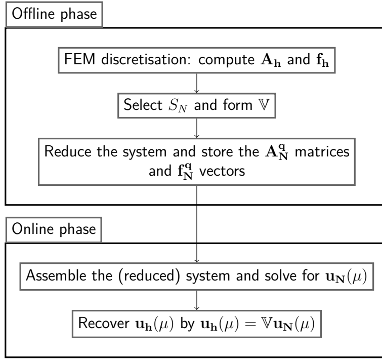
Figure 2.1: Overview of the offline-online phases. The (expensive) offline phase is only executed once, whereas the online phase is executed for every parameter point (\mu) of interest.
