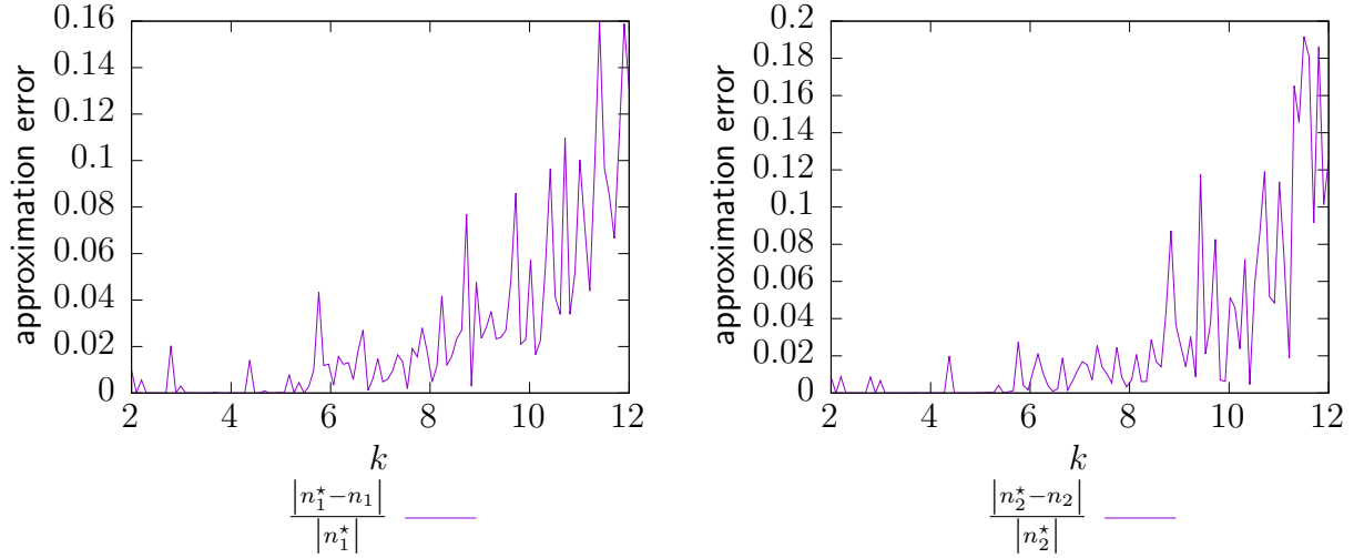
Figure 5.6: Error of the predicted values n_1 and n_2 for the inverse transmission/reflection problem from Section 5.1 at different wavenumbers. The exact solution is denoted by n_1^* and n_2^* .
