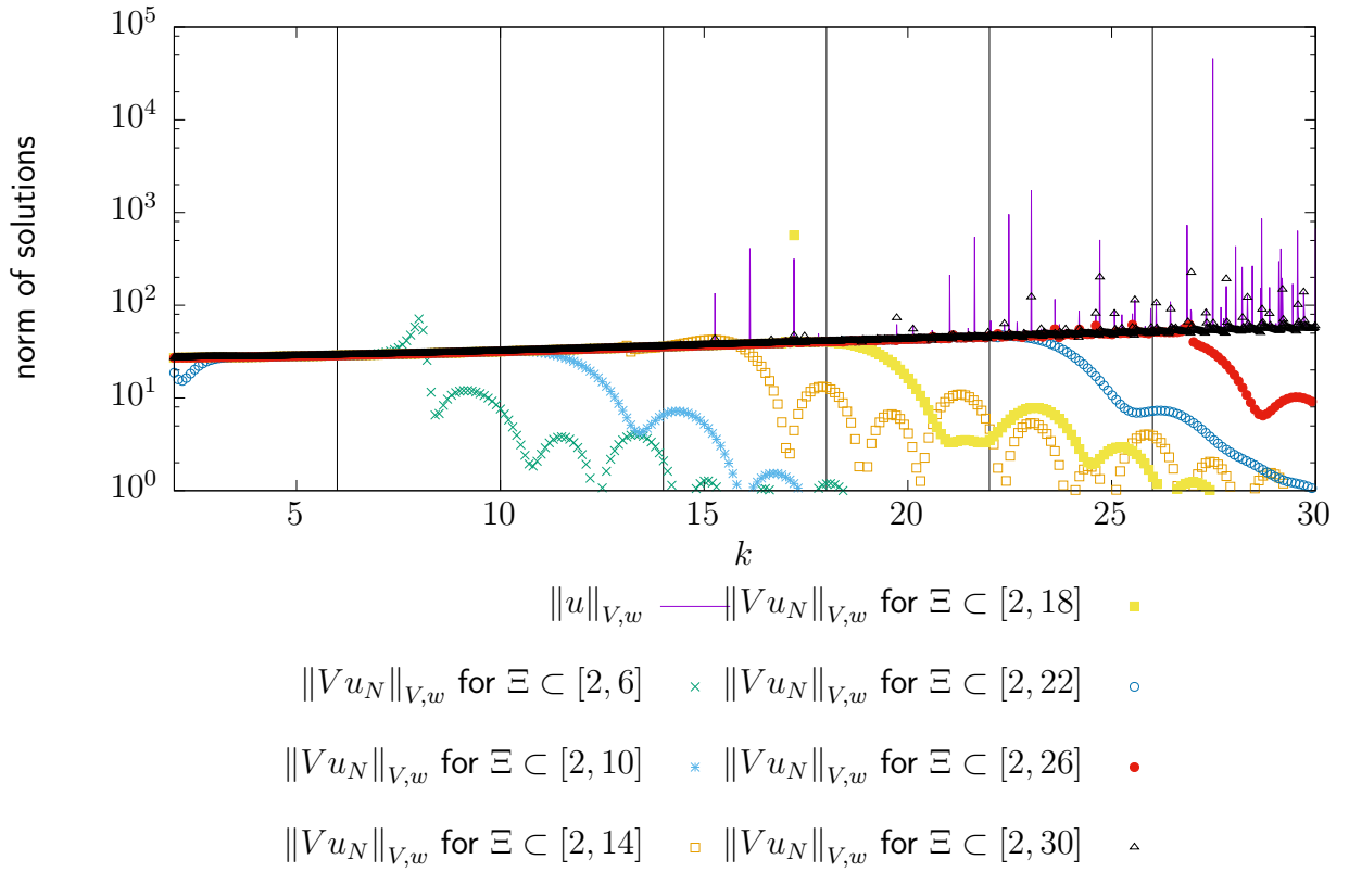
Figure 4.10: Comparison of different RB spaces for the plane wave problem from Section 4.1. The RB are constructed using training sets \Xi taken from different intervals.
