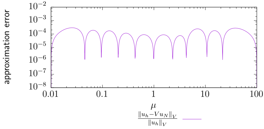
Figure 3.4: RB approximation error over the parameter space for the internal heat problem (3.9).
