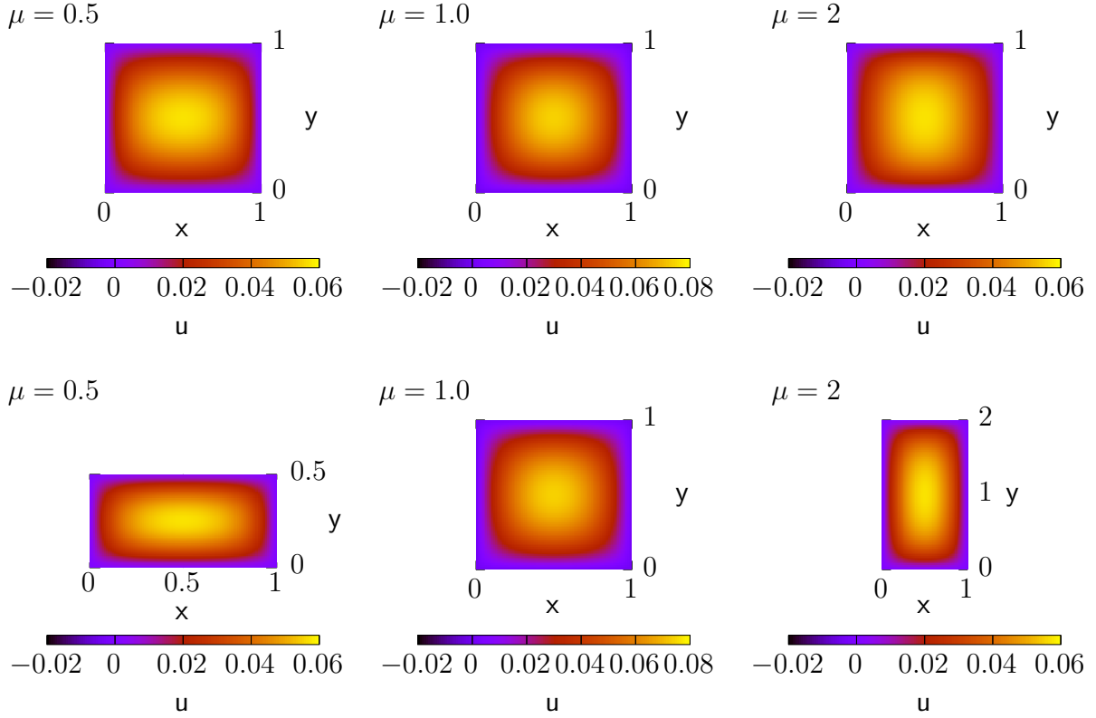
Figure 3.1: Solution to the internal heating problem for the parameter values \mu = 0.5 , \mu = 1 , and \mu = 2 . The first three figures show the solution in the reference domain \Omega . The last three in the original domain \Omega(\mu) .
