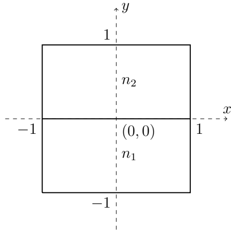
Figure 4.2: Domain of the transmission/reflection problem.
