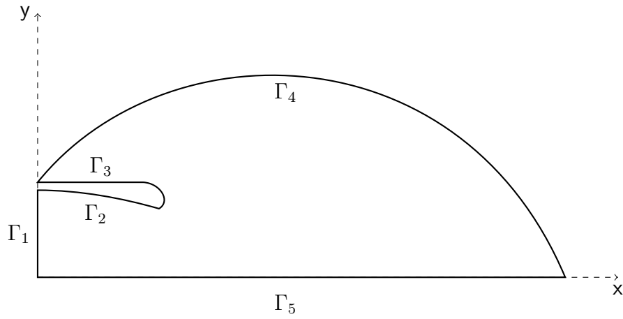
Figure 5.3: The domain and boundaries for problem (5.15).
