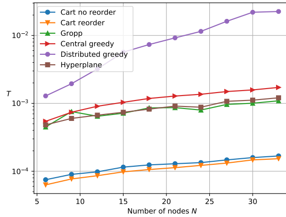
Figure 6.30: Instantiation time of different algorithms for the component stencil.
