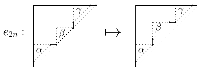
Figure 3.6: The action of e_{2n} on Young diagrams corresponding to noncrossing matchings of size n of the form (\alpha)\beta(\gamma) , where \alpha, \beta, \gamma are noncrossing matchings.
