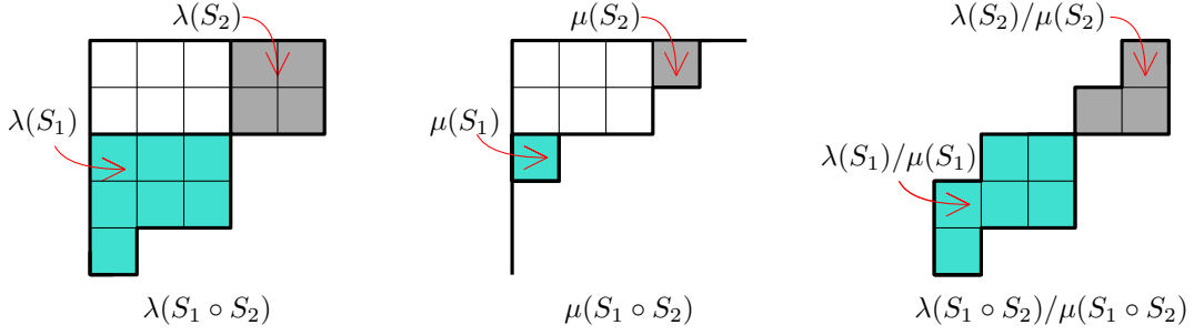
Figure 4.4: The (skew-shaped) Young diagrams corresponding to S_1 = \{-4, -2, -1, 0, 1, 3, 4\} , S_2 = \{-3, -1, 0, 1, 2\} and S_1 \circ S_2 .
