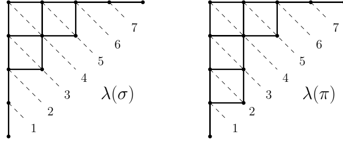
Figure 3.2: The matchings \sigma, \pi satisfy \sigma \nearrow_2 \pi .
