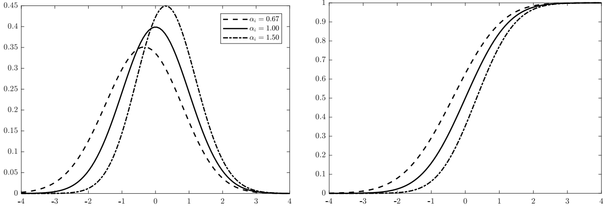
Figure 2.2. Density and distribution function of the normal distribution with \mu_i = 0 , s_i = 1 , and different levels of \alpha_i .
