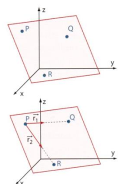
Abb.42: Parameterform
