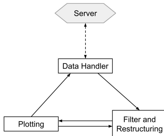
Figure 6.3: Component structure of the frontend JavaScript application
