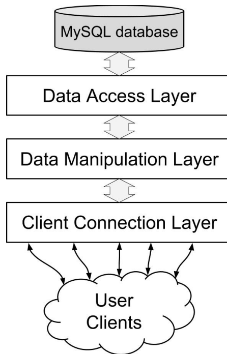
Figure 6.2: Layer structure of the Node.js backend server
