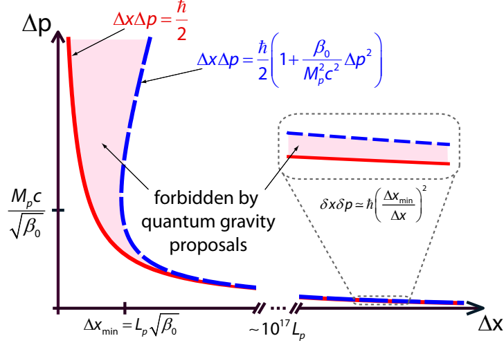
Figure 3.1: Reprint of a plot from Ref. [2]: The quantum mechanical minimum uncertainty given by eq. (3.2) as compared to the modified uncertainty, eq. (3.4). The modified uncertainty incorporates a minimal length scale \Delta x_{\min} = \sqrt{\beta_0} L_p , below which no quantum state can be prepared or read out. For \Delta x \gg \Delta x_{\min} the modified uncertainty principle is practically indistinguishable from the quantum mechanical prediction.
