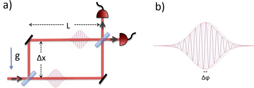
Figure 4.3: a) Schematic drawing of an interferometric setup where a photon travels in superposition at two different heights. The total area of the interferometer is A = L\Delta x . The Shapiro delay causes the amplitude on the lower paths to be delayed as compared to the upper path, given by eq. (4.32). If the delay \Delta t exceeds the pulse duration, the photon will not interfere. b) In the limit of very small delay as compared to the pulse length, the peak separation cannot be resolved and full interference is expected. However, the photon acquires a relative phase (dashed lines as compared to solid lines).
