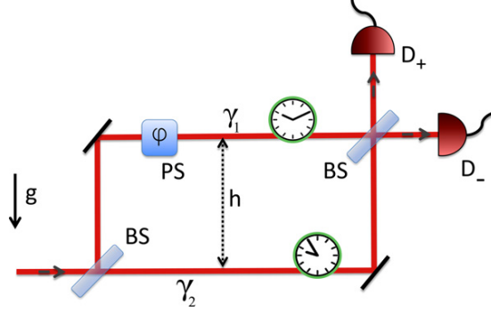
Figure 1. A Mach-Zehnder interferometer to measure the effect of general relativistic time dilation on a wavefunction of a single quantum system. The setup is placed in a homogeneous gravitational field ( g ) and it consists of two beam splitters (BS), two detectors D_{\pm} and the phase shifter (PS) which gives a controllable phase difference \varphi between the two trajectories \gamma_1 and \gamma_2 . The separation between the paths in the direction of the field is h . If the quantum particle that travels in superposition keeps track of time along its path, the visibility of the interference will be reduced since the which-way information becomes accessible due to the time dilation between the paths.
