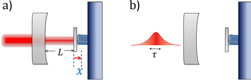
Figure 2.2: a) A typical opto-mechanical systems that consists of a one-sided cavity with a movable end mirror. The mirror is displaced by the light through radiation pressure, which in turn changes the resonance condition for the light. The interaction inside the cavity is governed by the Hamiltonian (2.1). b) In pulsed opto-mechanics an optical pulse of duration \tau is interacting with the mechanical mirror. The pulse duration is much shorter than the mechanical period. The Hamiltonian for pulsed opto-mechanics is given in eq. (2.3).
