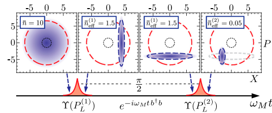
Fig. 3. Wigner functions of the mechanical state (above) at different times (indicated by arrows) during the experimental protocol (below). From left: Starting with an initial thermal state \tilde{n} = 10 , (this is chosen to ensure the figure dimensions are reasonable,) a pulsed measurement is made with \chi = 1.5 and outcome P_L^{(1)} = 4\chi obtained, which yields an X_M quadrature squeezed state. The mechanical state evolves into a P_M quadrature squeezed state following free harmonic evolution of 1/4 of a mechanical period prior to a second pulse with outcome P_L^{(2)} = -3\chi yielding the high-purity mechanical squeezed state. The effective thermal occupation of the mechanical states during the protocol is indicated. The final state's occupation can be reduced below unity even for large initial occupation, see Eq. 7 of the main text. Dashed lines indicate the 2\sigma -widths and the dotted lines show the ground state ( \tilde{n} = 0 ) for comparative purposes. The displacement \Omega is not shown.
