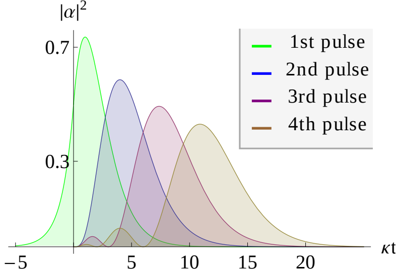
Figure 3.2: Change in the intra-cavity pulse shapes for the four subsequent interactions. An initial Lorentzian input pulse with \alpha_{in}(t) = \sqrt{\kappa}e^{-\kappa|t|} is broadened after entering and leaving the cavity. This effect can be minimized by using pulses of duration much larger than the cavity ring-down time.
