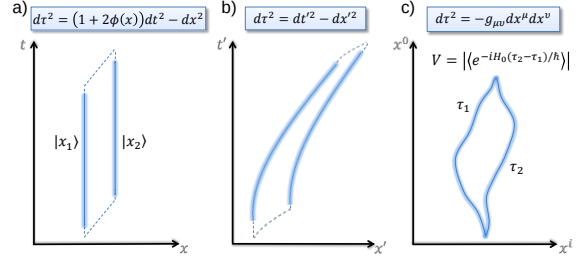
FIG. 2. A composite particle in superposition will decohere due to time dilation. The figure shows two superposed trajectories in different situations and space-times (here c=1 ). a) A particle in superposition at two different fixed heights above the earth, as considered in the main text (the dashed lines represent arbitrary small non-stationary contributions that would be necessary if one performs an interferometric experiment). The centre-of-mass will decohere after a time \tau_{dec} as given in eq. (4). In general, the full evolution of the centre-of-mass is given by eq. (5). b) A particle undergoing uniform acceleration g in flat space-time will experience the same time dilation and thus the same decoherence. Equivalently, the diagram describes the previous situation from the point of view of a freely-falling observer. c) A composite particle with internal Hamiltonian H_0 in an arbitrary space-time will decohere if the two superposed trajectories differ in proper time ( V is the interferometric visibility).
