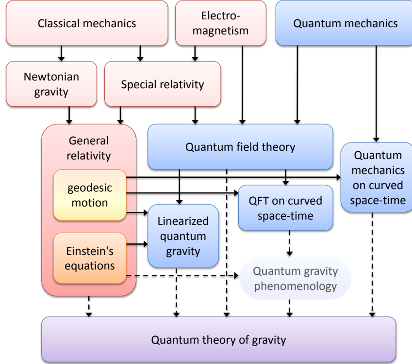
Figure 1.1: Schematic diagram of the development and unification of physical theories, inspired by Bronstein’s work [6, 7] and Okun’s cube of physical theories [8]. Classical theories are highlighted in red, while quantum theories are highlighted in blue. The arrows correspond to the development of the theories and dashed arrows represent currently unknown relations. For clarity, general relativity is shown to include two separate conceptual pillars: dynamics of physical systems on a background metric and dynamics of the metric itself (corresponding to eqs. (1.2) and (1.3), respectively). The former can be included into quantum theory, thus low-energy quantum mechanics and quantum field theory can be formulated on a fixed, possibly curved, background space-time. However, no complete theory of quantum gravity that includes quantization of gravity beyond the linear approximation is currently known. Quantum gravity phenomenology may allow for the possibility of testing possible aspects of quantum gravity by modelling some expected behaviour. The research focus in this thesis is on low-energy quantum systems (at non-relativistic velocities), which can be controlled with very high precision and which allow for tests of quantum theory at novel scales in terms of mass and size. It is shown that quantum mechanics in the presence of general relativistic time dilation, as well as possible quantum gravity phenomenology, can become accessible with such systems.
