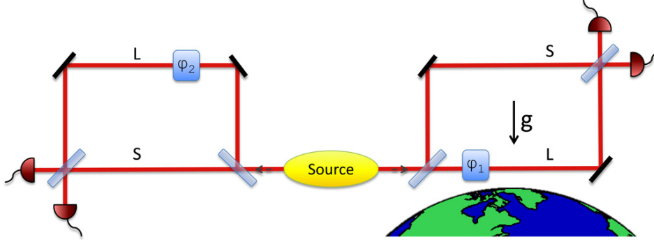
Figure 3. A Franson-type interferometer modified to test a local realistic description of photons undergoing gravitational time dilation. It consists of a source of photon pairs and two Mach–Zehnder setups with arms of different optical lengths S, L . On the right-hand side this difference is due to the general relativistic time dilation. This can be realized by utilizing a Mach–Zehnder setup as in figure 1, where the two paths of equal length are at different gravitational potentials, so that there will be a time dilation \Delta\tau between them. The Mach–Zehnder interferometer on the left-hand side is placed such that both arms feel the same gravitational potential and the difference in their lengths is L - S = c\Delta\tau . In each of the interferometers a controllable phase shift \phi_1, \phi_2 is induced in the optically longer arm. By varying those phases it is possible to violate Bell’s inequalities on a subsample of coincident detected photons.
