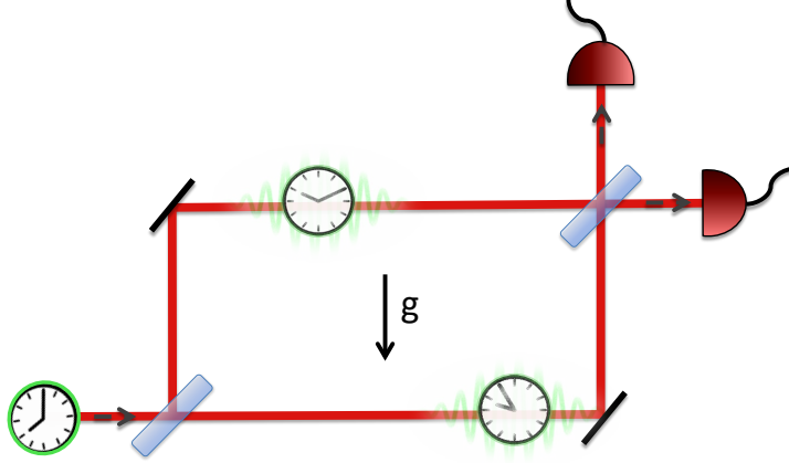
Figure 4.2: Schematic drawing of an interferometric setup where a matter wave with internal degrees of freedom is brought in superposition of two different heights. The matter-wave couples to gravity through the Hamiltonian (4.28), which captures time dilation. The internal degrees of freedom act as clocks. Thus, in addition to the relative phase as given in eq. (4.22), time dilation causes the wave function of the matter to become entangled to its internal clock states.
