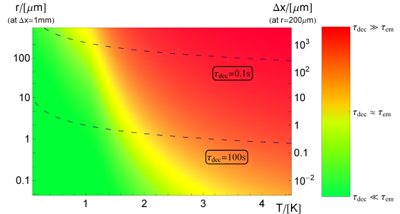
FIG. 3. Decoherence due to gravitational time dilation as compared to decoherence due to emission of thermal radiation for sapphire microspheres. In the green region time dilation is the dominant decoherence mechanism. The left axis shows various sphere radii r (corresponding to particle numbers N = 10^7 to N = 10^{18} ) for a fixed superposition size \Delta x , whereas the right axis shows various superposition sizes for a fixed particle radius. The dashed lines correspond to the respective time dilation decoherence timescales. Sapphire was chosen for its low emission at microwave frequencies.
