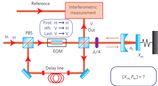
Figure 3 | Proposed experimental set-up to probe deformations of the canonical commutator of a macroscopic mechanical resonator. An incident pulse 'In' is transmitted through a polarizing beam splitter (PBS) and an electro-optic modulator (EOM) and then interacts with a mechanical resonator with position X_m via a cavity field a_L . The optical field is retro-reflected from the optomechanical system and then enters a delay line, during which time the mechanical resonator evolves for one quarter of a mechanical period. The optical pulse, now vertically polarized, is rotated by the EOM to be horizontally polarized and interacts again with the mechanical resonator. This is repeated for a total of four interactions, such that the canonical commutator of the resonator is mapped onto the optical field. Finally, the EOM does not rotate the polarization and the pulse exits in the mode labelled 'Out', where it is then measured interferometrically with respect to a reference field such that the commutator deformations can be determined with very high accuracy.
