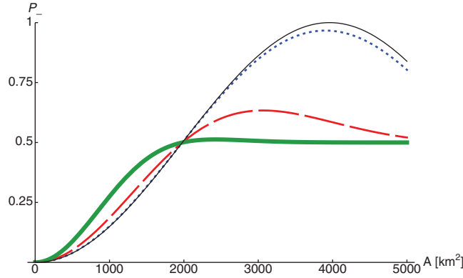
Figure 2. Probing the general relativistic slowdown of light in the proposed single photon interference experiments. The probabilities P_{J_{\sigma}^{-}}^{\nu_0} (equation (12)) to find the photon in the detector D_- are shown as a function of the area A [ \text{km}^2 ] of the interferometer in the vertical plane. The single-photon pulse has mean angular frequency \nu_0 \approx 4 \times 10^{15} Hz. The four graphs correspond to different widths \sigma of the wave packet and thus to different coherence times t_{\perp} = 2\sqrt{\sigma} : t_{\perp} = 0.05 fs (thick green line), t_{\perp} = 1 fs (red dashed line), t_{\perp} = 5 fs (blue dotted line) and t_{\perp} = \infty fs (black line), which is a limiting case of an infinitely long pulse (and thus with the clock effectively switched off). Observing a gravitational phase shift of a photon is within reach of current experimental capabilities.
