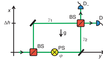
Figure 1 | Mach–Zehnder interferometer in the gravitational field.
