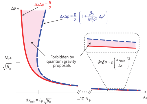
Figure 1 | The quantum uncertainty relation and a quantum gravitational modification. The minimum Heisenberg uncertainty (red curve) is plotted together with a modified uncertainty relation (dashed blue curve) with modification strength \beta_0 . M_P and L_P are the Planck mass and Planck length, respectively. The shaded region represents states that are allowed in regular quantum mechanics but are forbidden in theories of quantum gravity that modify the uncertainty relation. The inset shows the two curves far from the Planck scale at typical experimental position uncertainties \Delta x \gg \Delta x_{\min} . An experimental precision of \delta x \delta p is required to distinguish the two curves, which is beyond experimental possibilities at present. However, this can be overcome by our scheme, which allows one to probe the underlying commutation relation in massive mechanical oscillators and its quantum gravitational modifications.
