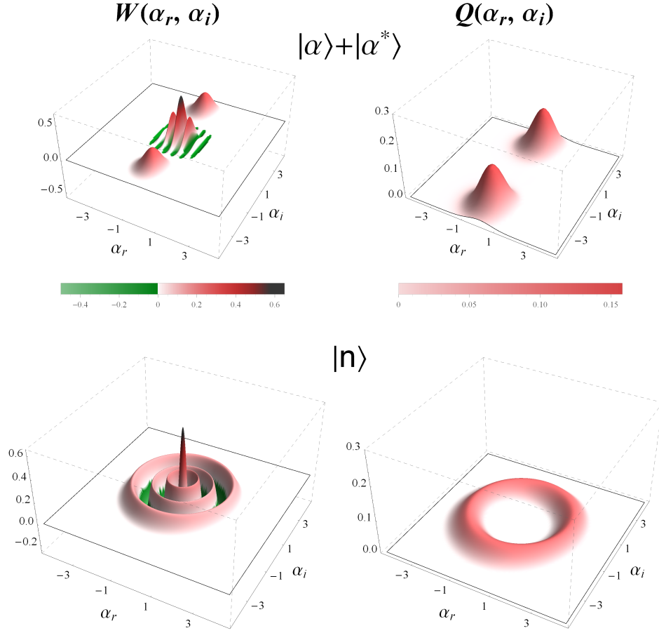
Figure 2.3: Comparison between the Wigner function (left) and the Husimi-Q-function (right) for two different states. The upper row shows the normalized superposition state |\alpha\rangle + |\alpha^*\rangle with \alpha = i3 [82, 83]. The lower row shows the Fock state |n\rangle with n = 6 [72, 74]. While the Wigner function can have negative values, the Q-function remains always positive. Since quasi-probability distributions are interrelated by convolution, see eq. (2.11), the Q-function smooths all features of the state as compared to the Wigner function. However, both distributions can be used to describe any quantum state.
