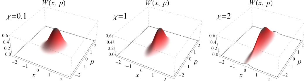
Figure 2.4: Wigner function of the mechanical state after a pulsed sequence. An initial coherent state becomes squeezed and displaced (the displacement is not shown here), see eq. (2.42). For interaction strength \chi = 0.1 , the state is practically indistinguishable from a coherent state. For \chi = 1 , the variance in the X_m -quadrature becomes \Delta X_m^2 = 1/4 . The squeezing grows with increasing \chi and is independent of the measurement outcome P_L .
