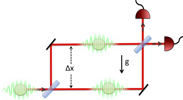
Figure 4.1: Schematic drawing of an interferometric setup where a particle is brought in superposition of two different heights. The matter-wave is coherently split on a beam splitter and the two amplitudes of the wave function evolve under the Newtonian gravitational potential (4.21). During the time spent at two different heights (with height difference \Delta x ), the system acquires a relative phase as given in eq. (4.22). In the first experimental implementation [167], a neutron beam was coherently split using Bragg reflection from Si-crystals. The total area of the interferometer was 6 \text{ cm}^2 and the neutrons were counted at the output ports using ^3\text{He} -detectors, confirming the gravitationally-induced relative phase of the wave function.
