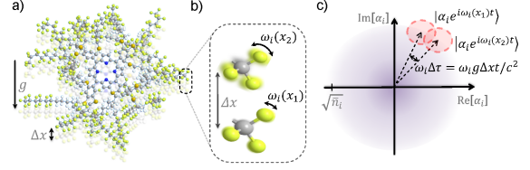
FIG. 1. Gravitational time dilation causes decoherence of composite quantum systems. a) Illustration of a TPPF20 molecule which has recently been used for matter-wave interference [5]. Here we illustrate a vertical superposition of size \Delta x in Earth's gravitational potential \Phi(x) = gx . b) The frequencies \omega_i of internal oscillations get red-shifted in the gravitational field, i.e. \omega_i \rightarrow \omega_i(1 + gx/c^2) . The internal oscillations entangle to the centre-of-mass position of the molecule. c) Phase-space representation of the i -th constituent which is in a thermal state with average occupation \bar{n}_i \approx k_B T / \hbar \omega_i . In the coherent state representation, the frequency of each coherent state depends on the position of the molecule and the internal states corresponding to the two superposition amplitudes evolve differently by an amount \omega_i \Delta \tau . Even for small time-dilations, this causes decoherence of the molecule with N constituents after a time \tau_{dec} , given in eq. (4).
