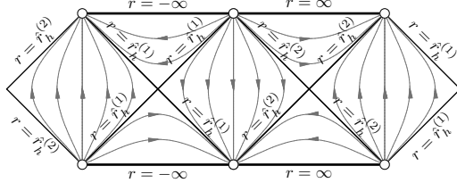
Figure 3.9: The conformal diagram for \theta \in (0, \pi) , with \theta \neq \frac{\pi}{2} , and \Delta_\theta \sin^2(\theta) small enough so that \hat{\Delta}_r always has two zeros.
