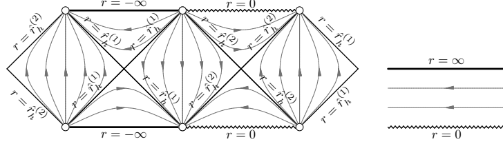
(a) The case \hat{r}_h^{(1)} < \hat{r}_h^{(2)} < 0 , with the left diagram showing r < 0 and the right diagram r > 0 .
