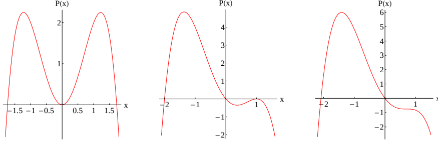
Figure 2.1: The function P(x) of (2.26) with \gamma = 0 when \beta = 0 (left plot), \beta = 1 (middle plot), and \beta = \sqrt{2} (right plot).
