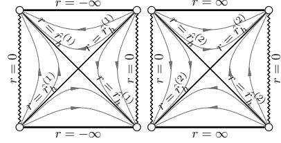
(c) The case \hat{r}_h^{(1)} < 0 < \hat{r}_h^{(2)} .
