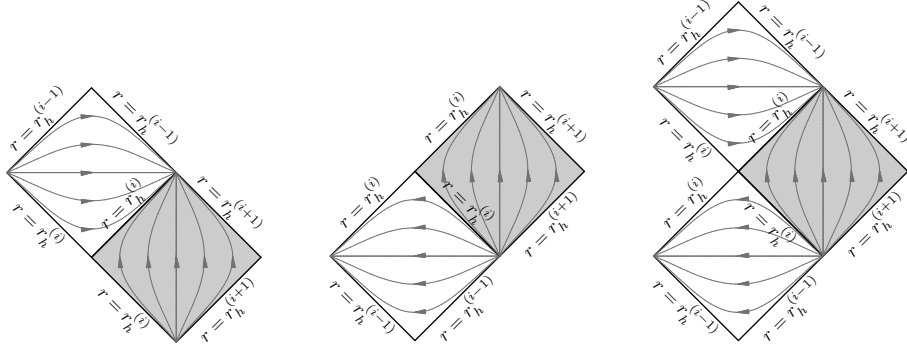
Figure 3.2: The two Eddington-Finkelstein-like extensions of the region (r_h^{(i)}, r_h^{(i+1)}) where F(r) > 0 , with the original region shaded in grey, and the resulting patch when gluing along the grey region. Note that only the interior of the diagrams is included.
