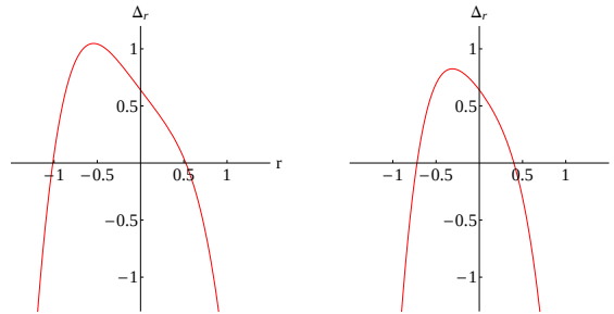
Figure 2.3: The function \Delta_r with m = 0.5 , a = 0.8 and \Lambda a^2 = 3 (left plot) or \Lambda a^2 = 6 (right plot).
