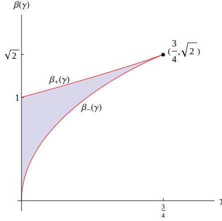
Figure 2.2: In the shaded region between the graphs, P(x) has four simple zeros. Two of them merge to x_h^{(1)} < x_h^{(2)} < x_h^{(3)} = x_h^{(4)} on \beta_+ and to x_h^{(1)} < x_h^{(2)} = x_h^{(3)} < x_h^{(4)} on \beta_- , all three positive zeros merge at the point (3/4, \sqrt{2}) , which leads to a triple and a simple zero there. In the unshaded region outside the graphs there always are two simple zeros.
