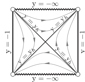
FIG. 13. The projection diagram for the Emparan-Reall black rings. The arrows indicate the causal character of the orbits of the isometry group. The boundary y = -1 is covered, via the projection map, by the axis of rotation and by spatial infinity i^0 . Curves approaching the conformal null infinities I^\pm asymptote to the missing corners in the diagram.
