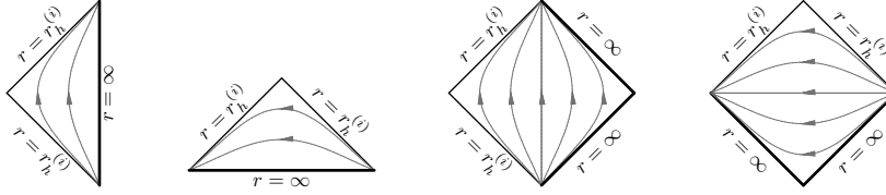
Figure 3.5: Conformal diagrams of blocks with r \in (r_h^{(i)}, \infty) . The first two diagrams show the case where I(r) approaches a finite constant value for r \rightarrow \infty , with F > 0 on the far left, and F < 0 next to it. The second pair of figures show the case where I(r) becomes unbounded for r \rightarrow \infty , again with the first diagram showing F > 0 and the second one F < 0 . A priori only the interior of the diagram is included, the strong lines indicating conformal infinities can be added separately, however still leaving out the corners.
