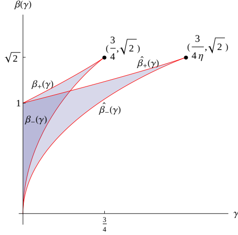
Figure 3.6: \beta_{\pm} and \hat{\beta}_{\pm} with \eta > 0 , here assuming \eta = 0.5 , are shown as a function of \gamma > 0 . The grey shading between \beta_{\pm} and \hat{\beta}_{\pm} , as well as between \hat{\beta}_{\pm} and \hat{\beta}_{\pm} , indicates the existence of four zeros of \Delta_r and \hat{\Delta}_r respectively. In the region where they intersect, indicated by a darker shading, as well as in the white regions where both \Delta_r and \hat{\Delta}_r have two zeros, the global structure is correctly represented by the conformal diagram.
