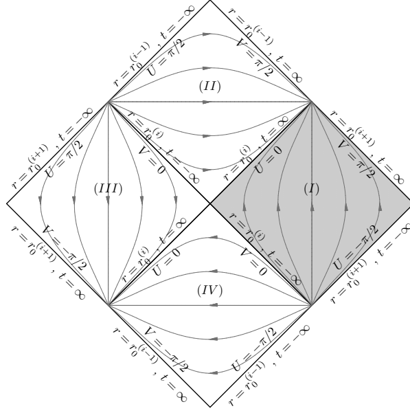
Figure 3.3: The region (r_h^{(i)}, r_h^{(i+1)}) , extended over the horizon at r_h^{(i)} by Kruskal-Szekeres-like transformation. The original unextended region is shaded. When using Eddington-Finkelstein-like coordinates only, the center point has to be removed. Note that only the interior of diagram is included.
