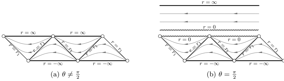
Figure 3.8: The conformal diagrams for \theta \in (0, \pi) and \Delta_\theta \sin^2(\theta) large enough so that \hat{\Delta}_r has one zero of order two at r_1 , where it's global maximum is located. While the strong lines indicate conformally smooth infinities that are part of the diagram, the circles indicate points that are excluded.
