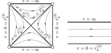
(b) The case \hat{r}_h^{(1)} < \hat{r}_h^{(2)} = 0 , with the left diagram showing r < 0 and the right diagram r > 0 .
