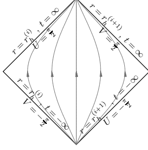
Figure 3.1: The region (r_h^{(i)}, r_h^{(i+1)}) and F(r) > 0 in manifestly conformally flat coordinates (X, T) , with T increasing vertically. The arrows indicate the orbits of the Killing vector field \partial_t , pointing in direction of increasing t .
