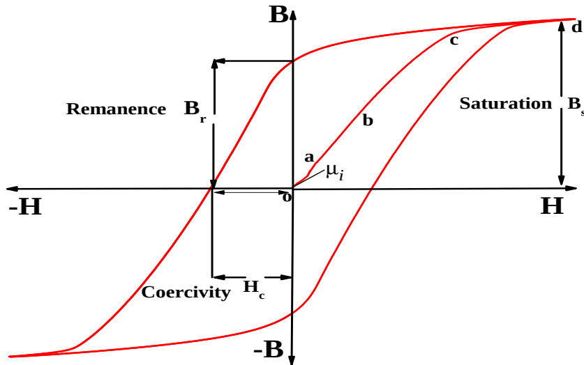
Figure 1.3: Hysteresis loop of ferromagnetic materials.
