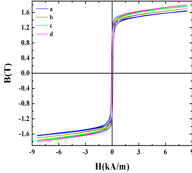
Figure 2.4: Hysteresis loops at different configurations of windings. "a", "b", "c", "d", corresponds to the different configurations mentioned in text.
