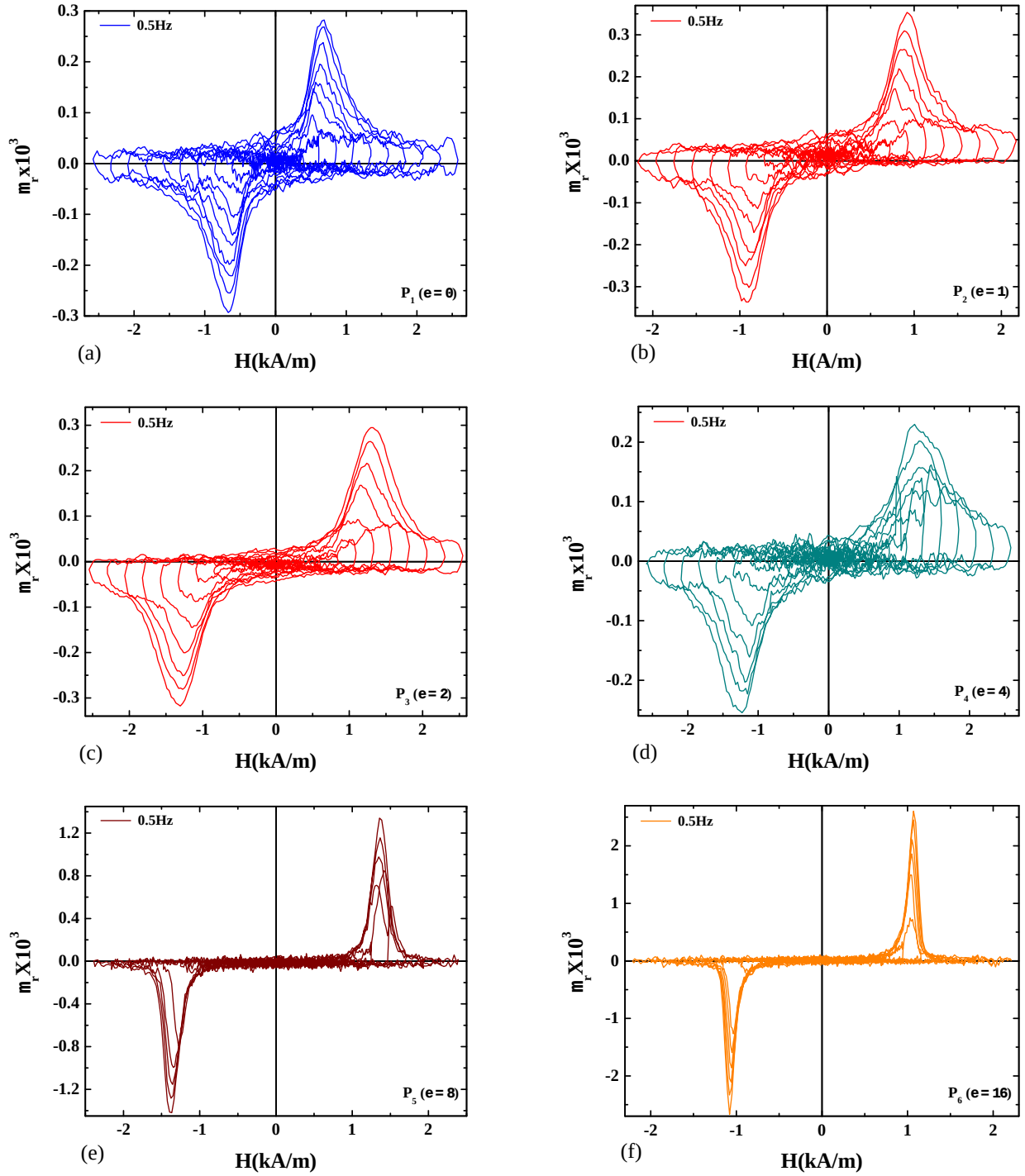
Figure 6.4: Relative permeability versus the field of SPD treated pearlitic steel (R260) (a) P_1(\epsilon=0) , (b) P_2(\epsilon=1) , (c) P_3(\epsilon=2) , (d) P_4(\epsilon=4) , (e) P_5(\epsilon=8) and (f) P_6(\epsilon=16) .
