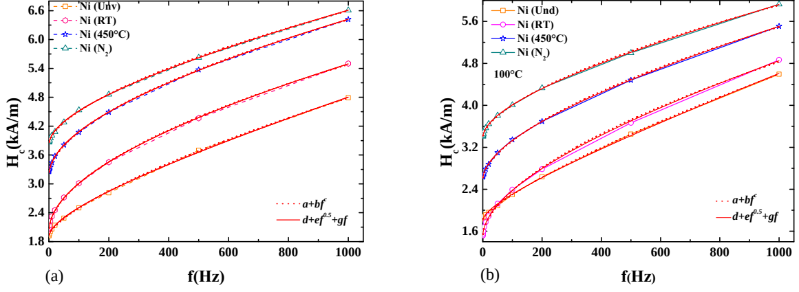
Figure 4.26: (a) Fitting frequency dependent coercivity for HPT-Treated Ni by Eq. 4.3 and 4.4 (a) at room temperature and (b) 100°C (373 K).
