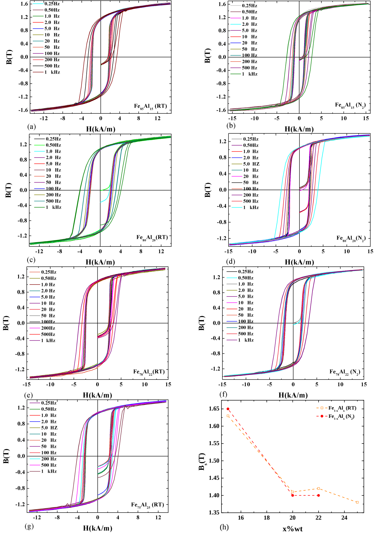
Figure 5.1: Hysteresis loops of HPT-treated Fe-Al system (a) \text{Fe}_{85}\text{Al}_{15} (RT), (b) \text{Fe}_{85}\text{Al}_{15} ( \text{N}_2 ), (c) \text{Fe}_{80}\text{Al}_{20} (RT), (d) \text{Fe}_{80}\text{Al}_{20} ( \text{N}_2 ), (e) \text{Fe}_{78}\text{Al}_{22} (RT), (f) \text{Fe}_{78}\text{Al}_{22} ( \text{N}_2 ), (g) \text{Fe}_{75}\text{Al}_{25} (RT) and (h) Magnetization as a function of Al concentration.
