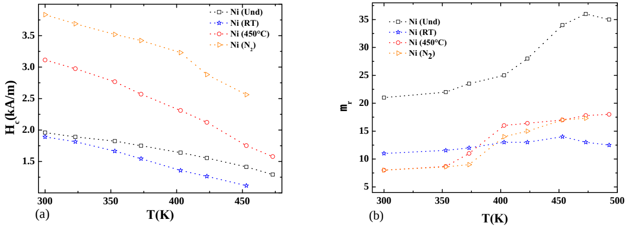
Figure 4.25: Temperature dependent (a) coercivity H_c(T) , (b) Relative permeability of HPT-Treated Ni .
