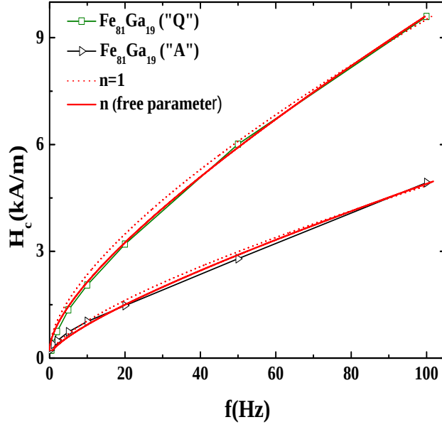
Figure 5.13: Fitting applying model Eq. 5.12 on the experimental data of the coercivity versus frequency of \text{Fe}_{81}\text{Ga}_{19} (Q) and (A).
