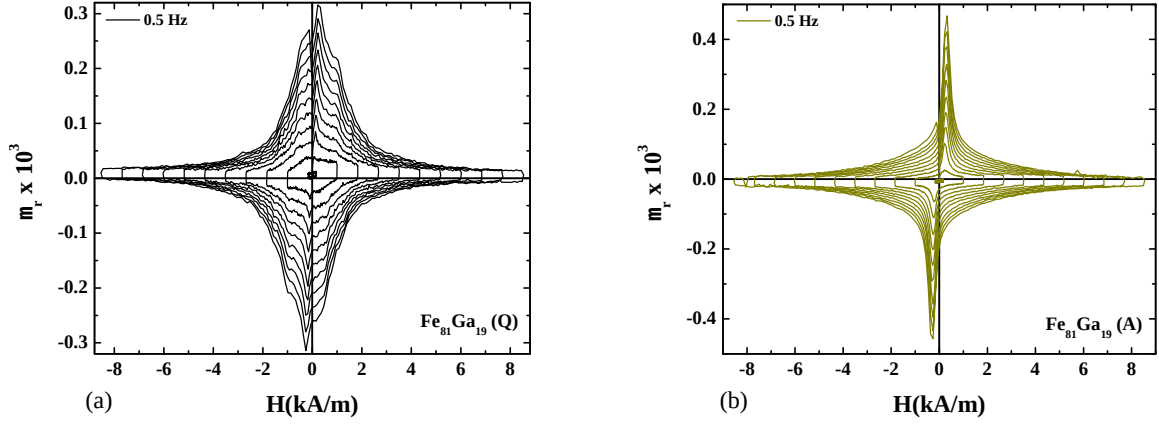
Figure 5.10: Relative permeability versus the field at room temperature measured at 0.5 Hz of \text{Fe}_{81}\text{Ga}_{19} (a) quenched (Q) and (b) annealed (A) samples.
