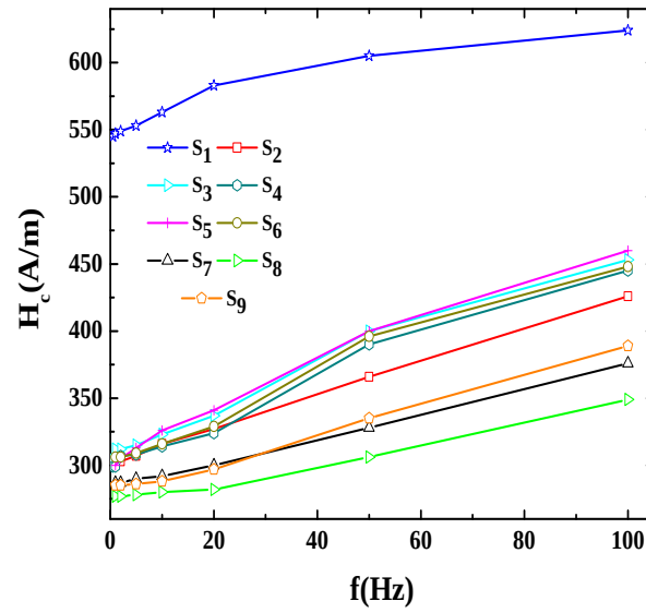
Figure 8.8: Coercivity versus frequency of resin coated Fe-Powder.
