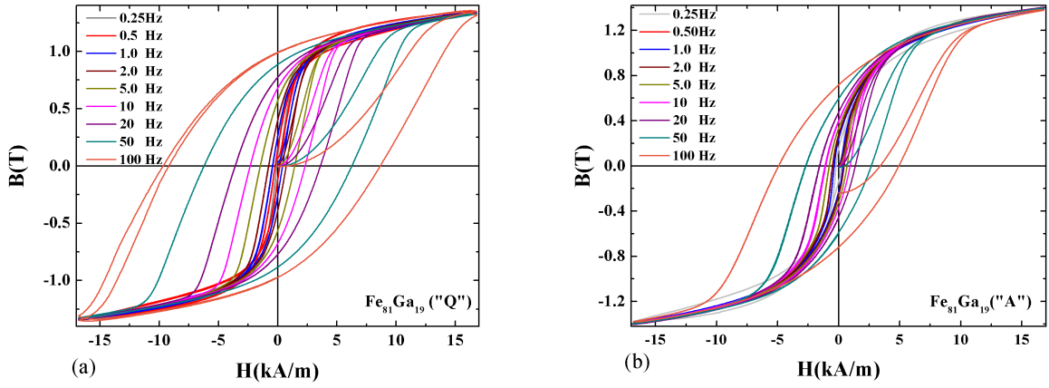
Figure 5.8: Hysteresis loop of Fe_{81}Ga_{19} measured at different frequencies: (a) on quenched (Q) and (b) on annealed (A) at room temperature.
