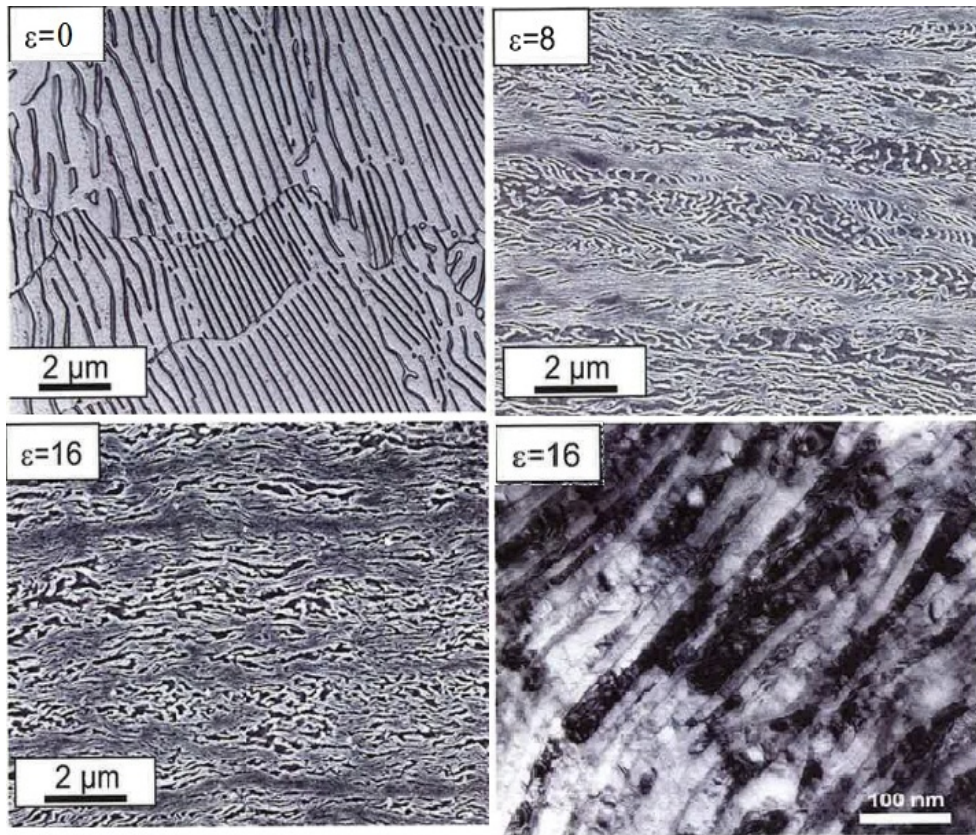
Figure 6.1: Microstructure photographs of SPD treated pearlitic steel (R260).
