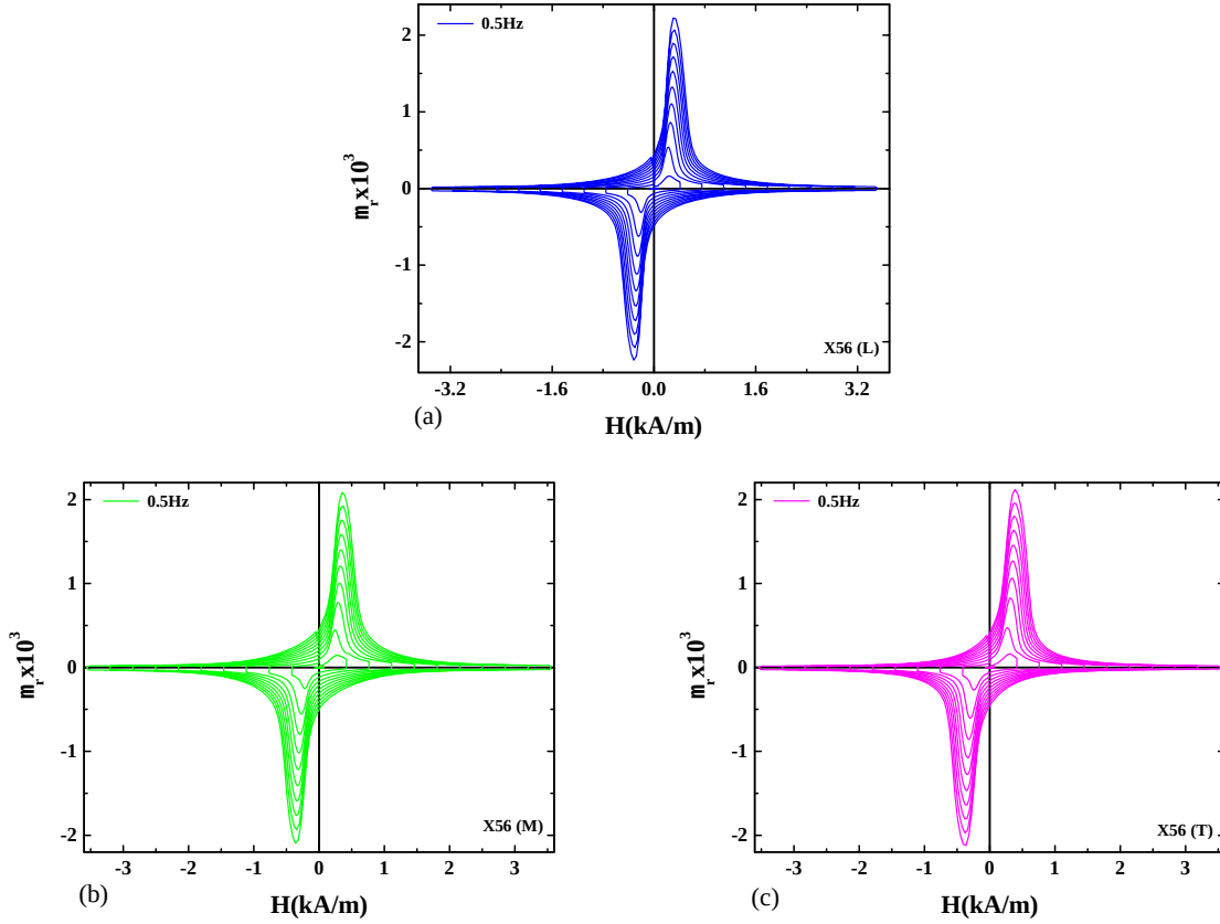
Figure 7.7: Relative permeability \mu_r versus field H(t) for pipeline steel X56 (a) X56 (L), (b) X56 (M) and (c) X56 (T).
