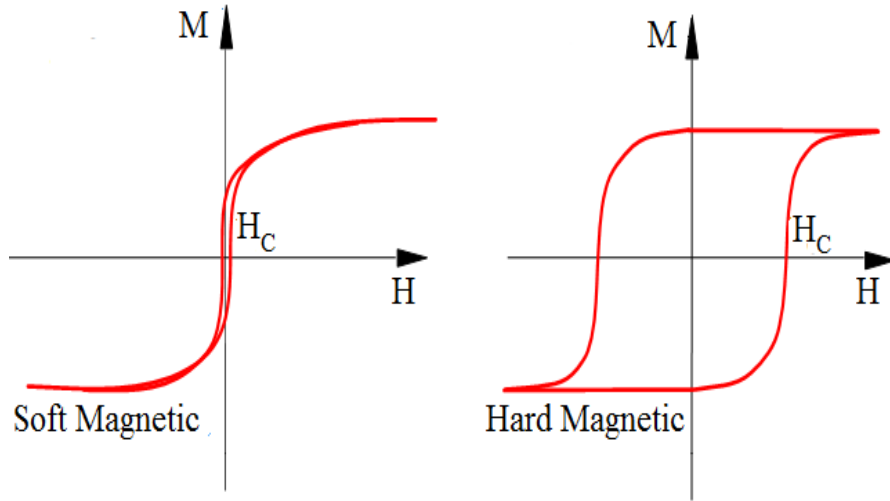
Figure 1.2: A magnetic hysteresis loop for soft and hard ferromagnetic materials.
