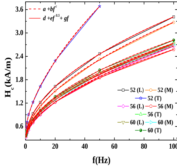
Figure 7.9: fit according to Eqs.3.16 and 3.17 on coercivity versus frequency of X52, X56, and X60 steel pipeline samples.
