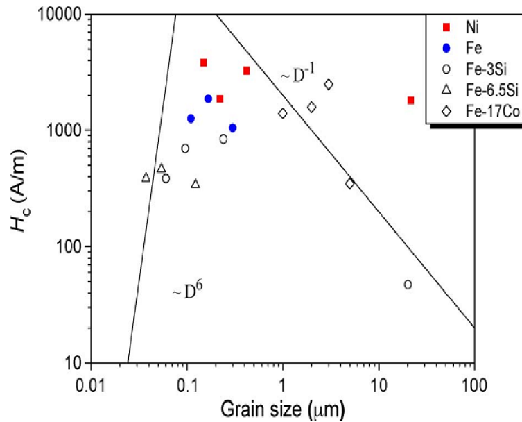
Figure 4.9: Coercivity as a function of the grain size ( D ) for Fe, Fe-3 wt%Si, Fe-6.5 wt%Si, Fe-17 wt%Co and Ni, after HPT-deformation [5].
