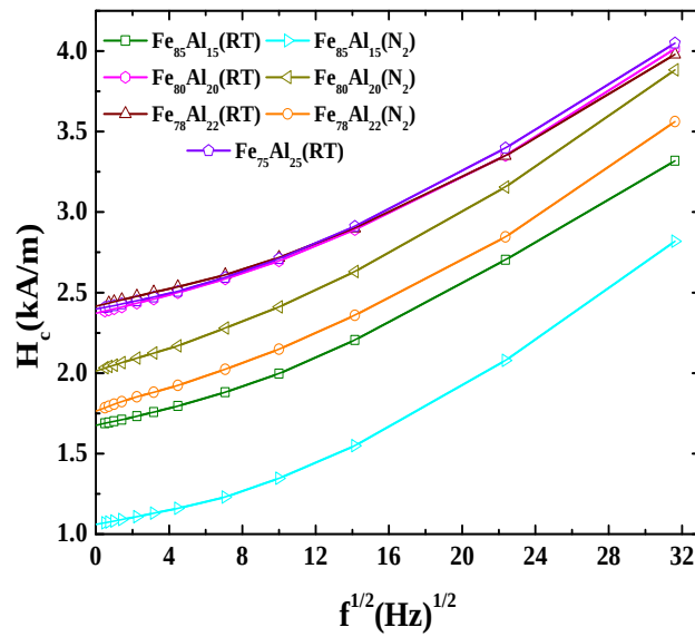
Figure 5.2: Coercivity versus square root of frequency of HPT-treated \text{Fe}_{100-x}\text{Al}_x ( x = 15 \leq x \leq 25 ) samples.
