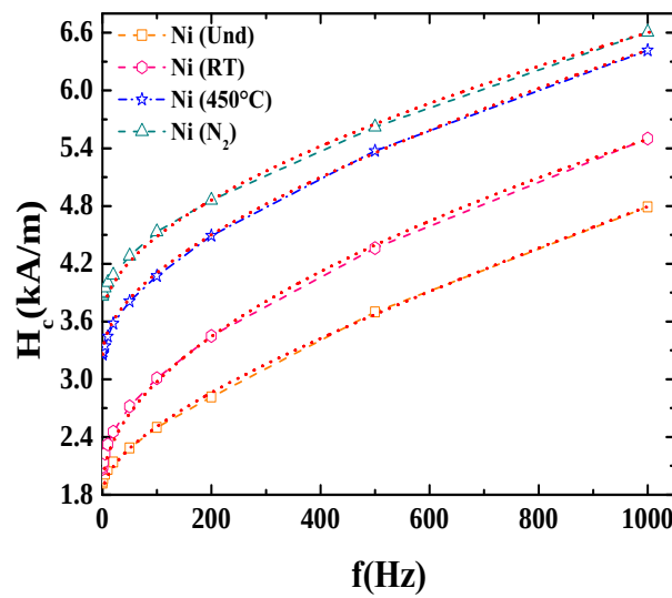
Figure 4.27: Fitting applying model Eq. (4.7) on the coercivity versus frequency data, indicated by dotted line.
