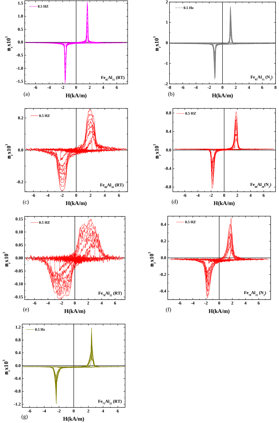
Figure 5.3: Relative permeability versus the field of HPT treated \text{Fe}_{100-x}\text{Al}_x ( x = 15 \leq x \leq 25 ) samples.
