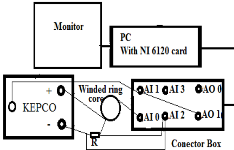
Figure 2.3: Diagram of the LabVIEW controlled hysteresigraph.
