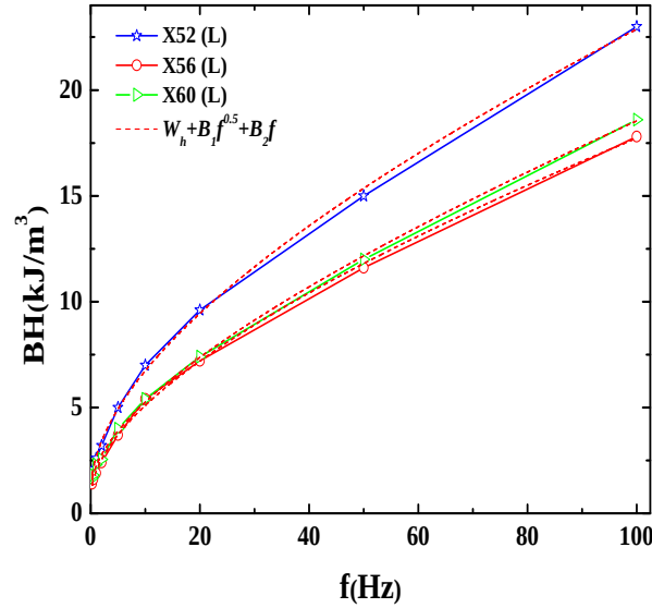
Figure 7.11: Total losses per cycle with frequency of X52 (L), X56 (L), and X60 (L). The dotted indicates the fitting result.
