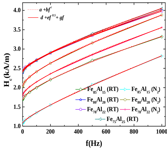
Figure 5.5: Fitting applying Eqs. (5.3) and (5.4) on experimental data of coercivity versus frequency of HPT treated \text{Fe}_{100-x}\text{Al}_x ( 15 \leq x \leq 25 ) samples.
