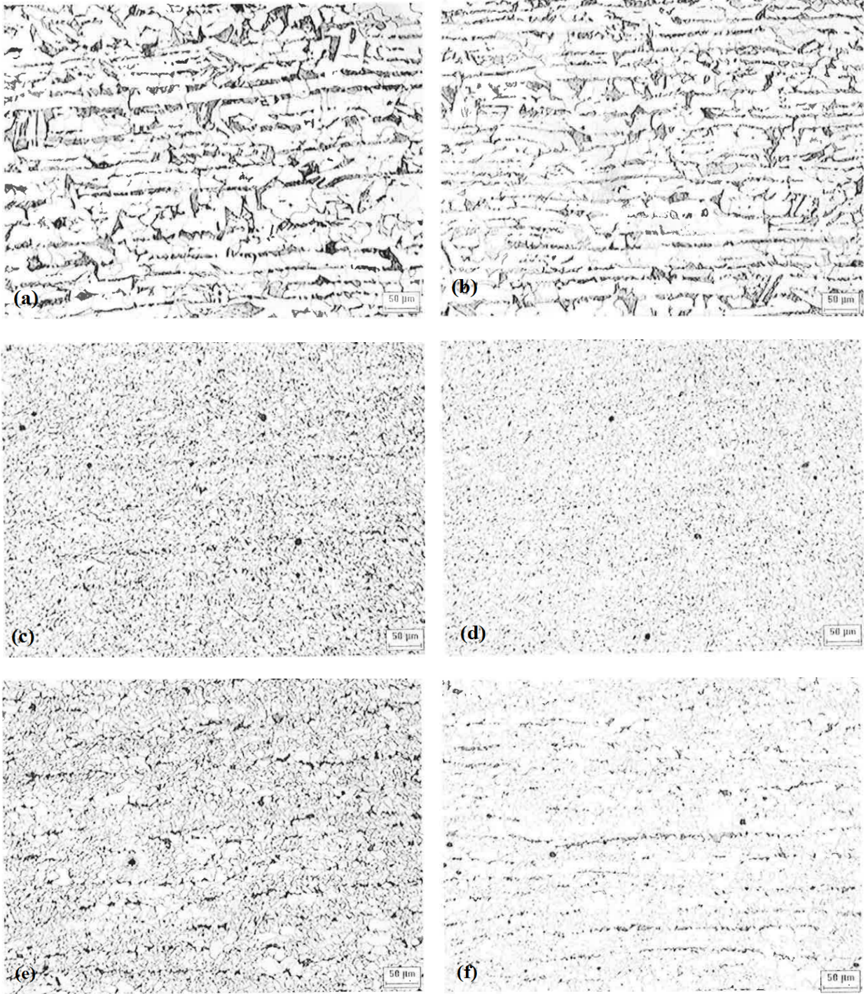
Figure 7.1: Microstructure of a longitudinal (left) and transversal (right) section of X52 (a, b), X56 (c, d) and X60 (e, f).
