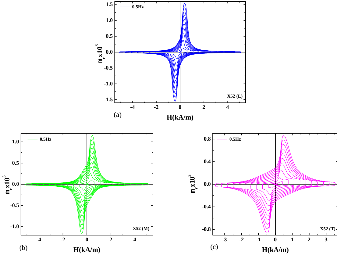
Figure 7.6: Relative permeability \mu_r versus field H(t) for pipeline steel X52 (a) X52 (L), (b) X52 (M), (c) X52 (T).
