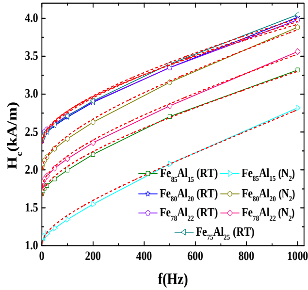
Figure 5.6: Fit applying the model Eq. (5.6) on experimental data of the coercivity versus frequency of of HPT-treated \text{Fe}_{100-x}\text{Al}_x ( 15 \leq x \leq 25 ) samples.
