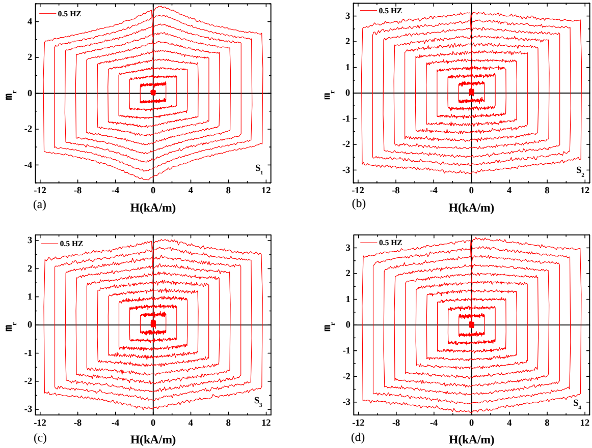
Figure 8.9: Relative permeability versus field of resin coated Fe-powder samples (a) S_1 , (b) S_2 , (c) S_3 and (d) S_4 .
