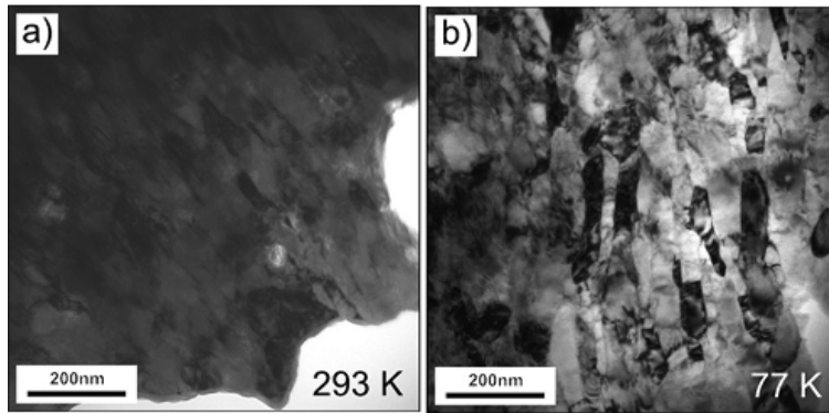
Figure 1.7: TEM micrographs of P800 deformed at low temperatures (293 K and 77 K) [1].
