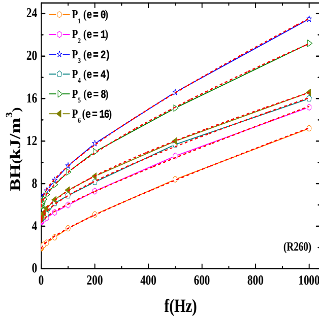
Figure 6.7: Total losses versus frequency for SPD pearlitic steel (R260) and analyzed by applying Eq.(6.2) shown by dotted line.
