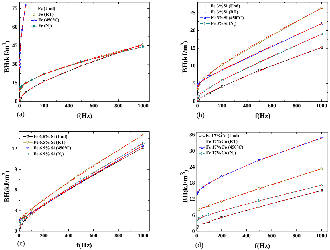
Figure 4.19: Fitting applying Eq. 4.8 on the frequency dependence of the losses; HPT-treated (a) Fe, (b) Fe-3 wt%Si, (c) Fe-6.5 wt%Si and (d) Fe-17 wt%Co samples.
