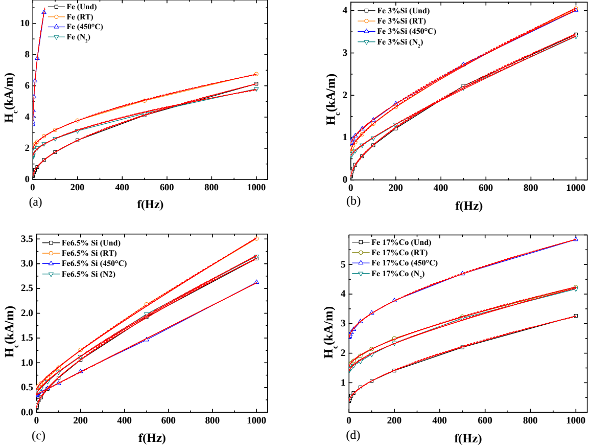
Figure 4.17: Fitting on frequency dependent coercivity of HPT-treated samples at room temperature by Eqs. (4.3) and (4.4) (a) Fe, (b) Fe-3 wt%Si, (c) Fe-6.5 wt%Si and (d) Fe-17 wt%Co.
