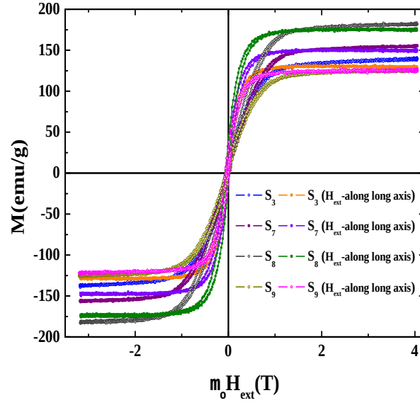
Figure 8.4: Magnetization loops of resin coated Fe-Powder to see demagnetizing effect.
