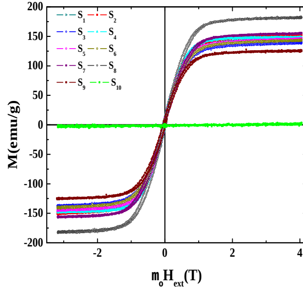
Figure 8.2: Magnetization M(H) loops of resin coated Fe-Powder.
