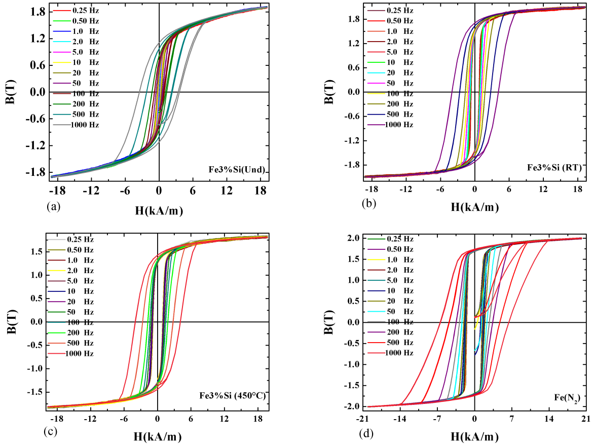
Figure 4.4: The frequency dependence hysteresis loops HPT-treated Fe-3 wt%Si (a) undeformed, (b) deformed at 300 K (RT), (c) deformed at 723 K and (d) deformed at liquid ( \text{N}_2 ) temperature.
