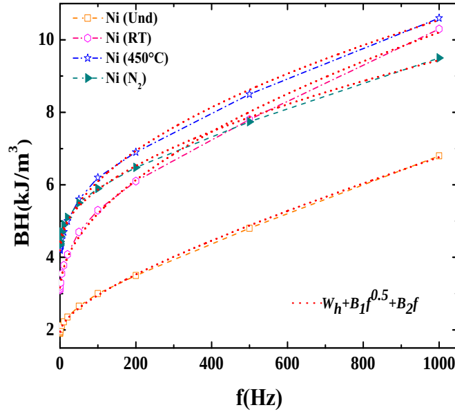
Figure 4.28: Frequency dependence of the losses calculated by integrated hysteresis loops of HPT treated Ni (dotted line indicate fitting).
