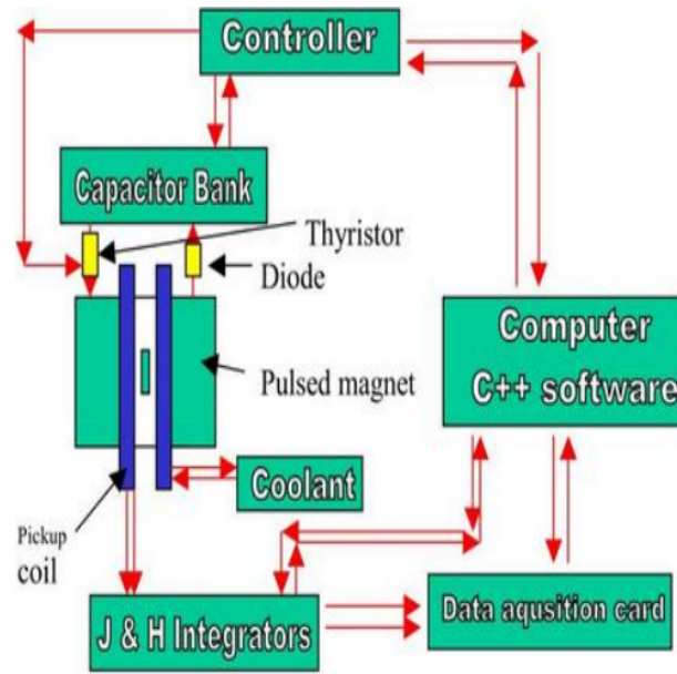
Figure 2.8: Block diagram of the pulse field magnetometer [4].
