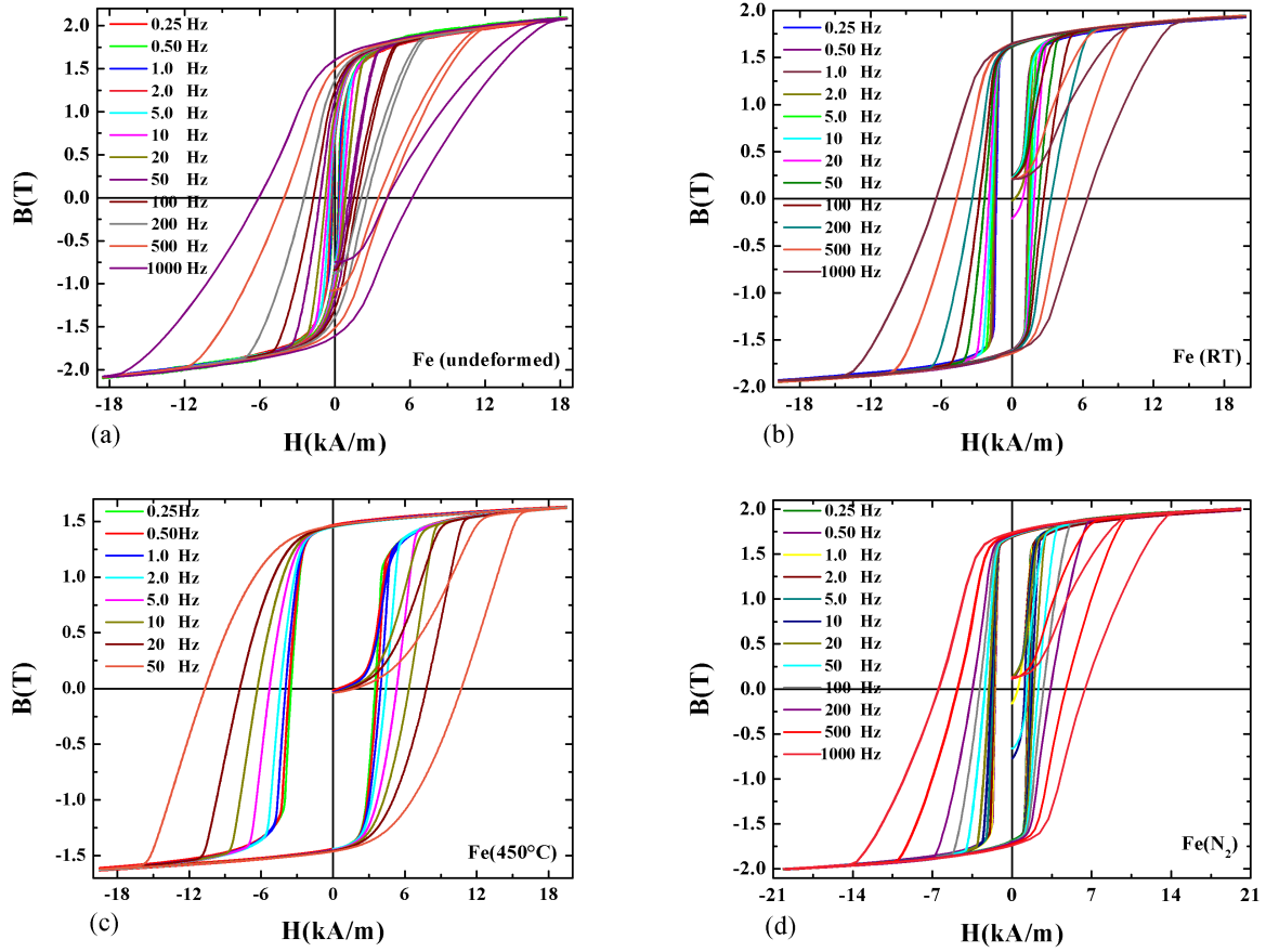
Figure 4.3: The frequency dependence hysteresis loops of HPT-treated pure Fe (a) undeformed, (b) deformed at 300 K (RT), (c) deformed at 723 K and (d) deformed at liquid ( N_2 ) temperature.
