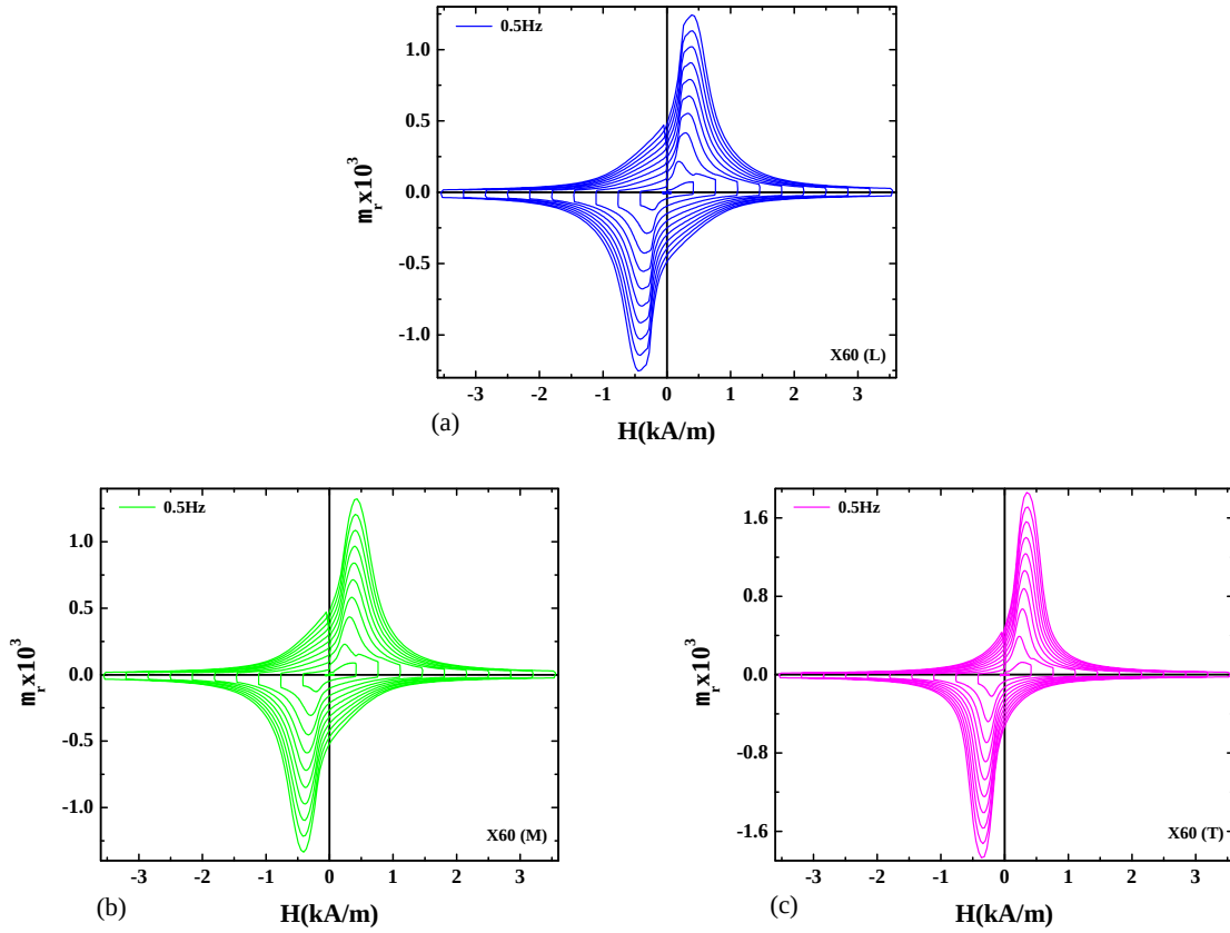
Figure 7.8: Relative permeability \mu_r versus field H(t) for pipeline steel X60 (a) X60 (L), (b) X60 (M) and (c) X60 (T).
