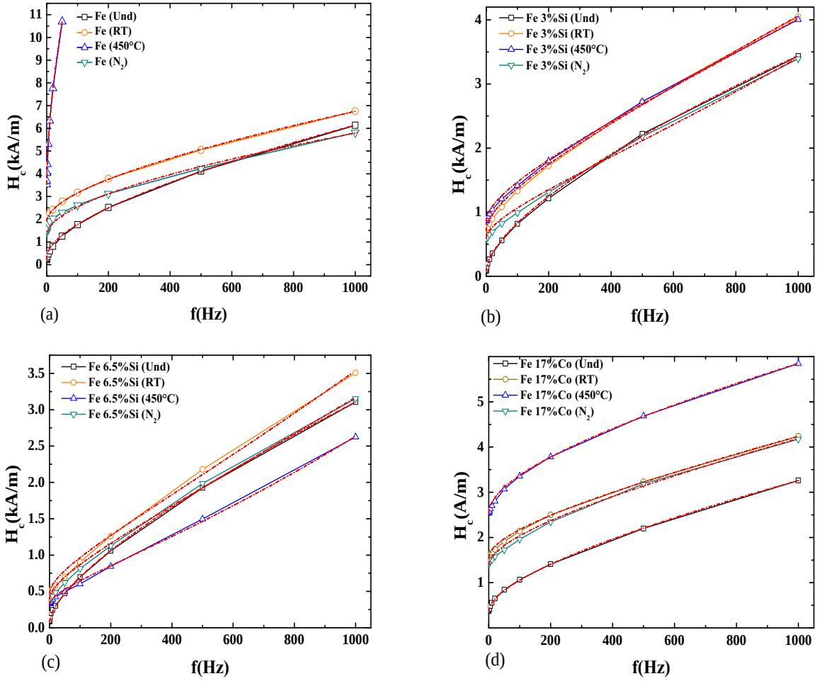
Figure 4.18: Fitting according to model Eq. 4.7 on the data coercivity versus frequency of HPT-treated Fe, Fe-3 wt%Si, Fe-6.5 wt%Si and Fe-17 wt%Co samples, whereas \Delta k described the error in k .
