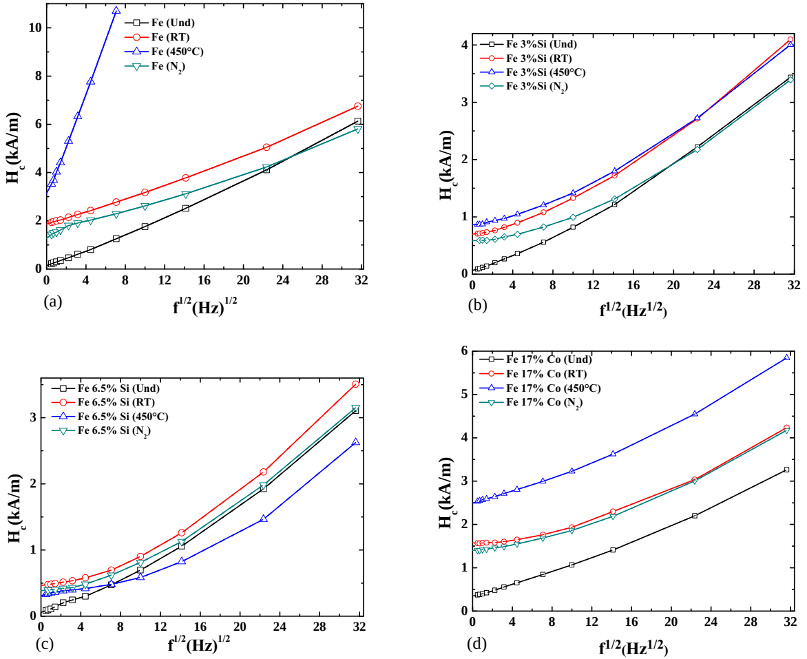
Figure 4.8: Frequency versus coercivity of HPT-treated (a) Fe, (b) Fe-3 wt%Si, (c) Fe-6.5 wt%Si and (d) Fe-17 wt%Co.
