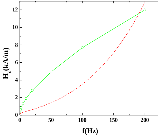
Figure 3.2: Comparison between model and experimental curve of H_c versus f . Solid line (experimental) and dotted line (model)
