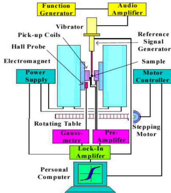
Figure 2.10: Block diagram of the vibrating sample magnetometer (VSM) [4].
