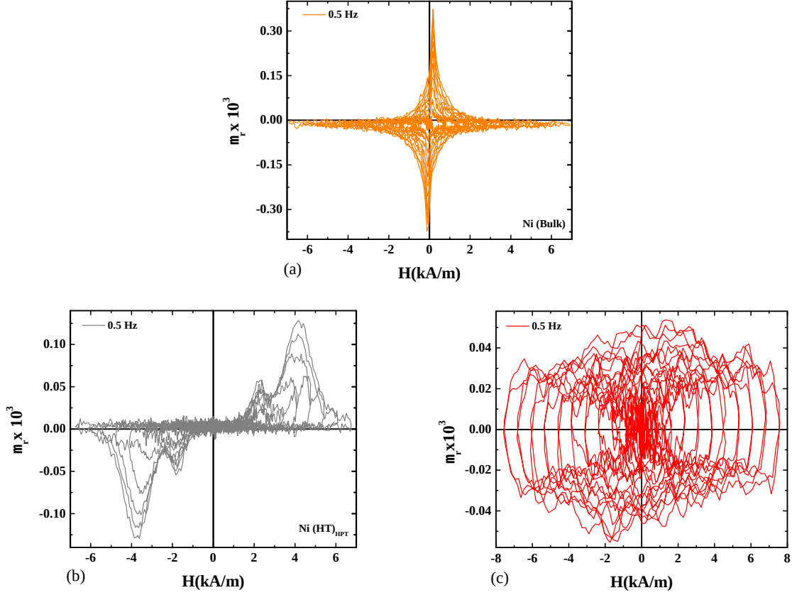
Figure 4.24: Relative permeability versus the field (a) Ni(Bulk), (b) HPT-deformed and heat treated Ni(HT) HPT and (c) Nano-crystalline Ni(nc) samples at room temperature.
