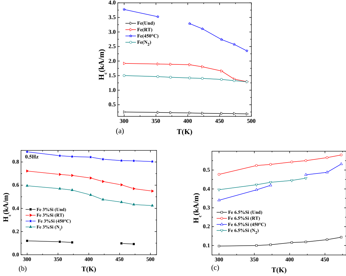
Figure 4.14: Temperature dependent coercivity of HPT-treated (a) Fe, (b) Fe-3 wt%Si and (c) Fe-6.5 wt%Si samples.
