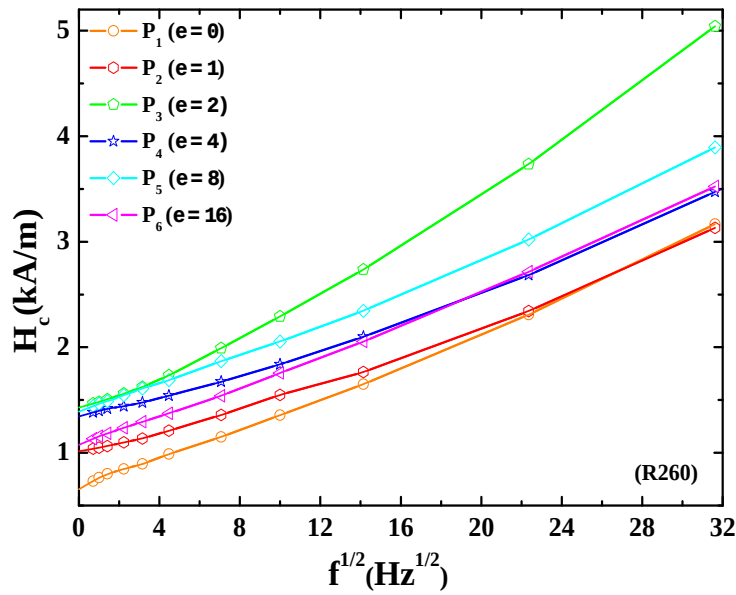
Figure 6.3: Coercivity versus square root of frequency of SPD treated pearlitic steel (R260).
