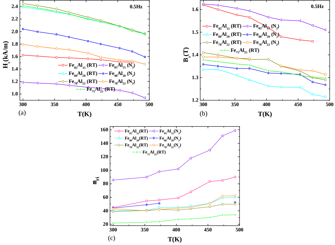
Figure 5.4: (a) coercivity versus temperature (b) saturation magnetization versus temperature and (c) initial relative permeability versus temperature (K) of HPT treated \text{Fe}_{100-x}\text{Al}_x ( x = 15 \leq x \leq 25 ) samples.
