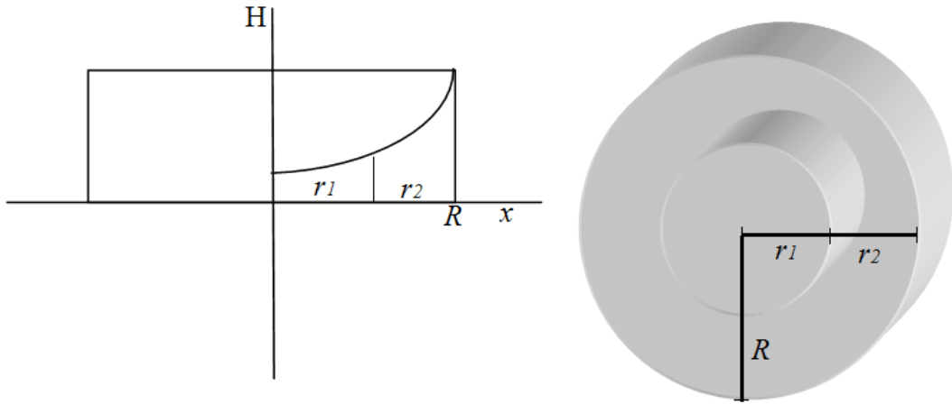
Figure 3.1: Schematic diagram for Eddy current model.
