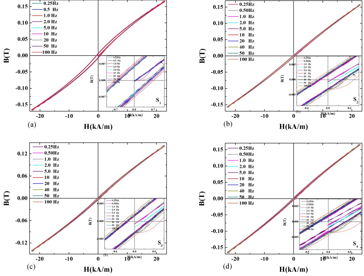
Figure 8.5: Frequency dependent hysteresis loops of resin coated Fe-Powder samples (a) S_1 , (b) S_2 , (c) S_3 and (d) S_4 .
