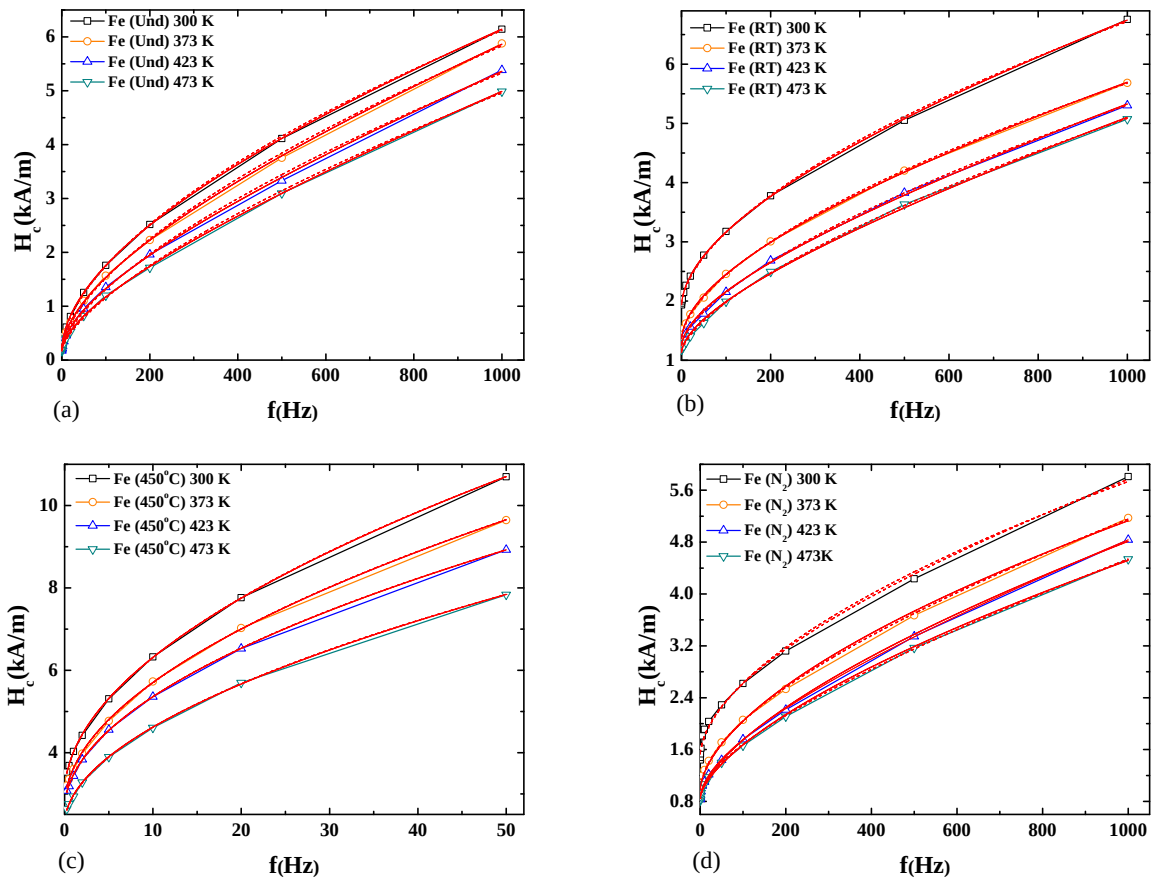
Figure 4.16: Fitting on the frequency dependent coercivity of HPT-treated Fe at different temperature by Eqs. (4.3) and (4.4) (a) un-deformed, (b) deformed at RT, (c) deformed at 450°C and (d) deformed at N_2 .
