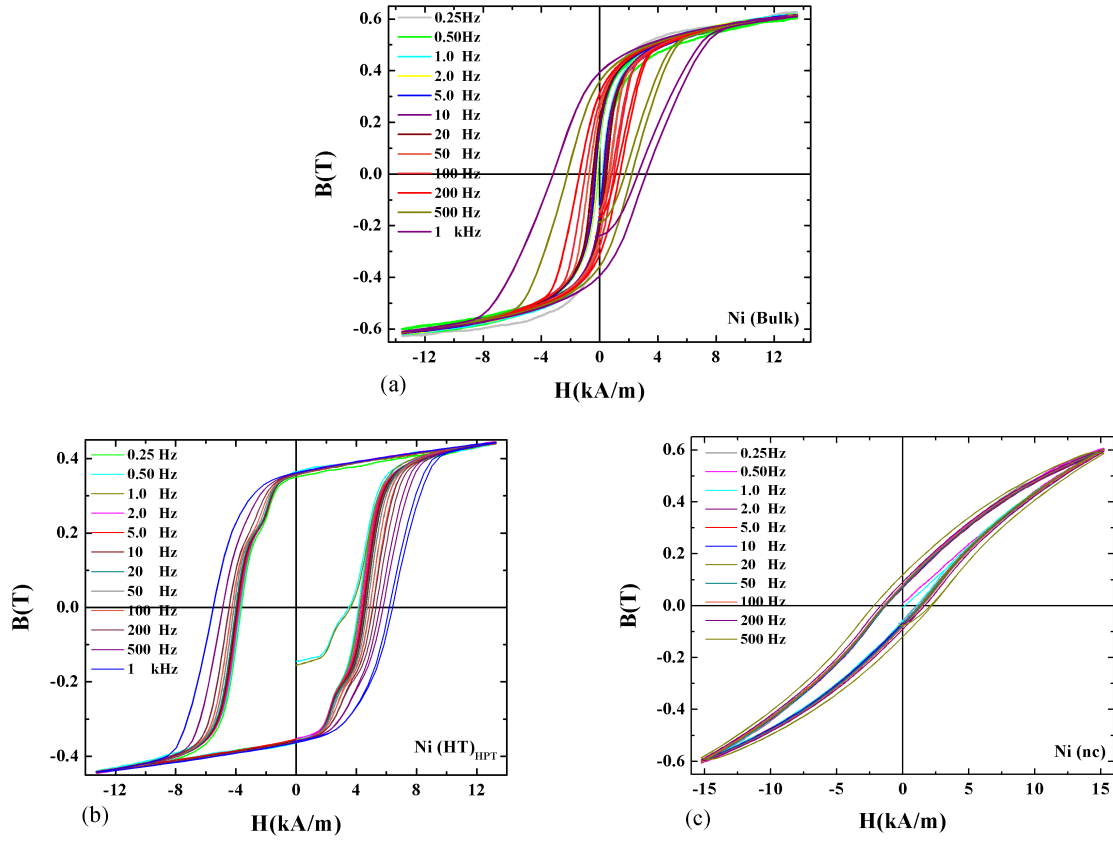
Figure 4.21: Hysteresis loops of Ni (a) Bulk, (b) HPT deformed and heat treated (420°C for 1 hr) and (c) Nano-crystalline Ni.
