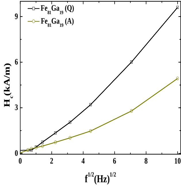
Figure 5.9: Extrapolated coercivity as a function of square root of frequency of Fe 81 Ga 19 quenched (Q) and annealed (A) samples.
