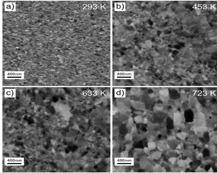
Figure 1.6: BSE images of HPT deformed P800 in radial direction; the samples were deformed at different temperatures (see insets) [1].
