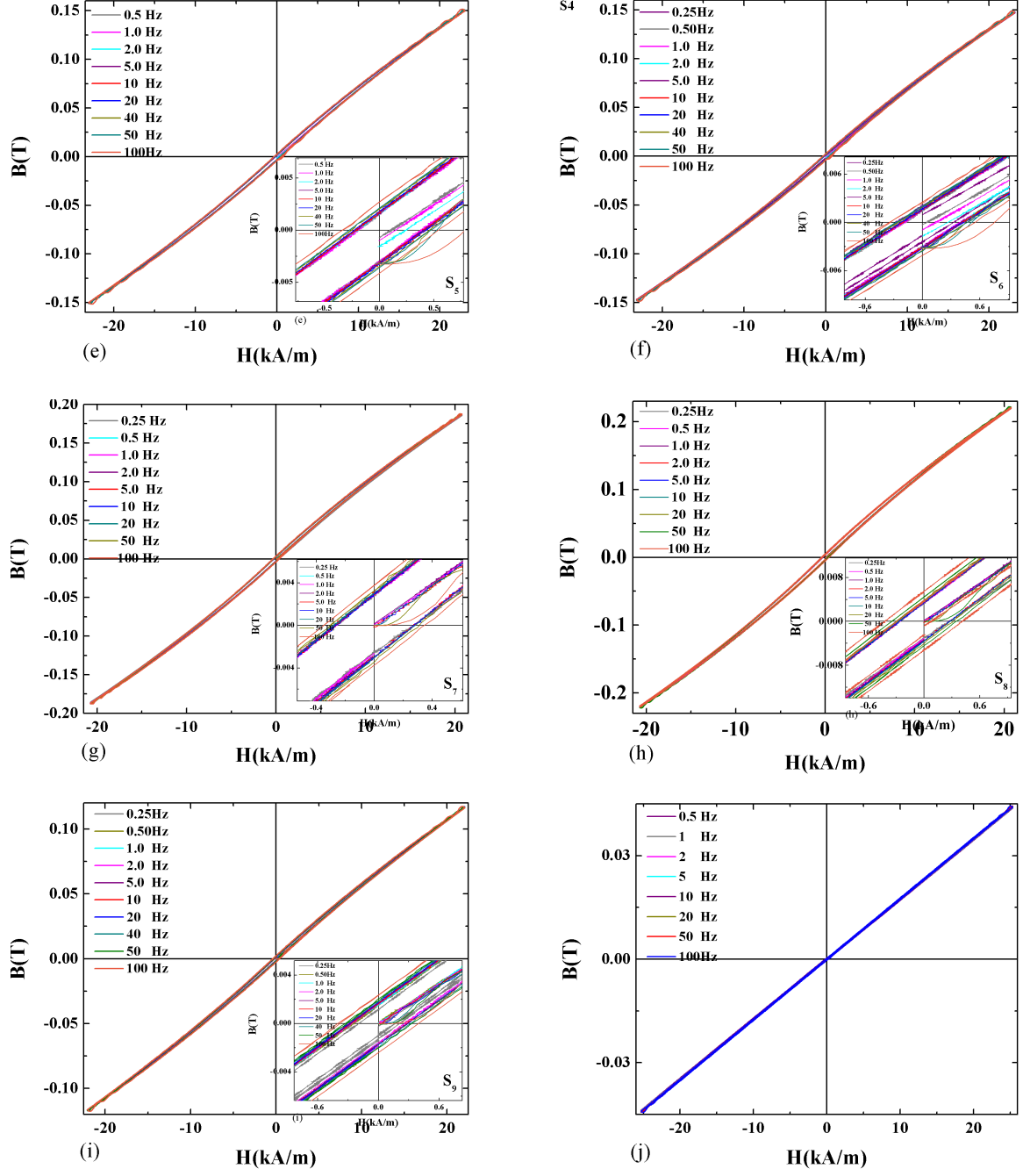
Figure 8.6: Frequency dependent hysteresis loops of resin coated Fe-Powder (e) S_5 , (f) S_6 , (g) S_7 , (h) S_8 , (i) S_9 and (j) S_{10} .
