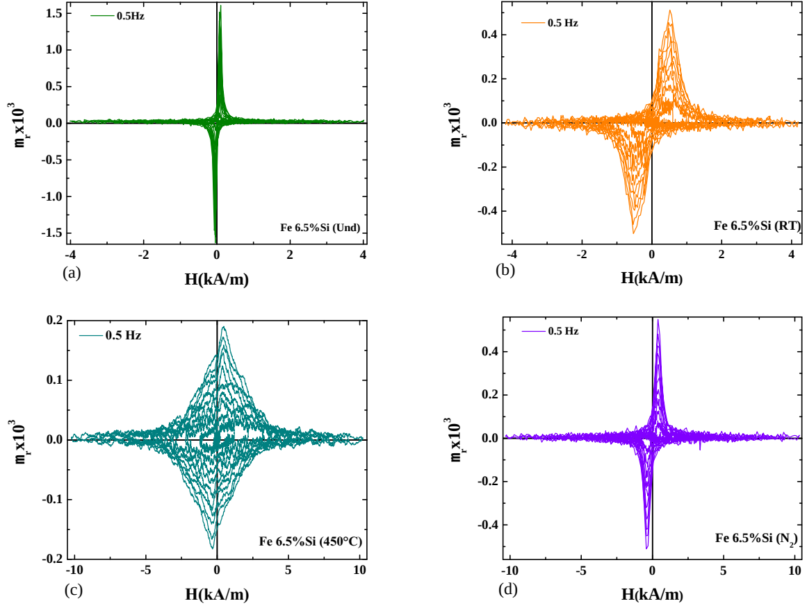
Figure 4.12: Relative permeability versus the field for HPT-treated Fe-6.5 wt%Si samples at room temperature.
