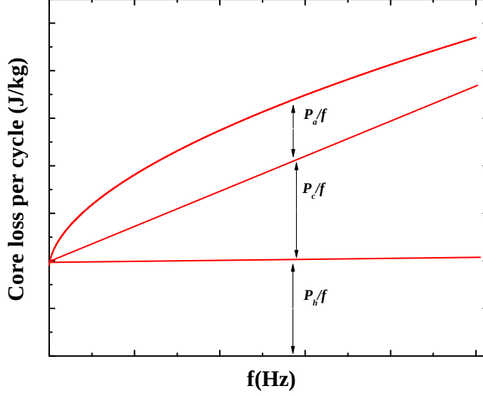
Figure 1.4: Separation of core losses.
