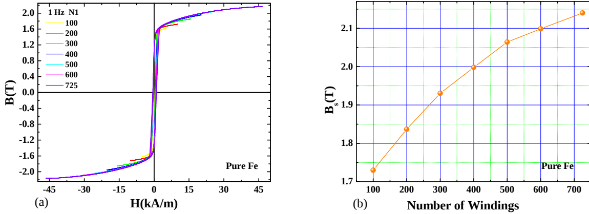
Figure 2.5: (a) Hysteresis loops measured at 1 Hz on pure Fe with different numbers of primary windings (b) Magnetization as a function of the number of the primary windings ( N_1 ).
