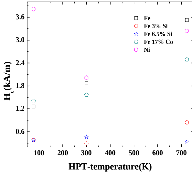
Figure 4.7: Dependence of the zero extrapolated coercivity versus the HPT-deformation temperature for: pure Fe, Fe-3 wt%Si, Fe-6.5 wt%Si, Fe-17 wt%Co (P800) and Ni.
