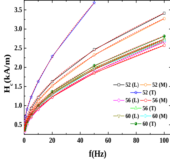
Figure 7.10: Fitting according to Eq. (3.15) on experimental data of coercivity versus frequency of X52, X56, and X60 pipeline steel.
