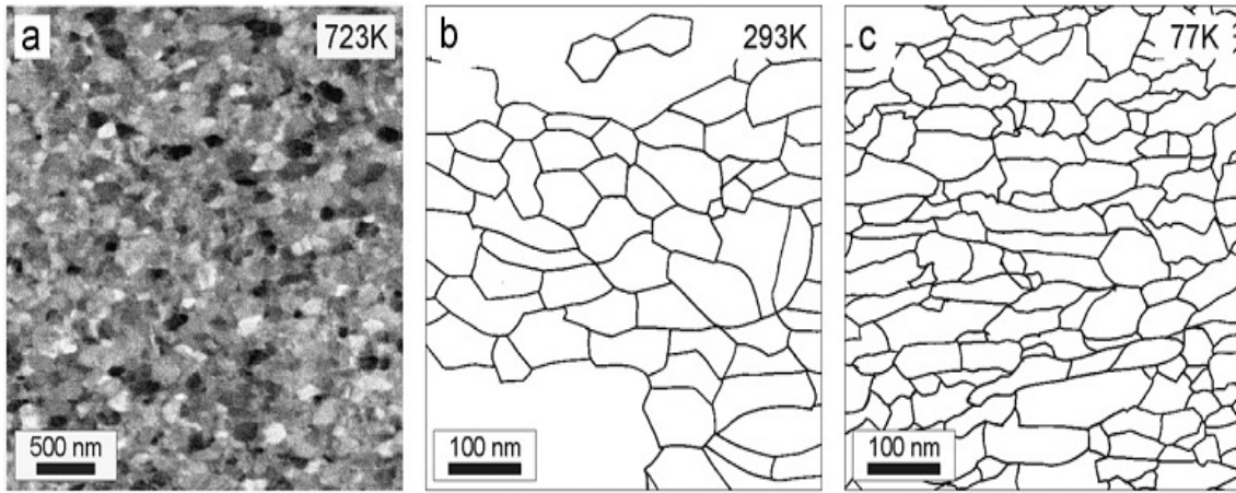
Figure 4.1: Grain size maps for Fe-17 wt% Co alloy correspond (a) 723 K, (b) 293 K and (c) 77 K [5].
