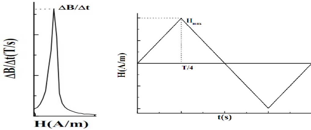
Figure 3.3: dB/dt versus H(t) loop and triangular form of field H(t) .
