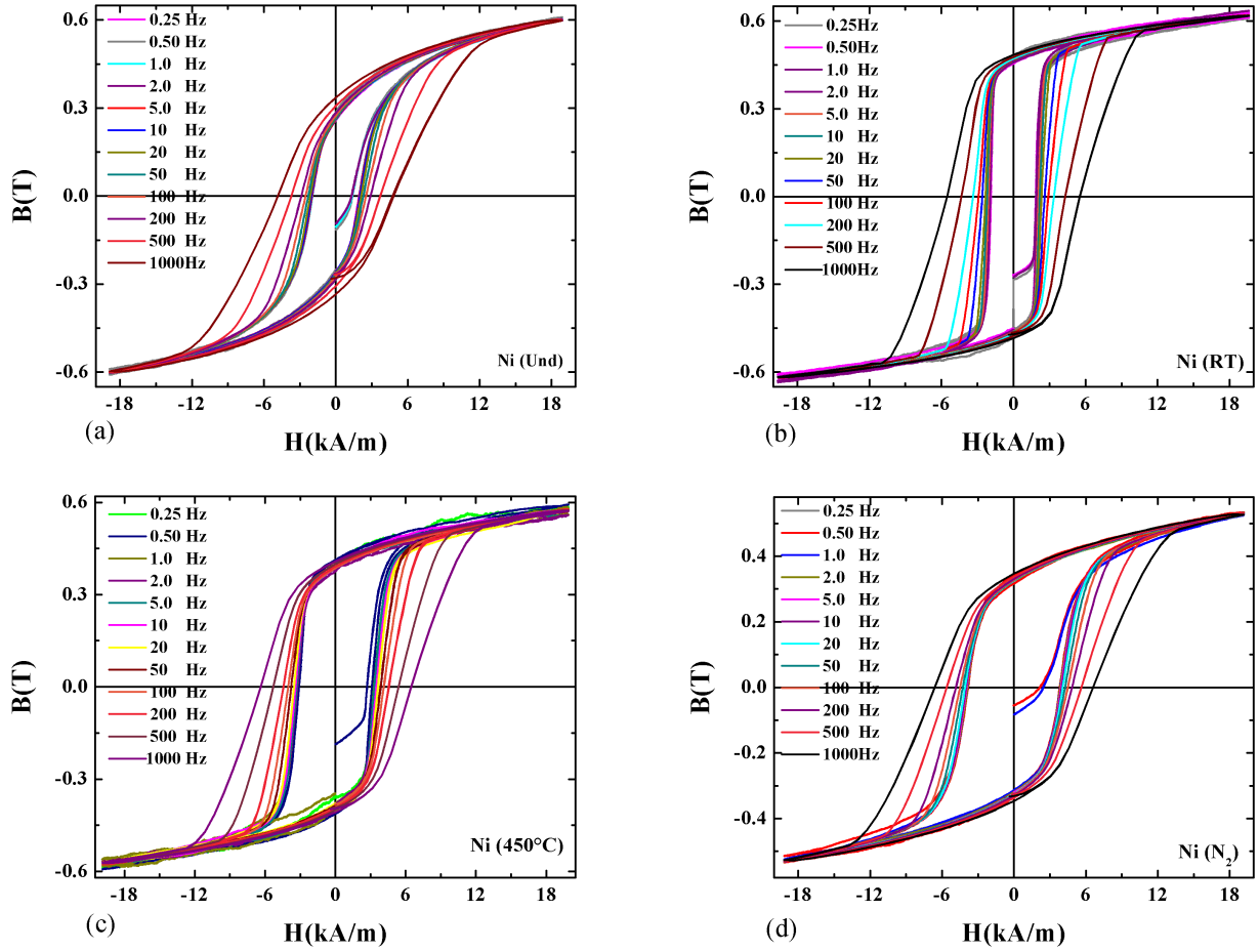
Figure 4.20: Hysteresis loops of HPT-treated Ni (a) un-deformed, (b) deformed at RT (300 K), (c) deformed at 450°C (723 K) and (d) deformed at liquid N 2 temperature (77 K).
