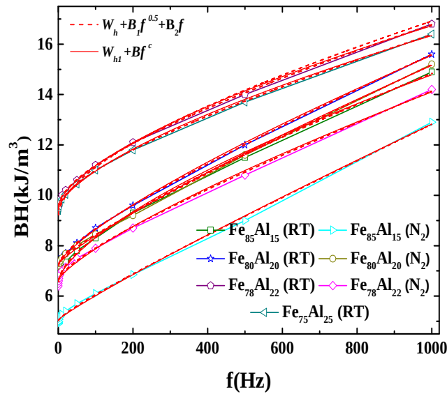
Figure 5.7: Fitting according to equation (5.8) and (5.9) on the frequency dependence of the losses of HPT-treated Fe 100-x Al x (15 ≤ x ≤ 25) samples.
