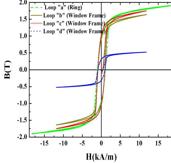
Figure 2.7: Hysteresis loops measured on the ring and the window frame samples.
