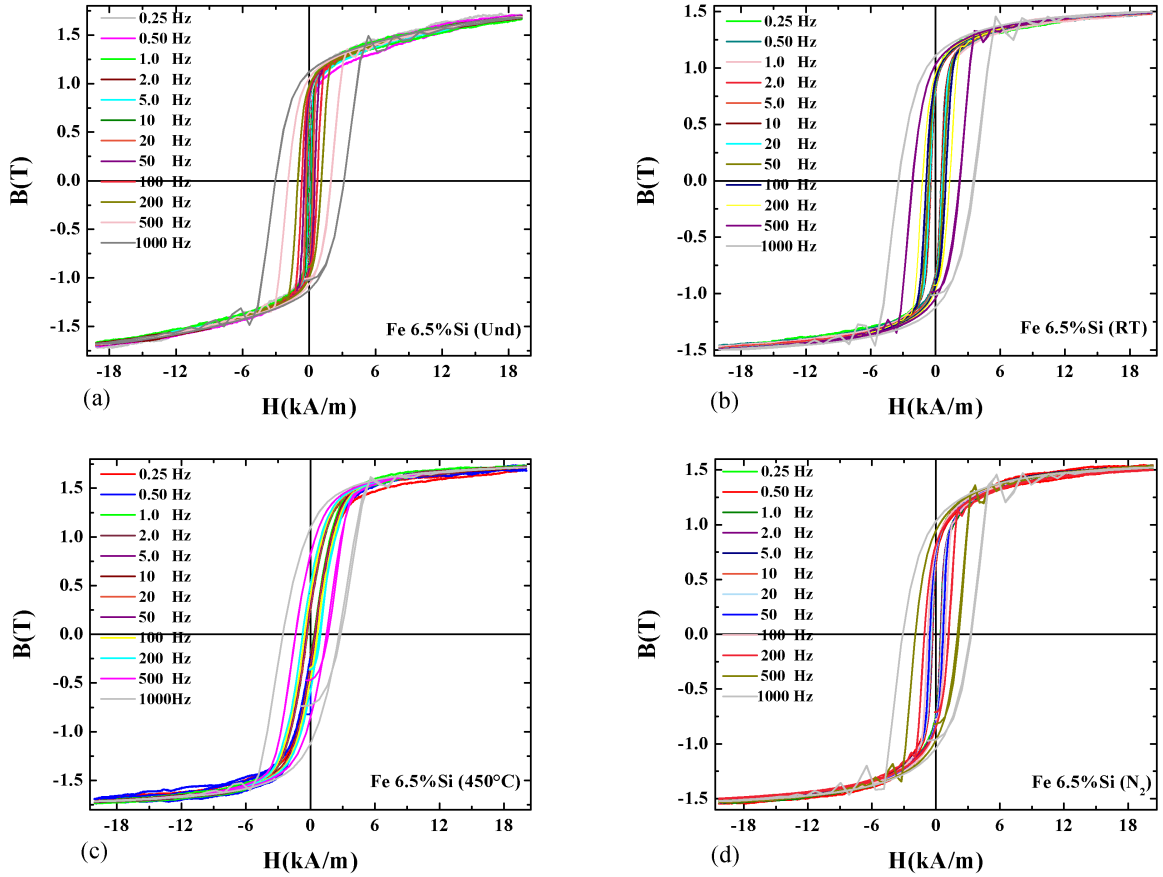
Figure 4.5: The frequency dependence hysteresis loops of HPT-treated Fe-6.5 wt%Si (a) un-deformed, (b) deformed at 300 K (RT), (c) deformed at 723 K and (d) deformed at liquid (N 2 ) temperature.
