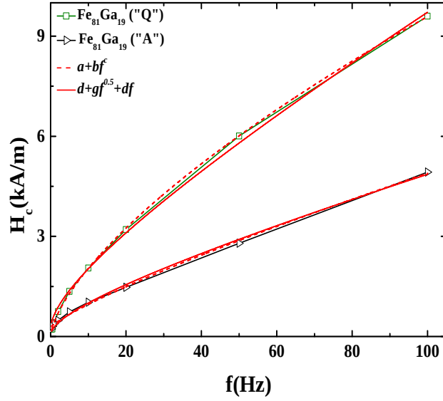
Figure 5.11: Fitting according to Eqs. 5.3 and 5.4 on experimental data of coercivity versus frequency of quenched and annealed \text{Fe}_{81}\text{Ga}_{19} samples.
