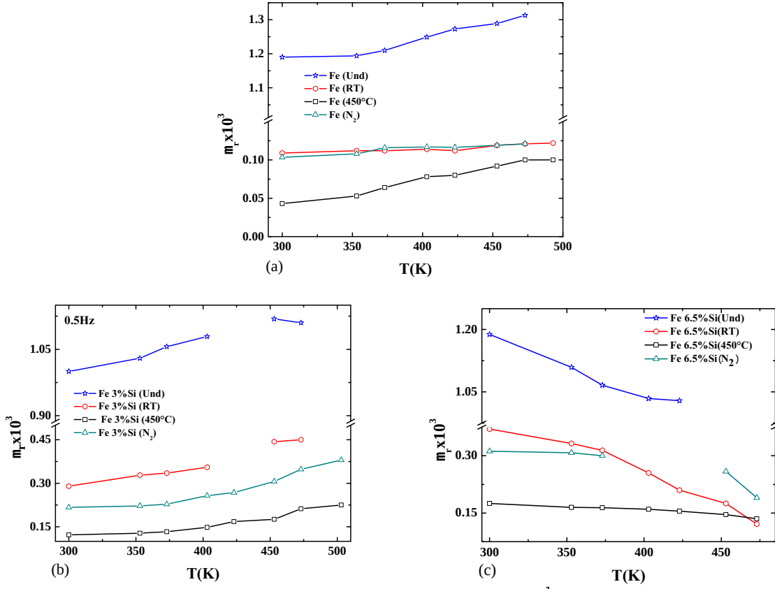
Figure 4.15: Relative initial permeability versus Temperature of HPT-treated (a) Fe, (b) Fe-3 wt%Si and (c) Fe-6.5 wt%Si samples.
