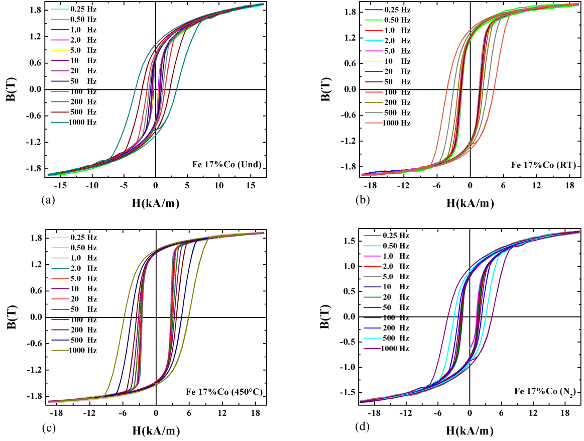
Figure 4.6: The frequency dependence hysteresis loops of HPT-treated Fe-17 wt%Co (a) un-deformed, (b) deformed at 300 K (RT), (c) deformed at 723 K, and (d) deformed at liquid ( N_2 ) temperature.
