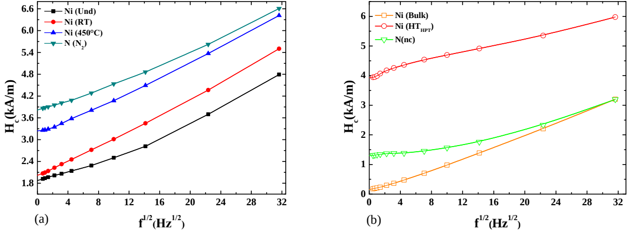
Figure 4.22: Coercivity versus square root of the frequency of (a) HPT-treated Ni and (b) Ni(Bulk), HPT-deformed with heat treatment Ni(HT) HPT , nano-crystalline Ni(nc) samples.
