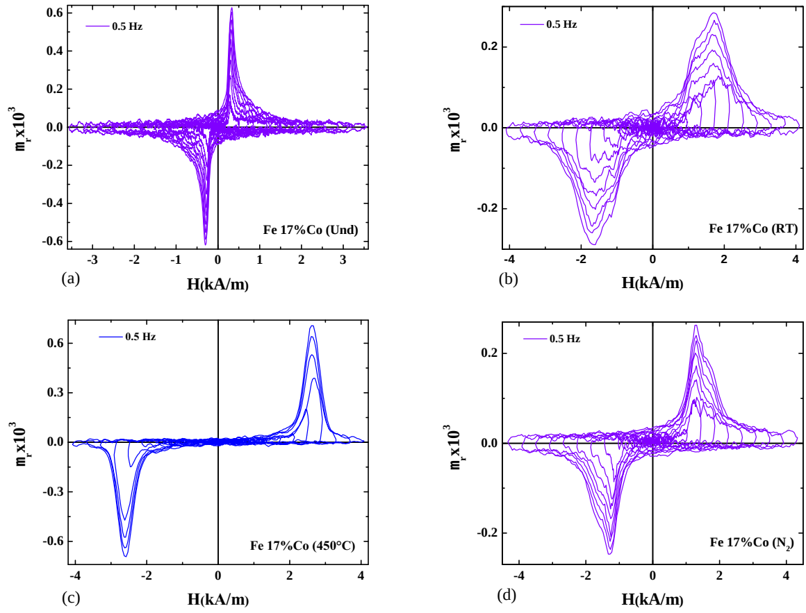
Figure 4.13: Relative permeability versus the field for HPT-treated Fe-17 wt%Co (P800) samples at room temperature.
