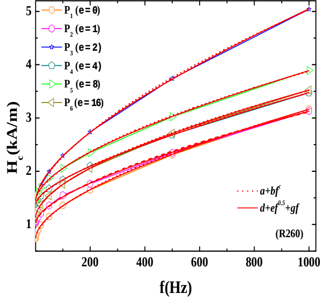
Figure 6.5: Fitting according to Eqs. (3.16) and (3.17) on coercivity versus frequency data of SPD treated pearlitic steel (R260).
