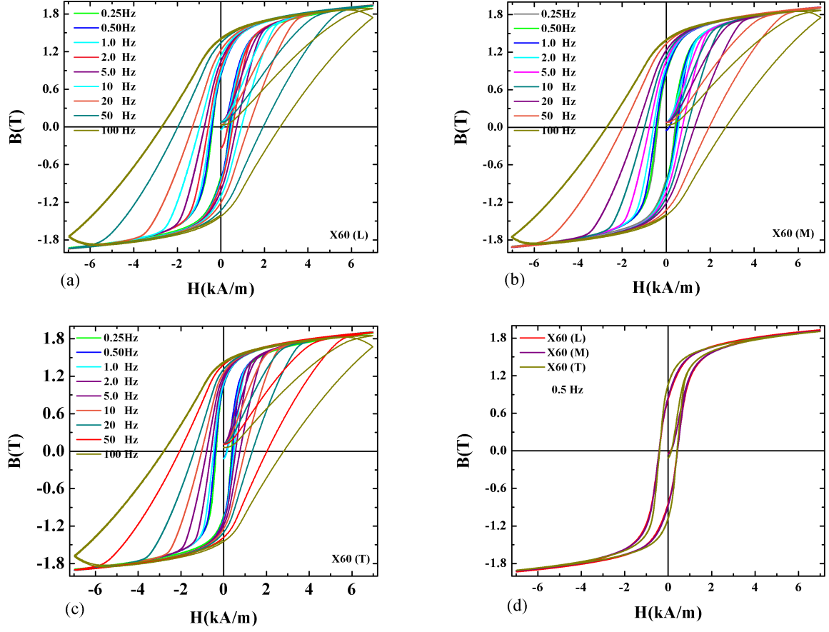
Figure 7.4: Hysteresis loops for X60 steel (a) L , (b) M , (c) T and (d) Comparison of texture at 0.5 Hz.
