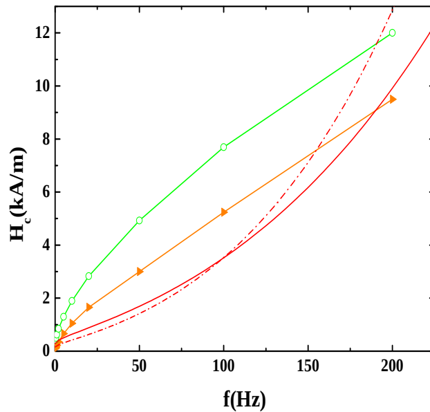
Figure 5.12: Fitting according to Eq. (5.6) on experimental data of coercivity versus frequency of \text{Fe}_{81}\text{Ga}_{19} quenched (Q) and annealed (A) samples.
