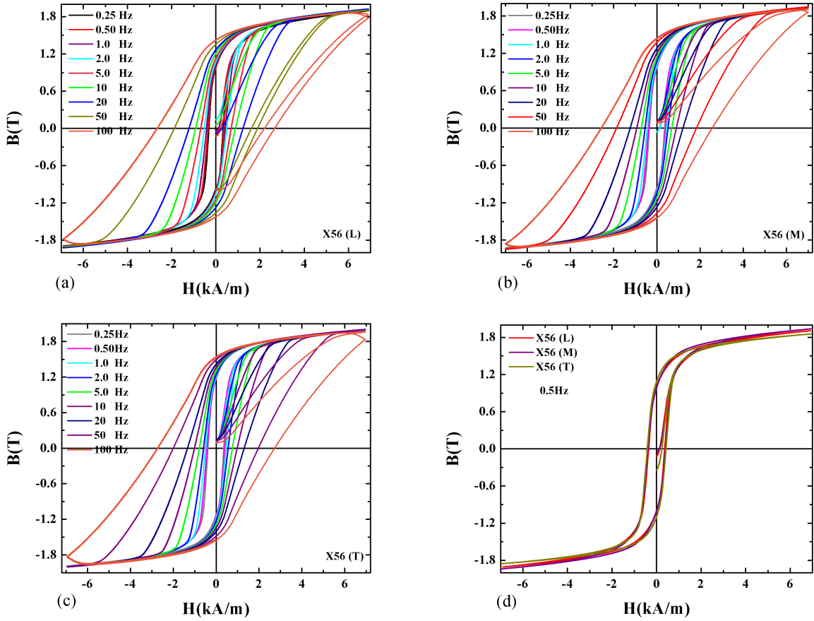
Figure 7.3: Hysteresis loops for X56 steel (a) L , (b) M , (c) T and (d) Comparison of texture at 0.5 H.
