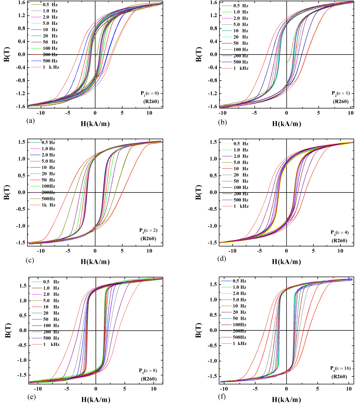
Figure 6.2: Hysteresis loops of SPD treated pearlitic steel (R260) (a) P_1(\epsilon=0) , (b) P_2(\epsilon=1) , (c) P_3(\epsilon=2) , (d) P_4(\epsilon=4) , (e) P_5(\epsilon=8) and (f) P_6(\epsilon=16) .
