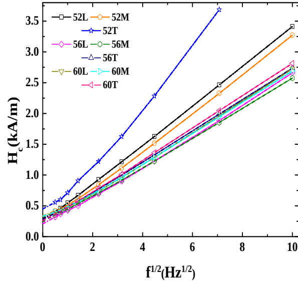
Figure 7.5: Coercivity versus square root of frequency of X52, X56, X60.
