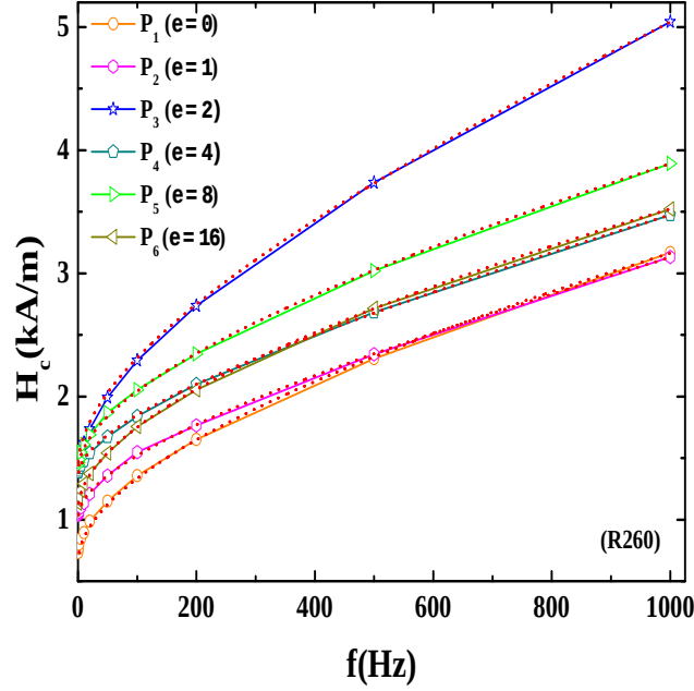
Figure 6.6: Fitting according to Eq. (6.1) on the coercivity versus frequency data of SPD pearlitic steel (R260).
