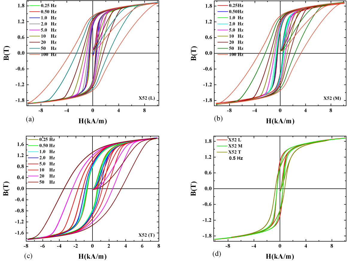
Figure 7.2: Hysteresis loops for X52 steel (a) L , (b) M , (c) T and (d) Comparison of texture of X52 at 0.5 Hz.
