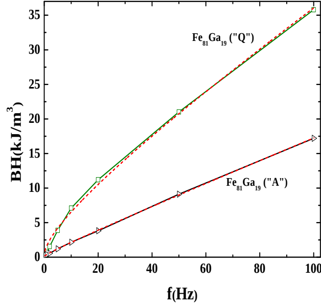
Figure 5.14: Fitting using Eq. 5.9 on the frequency dependence of losses of \text{Fe}_{81}\text{Ga}_{19} quenched (Q) and annealed (A) samples.
