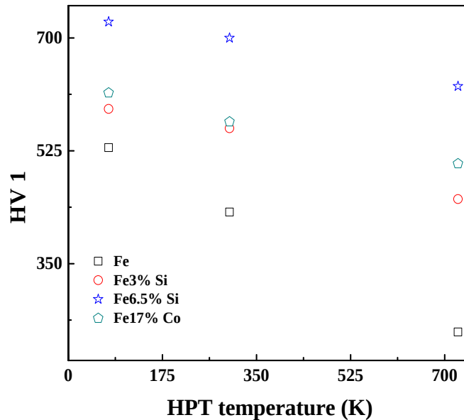
Figure 4.2: Vickers hardness as a function of the HPT processing temperature.
