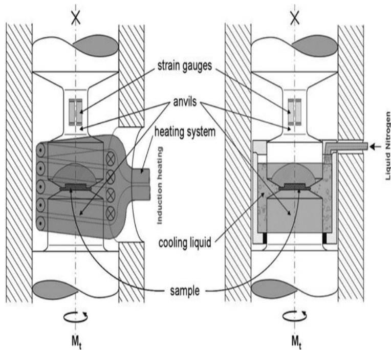
Figure 2.2: Schematic illustration of the used HPT equipment for hot (left) and cold (right) processing [3].
