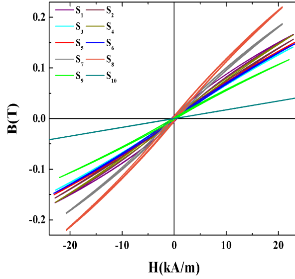
Figure 8.7: Hysteresis loops at 0.5 Hz of all resin coated Fe-Powder samples.
