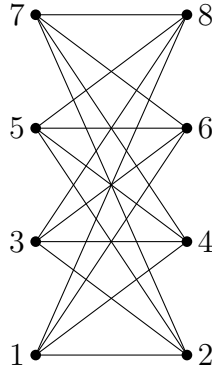
Figure 2.3: K_{4,4}
