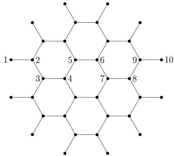
Figure 3.6: Honeycomb lattice
