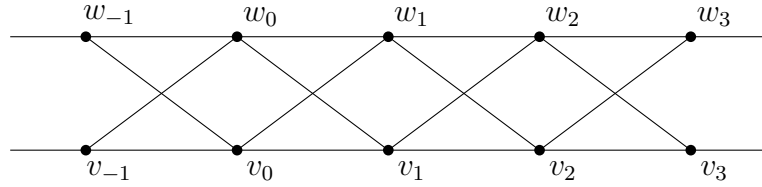
Figure 2.9: Infinite K_{2,2}
