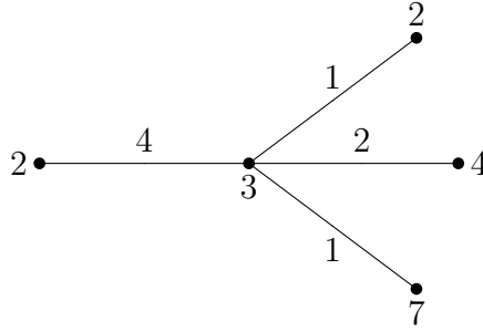
Figure 2.12: Tree of consistent cycles of the “Infinite K_{2,2} ”
