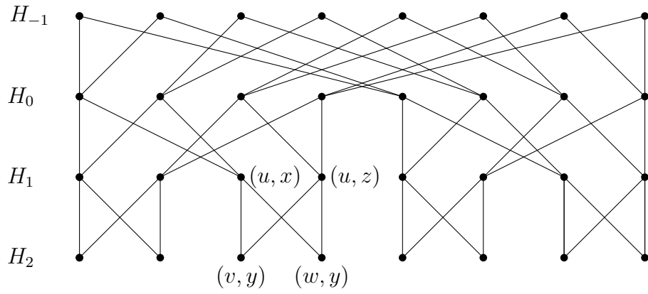
Figure 3.2: DL_{2,2}
