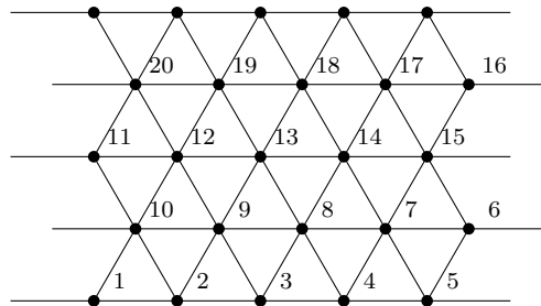
Figure 2.6: Triangular lattice
