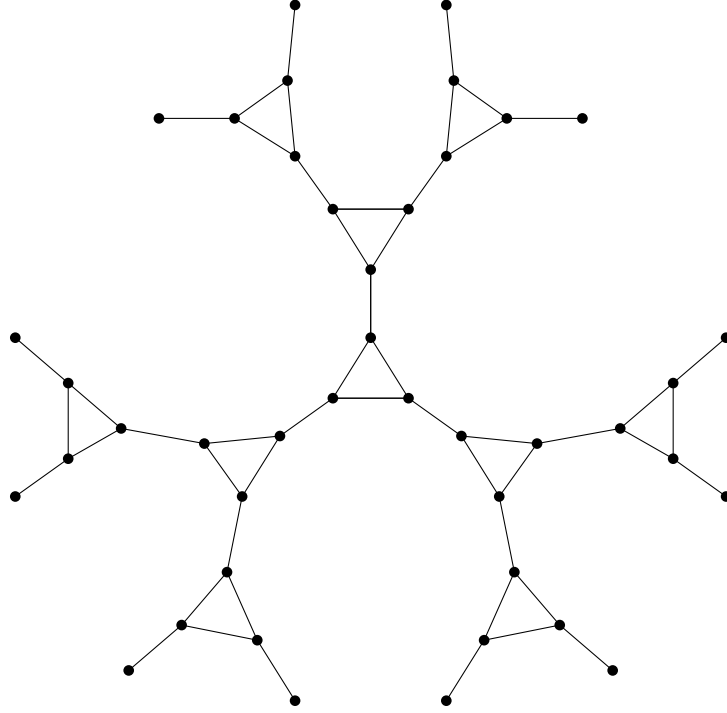
Figure 2.7: Infinite Triangles
