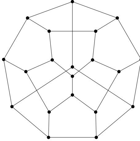
Figure 1.3: Dodecahedron
