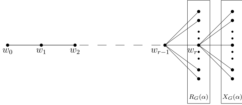
Figure 2.10
