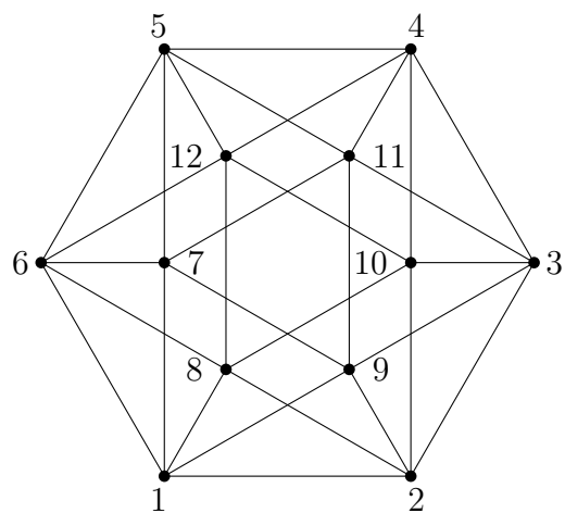
Figure 2.1: Icosahedron
