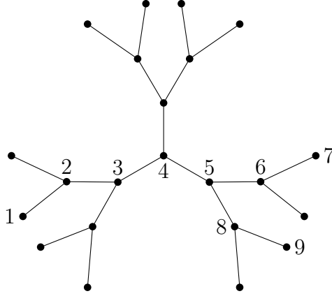
Figure 2.8: 3-regular tree
