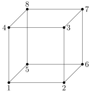
Figure 1.1: Cube
