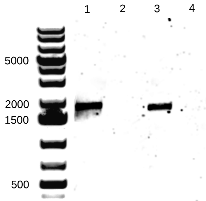
Fig. 1: PCR-amplified Laxus oneistus BPI1 and 2 cDNAs. PCR-products of L. oneistus BPI1-protein (lane 1: Lo-BPI1, lane 2: negative control) and L. oneistus BPI2-protein (lane 3: Lo-BPI2, lane 4: negative control) were visualized by gel electrophoresis. The molecular weight-markers are presented on the left (numbers are in base pairs).
