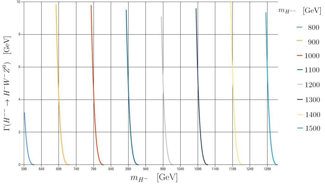
Figure 15: The partial decay width \Gamma(H^{--} \rightarrow H^- W^- Z^0) of the doubly charged Higgs boson for is plotted as a function of m_{H^-} for m_{H^{--}} = 800, 900, 1000, 1100, 1200, 1300, 1400, 1500 GeV. \Gamma(H^{--} \rightarrow H^- W^- Z^0) < 10 GeV was assumed. The range of m_{H^-} is again restricted to the interval [0.75m_{H^{--}}, m_{H^{--}} - m_W - m_Z] for each value of m_{H^{--}} .
