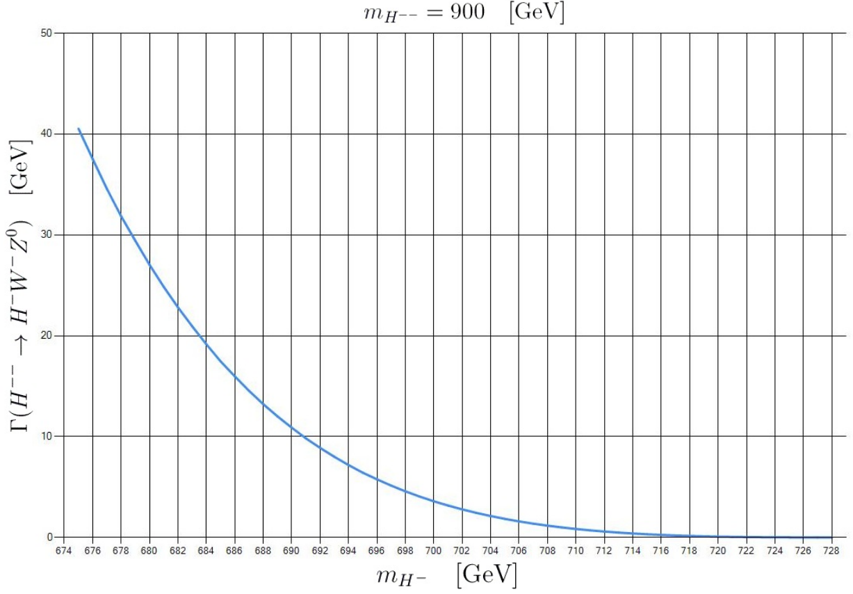
Figure 13: The partial decay width \Gamma(H^{--} \rightarrow H^- W^- Z^0) of the doubly charged Higgs boson for is plotted as a function of m_{H^-} for m_{H^{--}} = 900 \text{ GeV} . Like in the previous figure, \Gamma(H^{--} \rightarrow H^- W^- Z^0) increases strongly with the mass difference m_{H^{--}} - m_{H^-} . The range of m_{H^-} is again restricted to the interval [0.75m_{H^{--}}, m_{H^{--}} - m_W - m_Z] .
