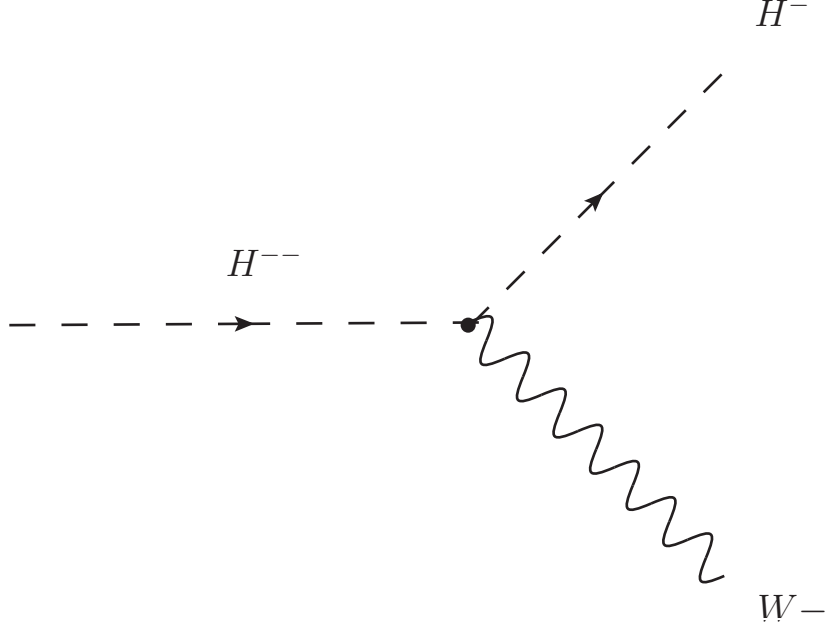
Figure 7: First order Feynman diagram for H^{--} \rightarrow W^- H^-
