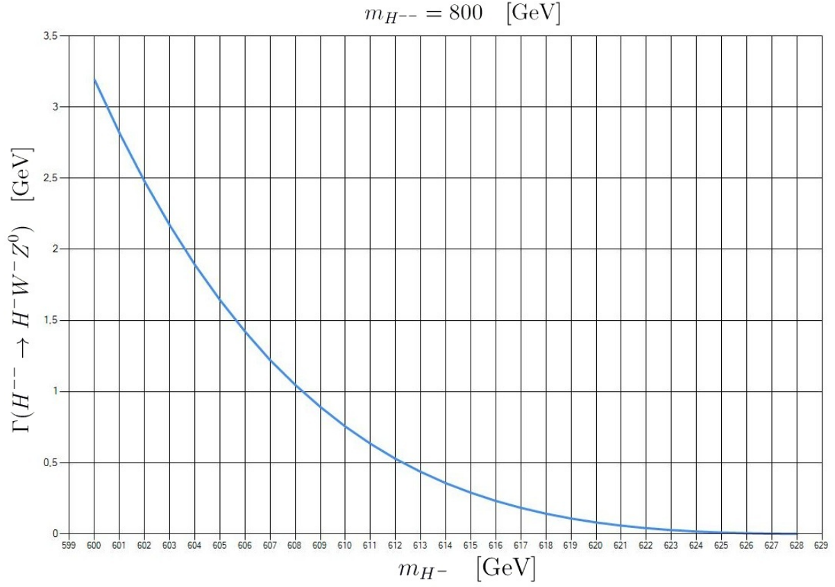
Figure 12: The partial decay width \Gamma(H^{--} \rightarrow H^- W^- Z^0) of the doubly charged Higgs boson is plotted as a function of m_{H^-} for m_{H^{--}} = 800 GeV. As we see \Gamma(H^{--} \rightarrow H^- W^- Z^0) strongly depends on the mass difference m_{H^{--}} - m_{H^-} . Therefore we restricted the range of m_{H^-} to the interval [0.75m_{H^{--}}, m_{H^{--}} - m_W - m_Z] .
