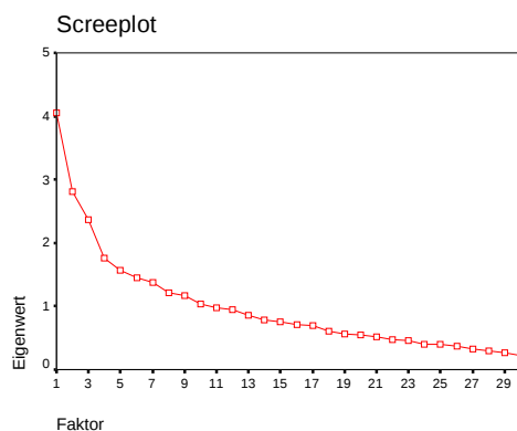
Abb. 12: Screeplot
