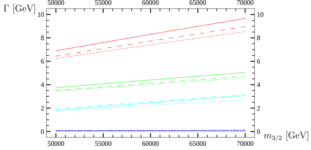
Figure 4.9: \tilde{b}_1 decays; AMSB model. red: t\tilde{\chi}_1^- , green: b\tilde{\chi}_1^0 , blue: b\tilde{\chi}_2^0 , gold: b\tilde{\chi}_3^0 , violet: b\tilde{\chi}_4^0 , cyan: \tilde{t}_1 W^- .
