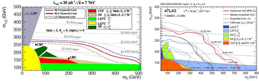
Figure 1.1: left: (The CMS Collaboration): Measured (red line) and expected (dashed blue line) 95% CL exclusion contour at NLO in the CMSSM ( m_0, m_{1/2} ) plane for \tan\beta = 3, A_0 = 0, \text{sign}(\mu) > 0 , taken from [23]; right: (The ATLAS Collaboration): Observed and expected 95% CL exclusion limits in the combined electron and muon channels; taken from [24].
