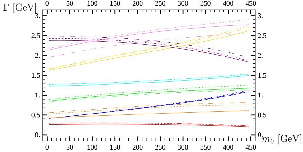
Figure 4.11: \tilde{t}_2 decays; CMSSM model. red: t \tilde{\chi}_1^0 , green: t \tilde{\chi}_2^0 , blue: t \tilde{\chi}_3^0 , gold: t \tilde{\chi}_4^0 , violet: b \tilde{\chi}_1^+ , cyan: b \tilde{\chi}_2^+ , orange: h_0 \tilde{t}_1 , purple: \tilde{t}_1 Z .
