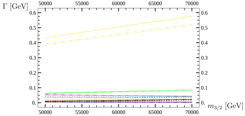
Figure 4.5: \tilde{b}_2 decays; AMSB model. red: t\tilde{\chi}_1^- , green: t\tilde{\chi}_2^- , blue: b\tilde{\chi}_1^0 , gold: b\tilde{\chi}_2^0 , violet: b\tilde{\chi}_3^0 , cyan: b\tilde{\chi}_4^0 , orange: h_0\tilde{b}_1 , purple: \tilde{t}_1 W^- , brown: \tilde{t}_2 W^- , black: \tilde{b}_1 Z .
