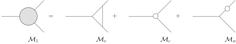
Figure 3.1: One-loop renormalization procedure for a 1 to 2 process schematically
