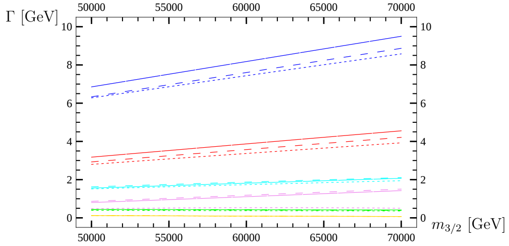
Figure 4.13: \tilde{t}_2 decays; AMSB model. red: t\tilde{\chi}_1^0 , green: t\tilde{\chi}_2^0 , blue: t\tilde{\chi}_3^0 , gold: t\tilde{\chi}_4^0 , violet: h_0\tilde{t}_1 , cyan: \tilde{t}_1 Z .
