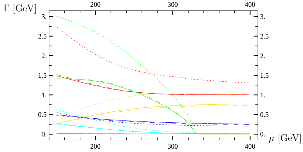
Figure 4.10: \tilde{b}_1 decays; MSSM model. red: t\tilde{\chi}_1^- , green: t\tilde{\chi}_2^- , blue: b\tilde{\chi}_1^0 , gold: b\tilde{\chi}_2^0 , violet: b\tilde{\chi}_3^0 , cyan: b\tilde{\chi}_4^0 , orange: \tilde{t}_1 W^- .
