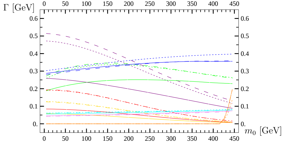
Figure 4.3: \tilde{b}_2 decays; CMSSM model. red: t \tilde{\chi}_1^- , green: t \tilde{\chi}_2^- , blue: b \tilde{\chi}_1^0 , gold: b \tilde{\chi}_2^0 , violet: b \tilde{\chi}_3^0 , cyan: b \tilde{\chi}_4^0 , orange: b \tilde{g} , purple: \tilde{t}_1 W^- .
