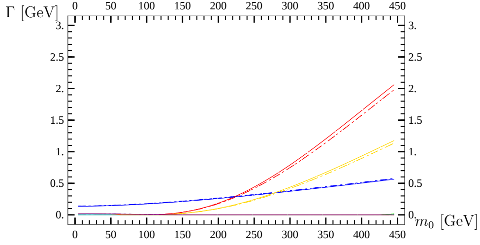
Figure 4.19: \tilde{\tau}_2 decays; CMSSM model. red: \nu_\tau \chi_1^- , green: \nu_\tau \chi_2^- , blue: \tau \chi_1^0 , gold: \tau \chi_2^0 .
