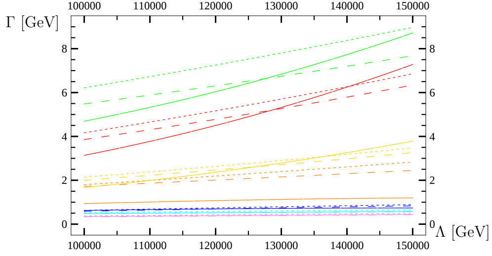
Figure 4.4: \tilde{b}_2 decays; GMSB model. red: t\tilde{\chi}_1^- , green: t\tilde{\chi}_2^- , blue: b\tilde{\chi}_1^0 , gold: b\tilde{\chi}_2^0 , violet: b\tilde{\chi}_3^0 , cyan: b\tilde{\chi}_4^0 , orange: \tilde{t}_1 W^- .
