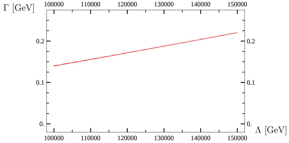
Figure 4.24: \tilde{\tau}_1 decays; GMSB model. red: \tau \tilde{\chi}_1^0 .
