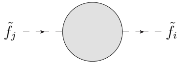
Figure 2.1: Two-point functions for mixing scalars
