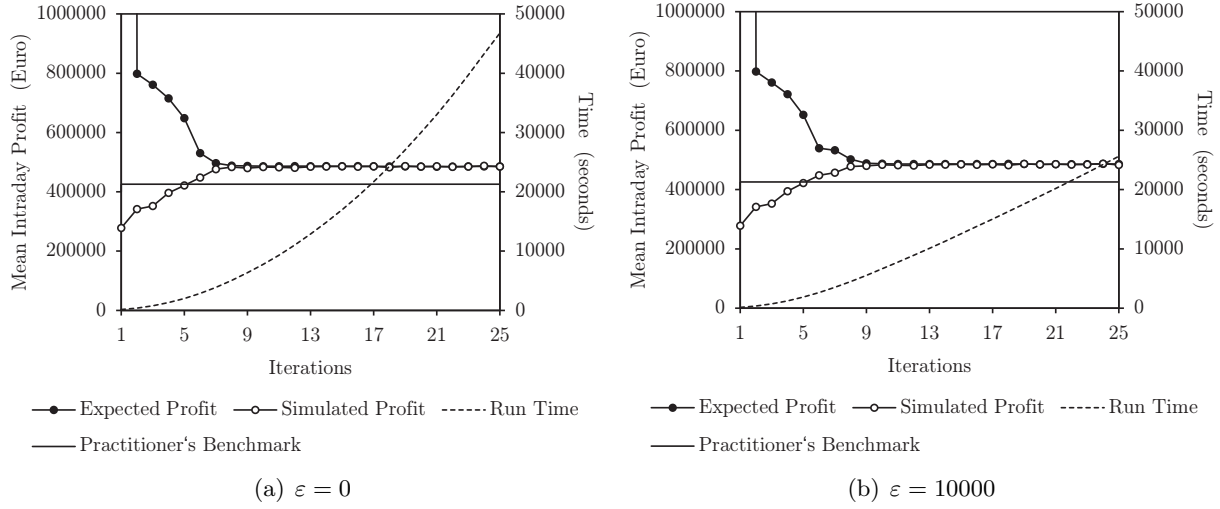
Figure 4.5: Convergence of ADDP for the system after the upgrade
