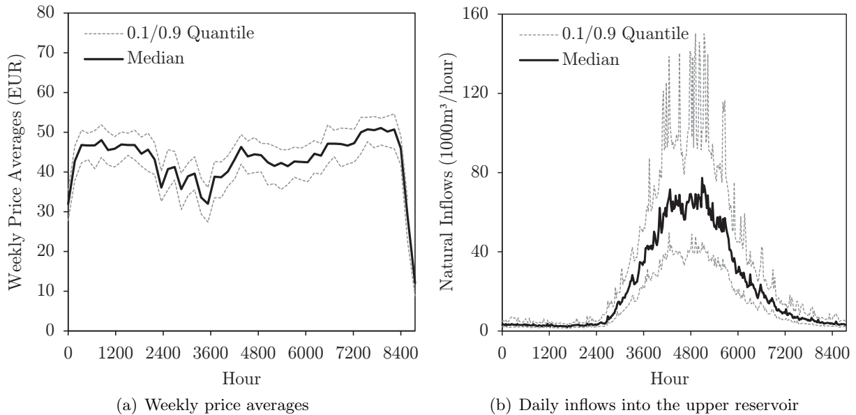
Figure 4.7: Stochastic processes
