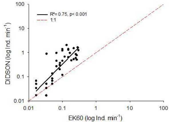
Figure 7 Relationship between DIDSON based abundance estimation and EK 60 based abundance estimation in (a) the overfall pool and (b) the groyne-head pool (both n=96 ). The 1:1 line highlights the variability of the abundance estimates in both systems.
