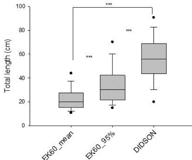
Figure 12 Comparison of fish total length estimates based on the three different sizing methods and two measuring devices. The stars indicate highly significant differences; the lines between the DIDSON box plot and the EK 60_mean box plot and the stars above the line show the significant between these two sizing methods.
