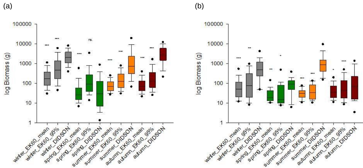
Figure 21 Comparison of the calculated biomass (EK 60_mean vs. EK 60_95% percentile vs. DIDSON) at the single recording dates (a) overall pool (b) groyne-head pool.
