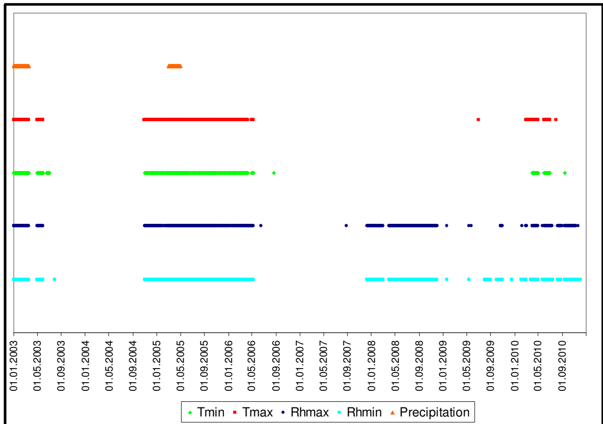
Appendix 1: Overview of missing climatic data. Signs mark missing values. Total number of missing days: Tmin 499, Tmax 516, RHmax 1004, RHmin 926, Precipitation 139
