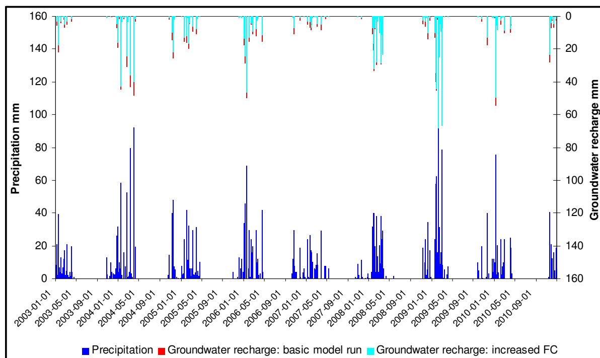
Figure 26: Daily sums of precipitation and calculated groundwater recharge rates in the basic model run compared to the model run with increased field capacity for the whole modelling period. When red colour is absent, both models show equal values. Precipitation during the rainy seasons (October to April) was 348 mm at the beginning of 2003, 613 mm in 2003/2004, 580 mm in 2004/2005, 557 mm in 2005/2006, 365 mm in 2006/2007, 581 mm in 2007/2008, 850 mm in 2008/2009, 449 mm in 2009/2010 and 204 mm at the end of 2010.
