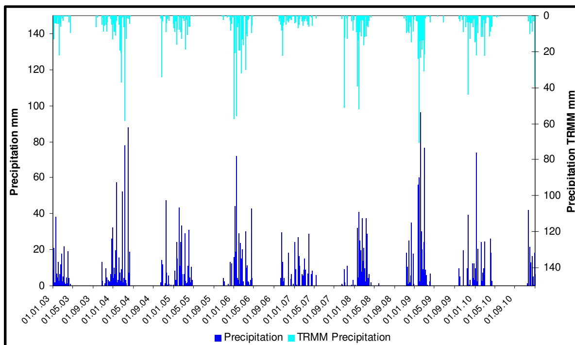
Appendix 4: Comparison of the completed NMS (2010) precipitation dataset with the TRMM (2010) precipitation time series
