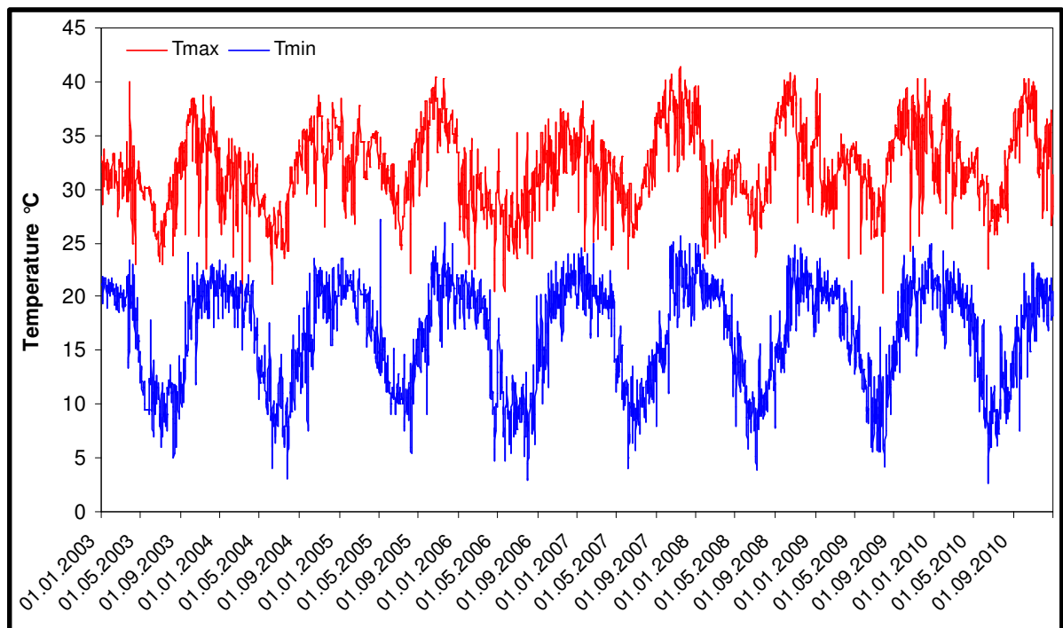
Appendix 2: Completed temperature time series 2003 – 2010.
