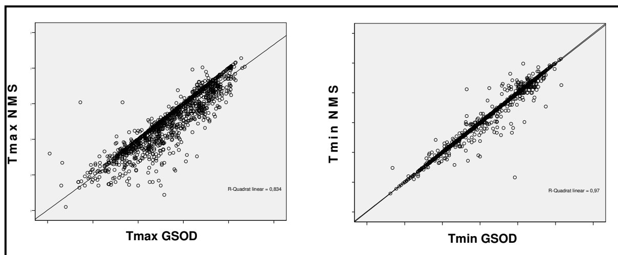
Figure 18: Scatter plots with regression line of maximum temperature (left) and minimum temperature (right) between the NMS- (Y- axis) and the GSOD (X – axis, station 680060) datasets. Homogeneity is assumed when the derivations of the regression line are in about the same range for all values.
