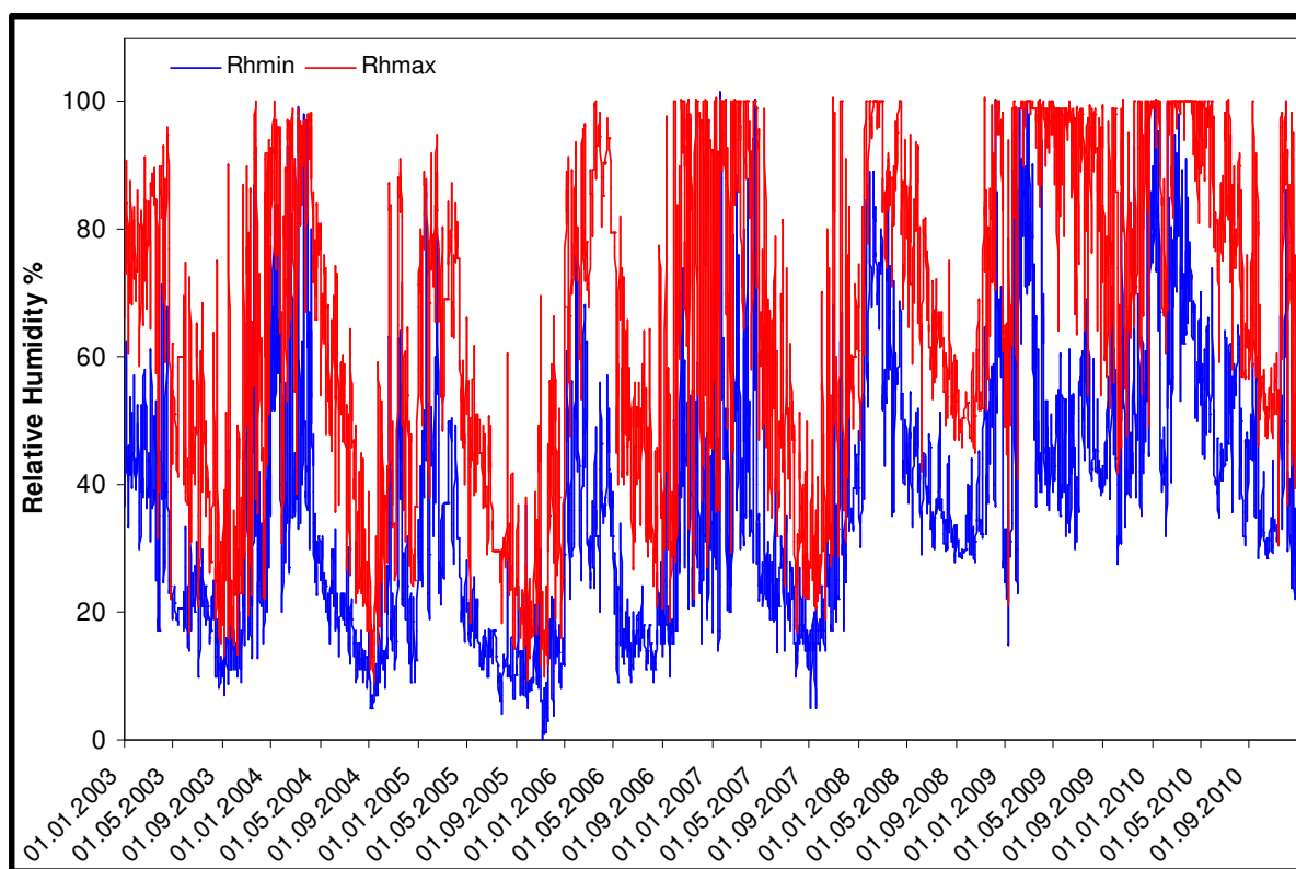
Appendix 3: Completed relative humidity time series 2003 – 2010.
