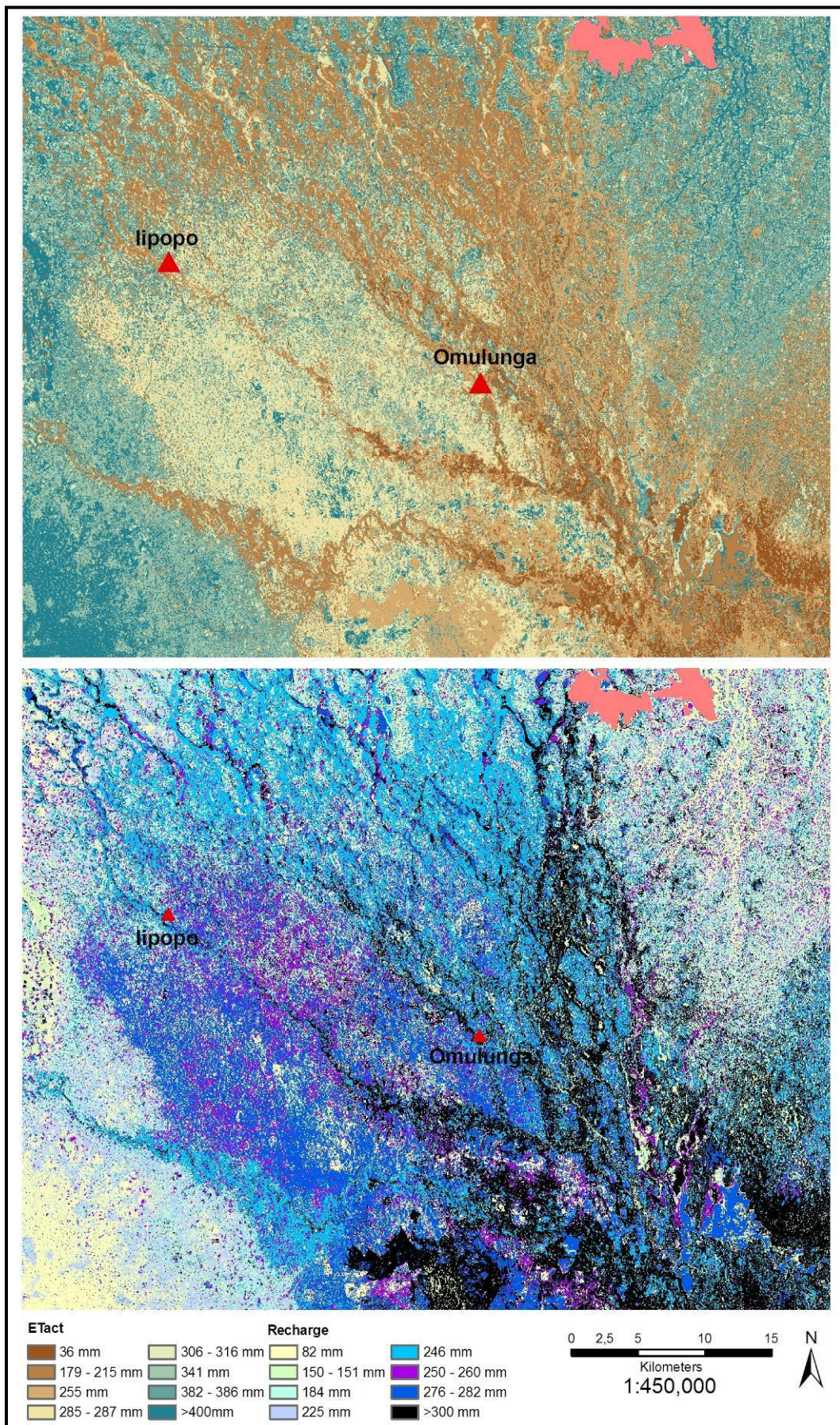
Figure 29: Modelled mean annual actual evapotranspiration (ETact, above) and potential groundwater recharge (below) in mm for the basic model run. ETact is without ETsec. Red area in the Northeast represents urban districts (not modelled).
