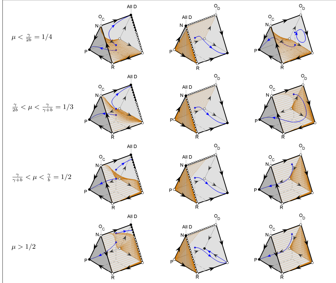
Figure 2.5: Replicator dynamics for b = 4 , c = 1 , \beta = \gamma = 2 and \mu = 15\%, 30\%, 45\% resp. \mu = 60\% . The arrows on the edges indicate the direction of the dynamics if all other strategies are absent. Black points represent Nash-equilibria, white points indicate unstable fixed points. The orange grid is the manifold that separates initial values with different asymptotic behaviour (i.e., a separatrix). The blue curves represent the typical dynamics for a given initial population.
