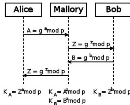
Abbildung 7.1: Bsp.:Man-in-the-Middle-Attack
