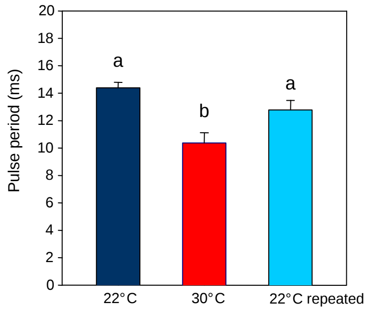
Fig. 8. Mean ( \pm S.E.) pulse period of long drumming sounds in catfishes kept at 22° C (■), 30° C (■) and 22° C repeated (■). N = 5 at 22° C and 22° C repeated; N = 8 at 30° C. Different letters indicate significant differences between temperatures ( p \leq 0.05 ).
