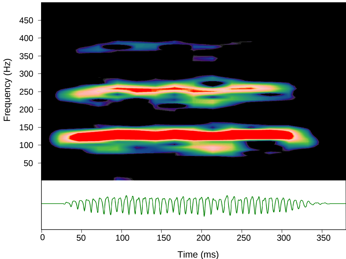
Fig. 7. Sonagram and oscillogram of a long drumming sound. The sonagram shows three harmonics with the main energy concentrated at the first harmonic (fundamental frequency). Sampling rate 44.1 kHz, Filter bandwidth 10 Hz, hanning filter, overlap 75 %.
