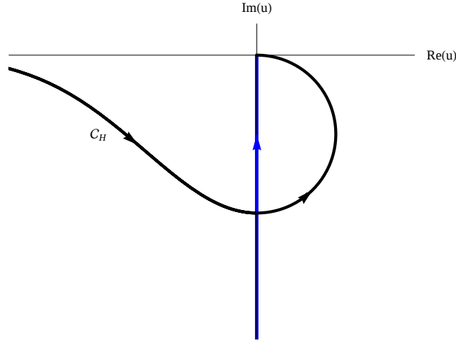
Figure 4.1.: Integration contour \mathcal{C}_H for H_1^{(2)} .
