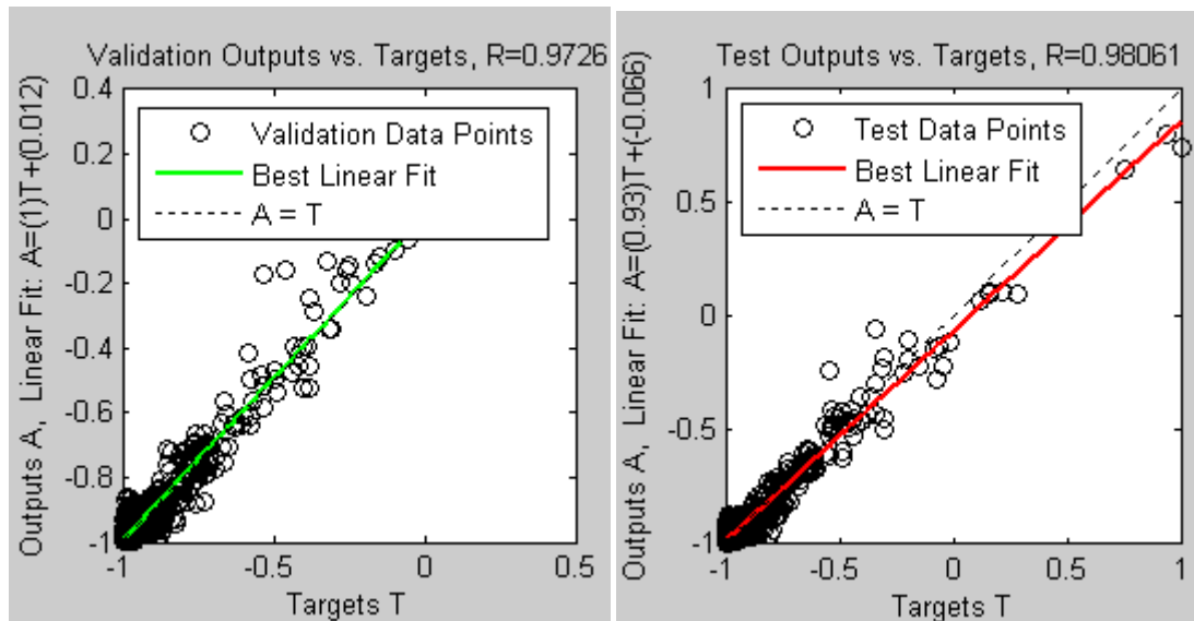
Figure 3 - 6: Validation Set Outputs versus Targets Figure 3 - 7: Test Set Outputs versus Targets
